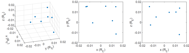
Figure 2. Configuration of the 7-S/C constellation.
