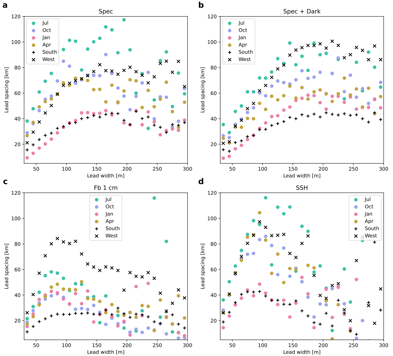
Figure A2. Sensitivity of the lead spacing combining the southern and western regions for the following lead definitions (a) ‘Specular’, (b) ‘Specular + Dark’, (c) ‘Freeboard height threshold at 1 cm’ and (d) ‘SSH flag’. The analysis is conducted as in Fig. 6.
