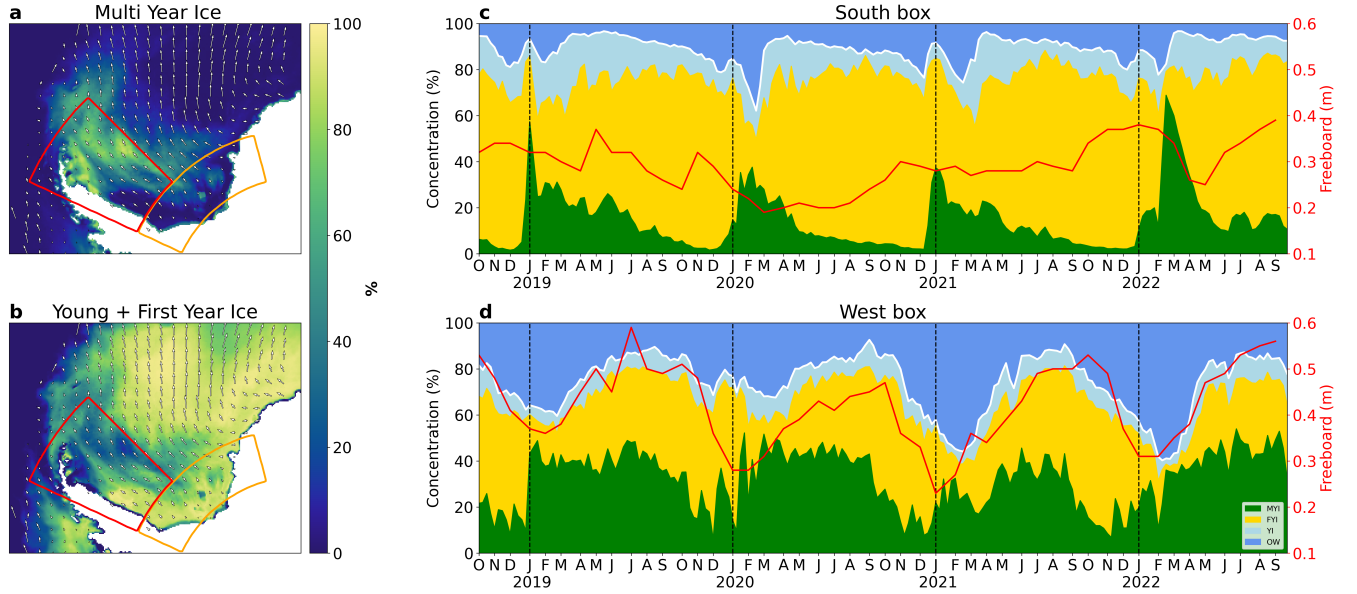
Figure 2. Seasonality of sea ice types in the perennial ice pack. (a-b) Sea ice concentration for (a) MYI and (b) YI+FYI in the Weddell Sea averaged between June-August 2019, with concurrent sea ice drift vectors (Melsheimer et al., 2023; Tschudi et al., 2019). The orange and red boxes in each panel delimit the southern and western regions, respectively. (c-d) Weekly-resolved time series of sea ice types averaged over the southern (c) and western (d) regions. The white line highlights the total sea ice concentration. The red line represents the area-weighted sea ice freeboard thickness at monthly resolution obtained from ICESat-2’s gridded product (ATL20).
