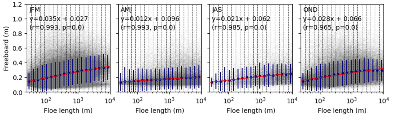
Figure A3. Mean floe freeboard versus floe chord length aggregated in 4 seasons during the years 2019 to 2022 for the (a) western and (b) southern regions of the pack. The floe length is divided into 20 ranges on a log scale. The red line indicates the linear best fit line and its corresponding statistics are detailed in each panel. The navy dots represents the median freeboard for each bin range, and the vertical navy bar indicates the standard deviation of freeboard.
