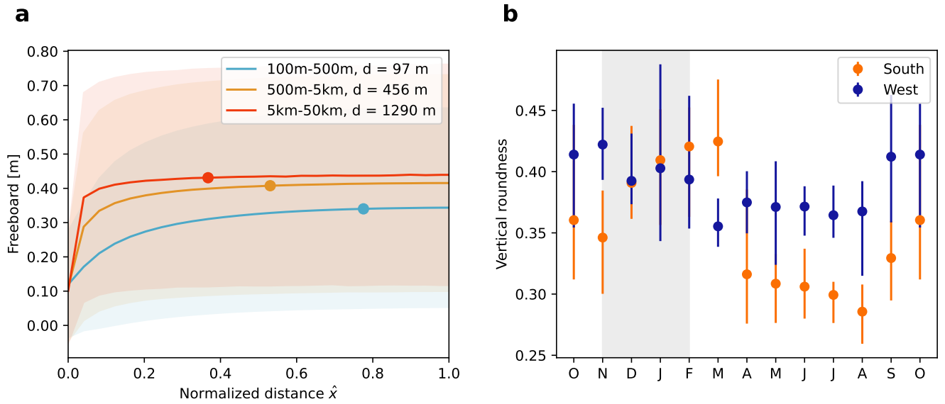
Figure 7. (a) Composited vertical floe profiles obtained by averaging the freeboard distribution along each floe and over a normalized horizontal distance \hat{x} . We consider all the floes detected within the analysis period and over both regions. The compositing is done separately for small (100 - 500 m, blue), medium (500 m - 5 km, orange) and large (5 - 50 km, red) floes, with each category comprising 2.8 \cdot 10^5 , 3.6 \cdot 10^5 and 1.5 \cdot 10^5 floes, respectively. The shading represents two standard deviations variability across individual floes. The colored dots represent the distance d over which the profiles flatten, defined as the point along \hat{x} where the profile slope drops below 0.05 in normalized units. (b) Monthly-mean vertical roundness of floes for the southern (orange) and western (blue) regions calculated from floe profiles including all sizes (100 m - 50 km). The error bars represent the minimum to maximum ranges of vertical roundness reported for the 4 years of analysis. The vertical grey shading highlights the approximate duration of the sea ice melt period.
