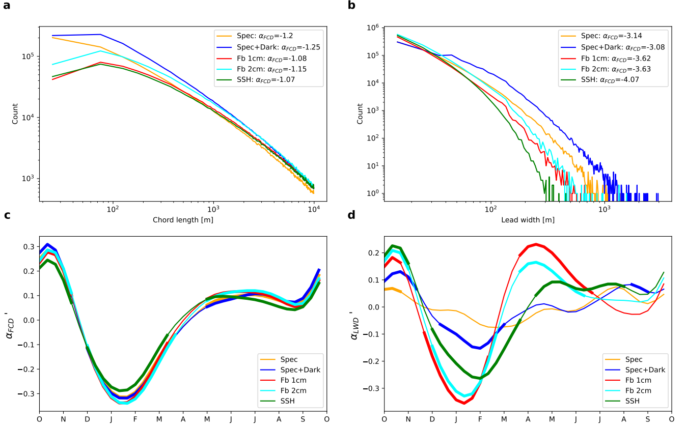
Figure A1. Sensitivity of the FCD and LWD to the lead detection method. (a) FCD for all floe chords, and (b) LWD for all leads. (c-d) Seasonal composites of (c) \alpha'_{FCD} and (d) \alpha'_{LWD} , calculated as in Fig. 4 (a) and Fig. 5 (b), respectively, combining the southern and western regions. The following lead detection methods are considered: ‘Specular’, ‘Specular + Dark’, ‘Freeboard height threshold at 1 cm’, ‘Freeboard height threshold at 2 cm’ and ‘SSH flag’. The thickner parts of each curve are significantly different from zero, based on a p-value of 0.05.
