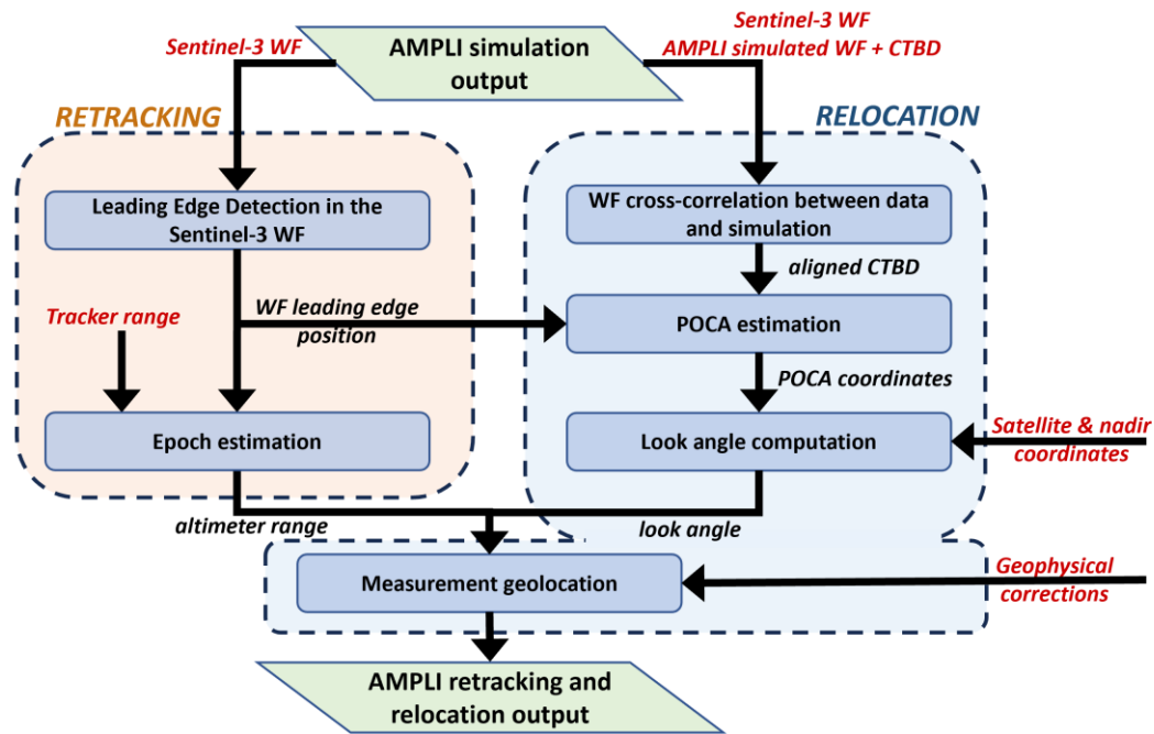
175 Figure 2: Flow chart describing the main operations included in the “retracking and relocation” module implemented in the AMPLI software.
