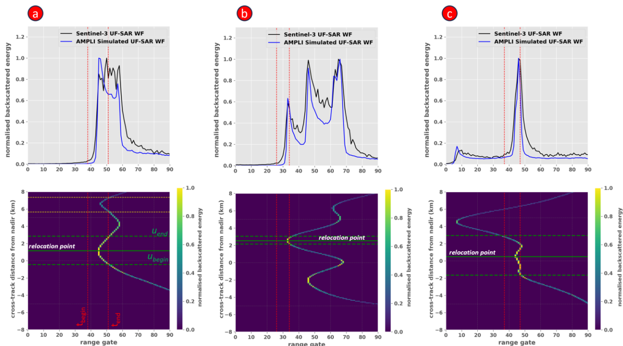
265 Figure 5: Illustration of the relocation method implemented in the AMPLI software, for three case studies (a, b, c). Sentinel-3A UF-SAR waveforms (black) and AMPLI simulated waveforms (blue) are displayed in the top panels. The corresponding AMPLI Cross Track Backscatter Distributions (CTBD) are displayed in the bottom panels. Red dotted lines indicate the start and stop indexes of the waveform leading edge, as identified by the retracker. Solid dotted lines indicate the centre of gravity of the cluster, where the measurement is relocated. In the cases of (a) and (b), yellow dotted lines indicate the location of an ambiguous cluster.
