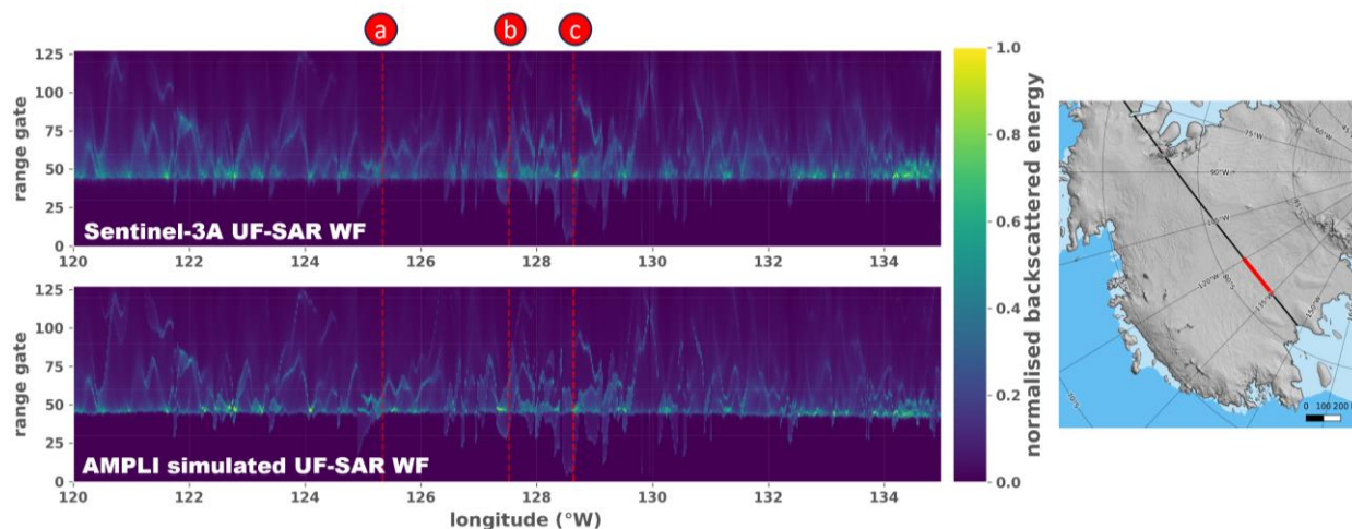
250 Figure 4: Illustration of the Sentinel-3A waveforms generated by the ESA ground segment processing (top), and simulated with the AMPLI software (bottom), along a track portion of about 250 km length, located in West Antarctica. The segment displayed is highlighted in red colour on the right map. The red dotted lines correspond to 3 single measurements used as case studies to illustrate the relocation processing in Fig. 5.
