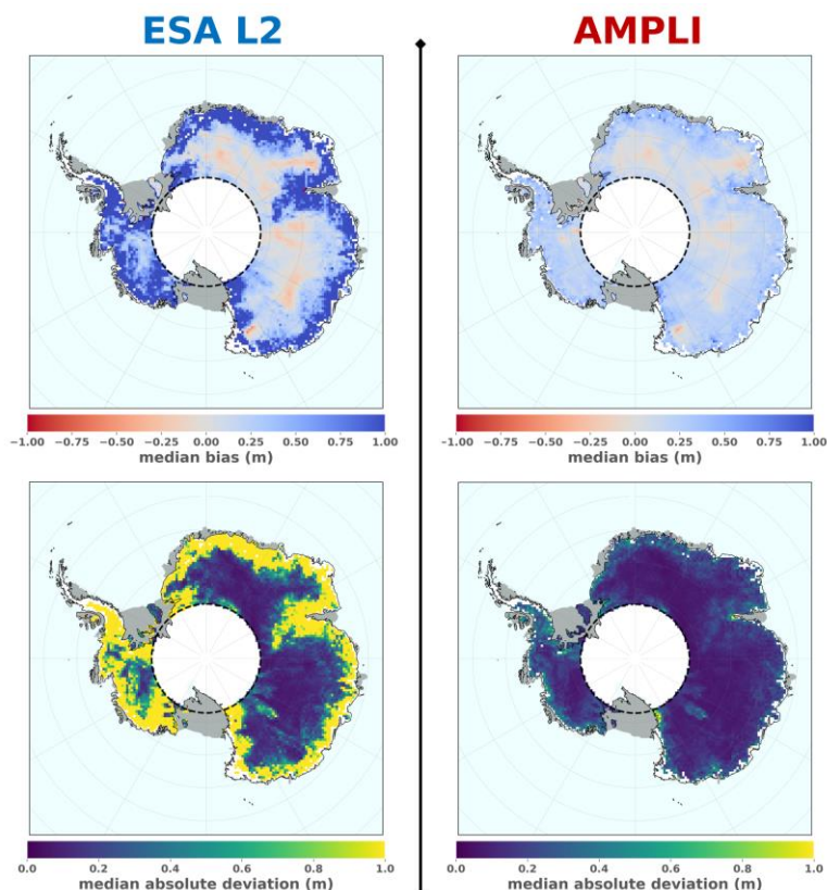
Figure 6: Gridded statistics of the elevation differences between Sentinel-3 and ICESat-2 ATL06 co-located elevations: median difference (top), median absolute deviation (bottom). Sentinel-3 elevations were read in the ESA L2 products (left) and derived from AMPLI (right). Elevations are computed as Sentinel-3 – ICESat-2. Grid resolution is 40 km.
