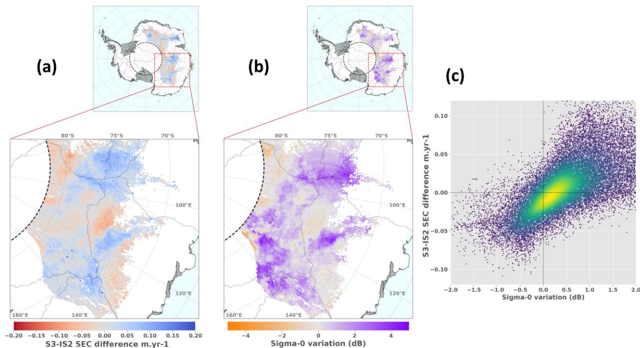
490 Figure 9: (a) Difference between Surface Elevation Change (SEC) maps from Sentinel-3 AMPLI and ICESat-2 ATL15, calculated over the 2019-2022 period, over the East Antarctic Ice Sheet interior (surface elevation above 2,500 metres, surface slope below 0.2° and ICESat-2 ATL15 SEC below 5 cm yr -1 ). (b) Sentinel-3 backscattered coefficient variation between 2019 and 2022 over the same area. (c) 500 Scatter plot between grid points of the Sigma-0 variation map displayed in (b) and SEC difference map displayed in (a).
