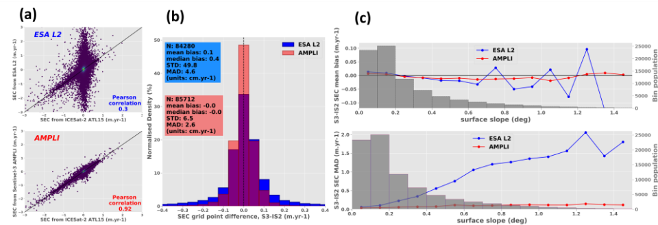
Figure 8: Statistical analysis of the difference between Sentinel-3 and ICESat-2 Surface Elevation Change (SEC) maps of the Antarctic ice sheet, 2019-2022 period. In the case of Sentinel-3, SEC is estimated with ESA L2 (blue) and AMPLI (red) data. In the case of ICESat-2, SEC is extracted from ATL15 product. SEC is mapped on a same 10 km x 10 km stereographic grid. (a) Scatter plots of the grid point differences. (b) Histograms of the grid point differences, computed as Sentinel-3 – ICESat-2. (c) Mean bias (top) and Median Absolute Deviation (bottom) of the grid point differences, represented as a function of the surface slope.
