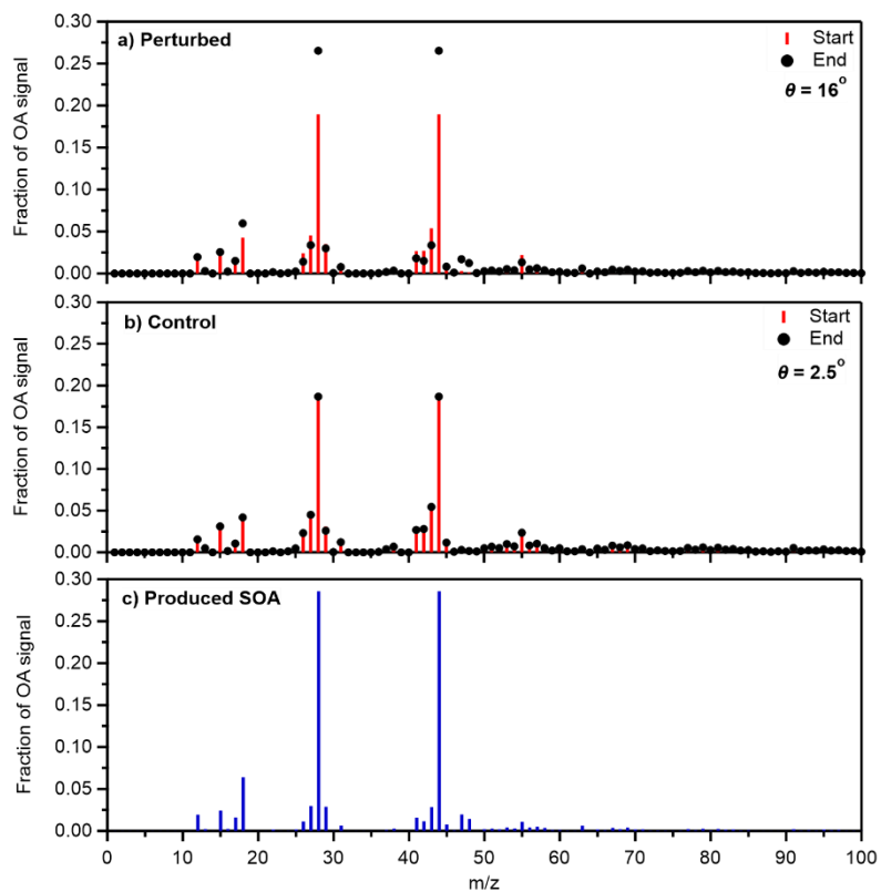
1005 Figure 3: Average fractional signal of the organic aerosol at the start and the end of Exp. 1 in Po Valley in a) the perturbed and b) the control chambers. The mass spectrum of the SOA formed in the perturbed chamber during the same experiment (c) is also depicted.
