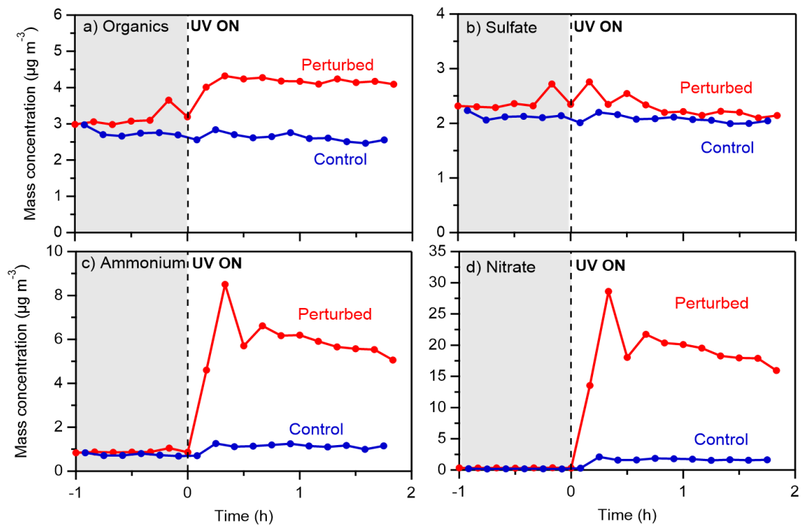
1020 Figure 7: Wall-loss and CE corrected mass concentrations of a) organics, b) sulfate, c) ammonium and d) nitrate in the perturbed and the control chambers during Exp. 1 in Pertouli.
