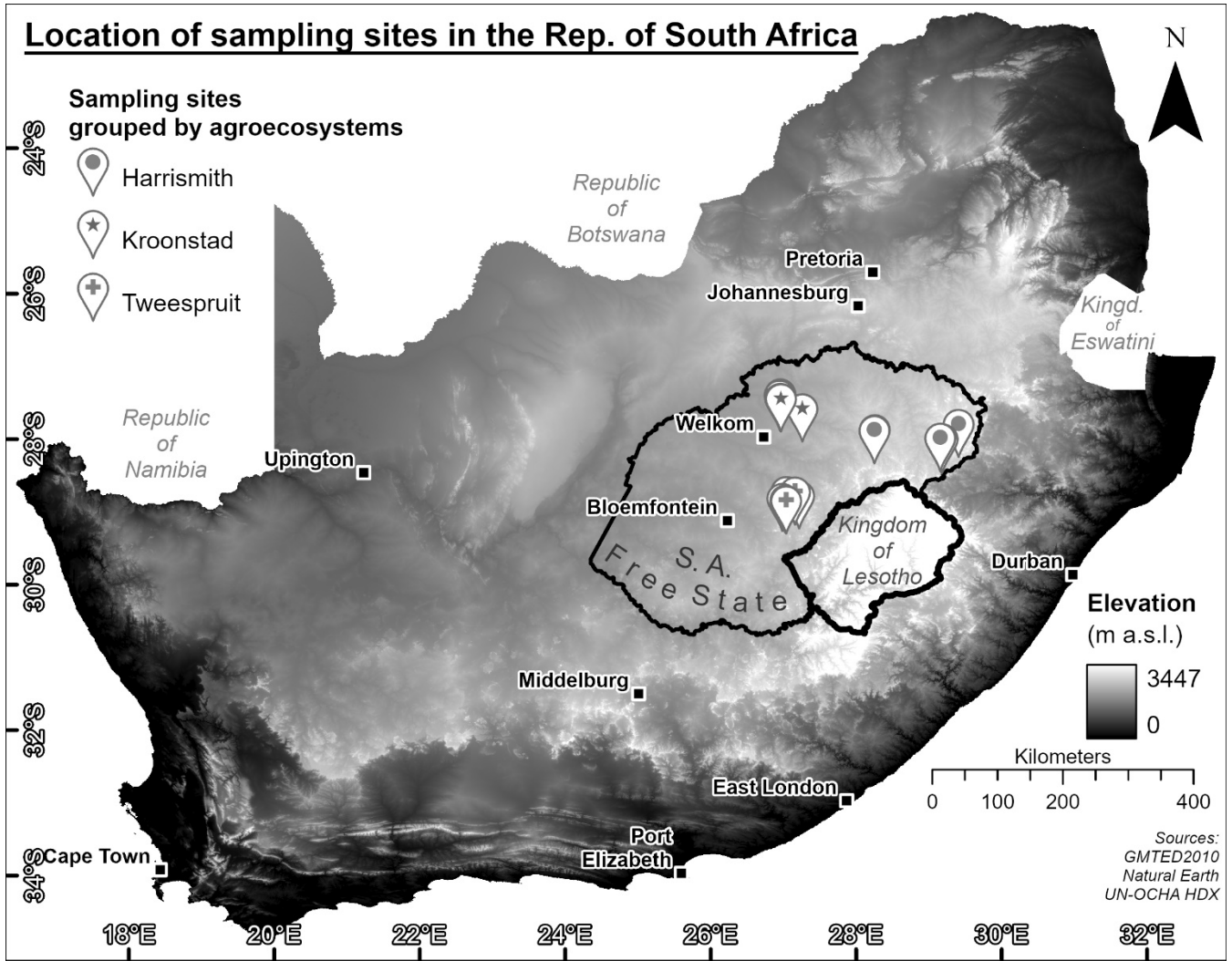
785 Figure 1: Topographic map of the Republic of South Africa and the state territory of the Kingdom of Lesotho. Sampling locations are highlighted by tear pins. Administratively, the investigated sites are located within the Free State Province of the Republic of South Africa. The province largely stretches the Highveld ecoregion, which resembles an elevated, open grassland plain landscape.
