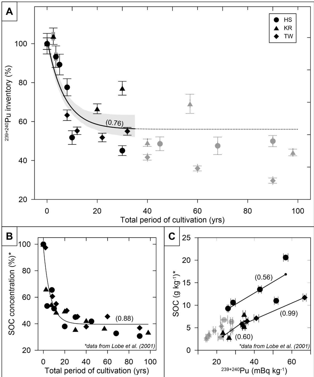
795 Figure 2: Changes in topsoil fallout inventories (A) and bulk soil organic carbon (SOC) content (B; Lobe et al., 2001) over time, and correlation of the SOC and ^{239+240}\text{Pu} concentrations (C). The inventories in cultivated soils are shown relative to those found in adjacent native grassland soils (i.e., 100% at t = 0 ). The mono-exponential regression (thin black line, enveloped by grey 68% confidence interval) in panel (A) indicates the approach towards a concentration equilibrium level after about 20-40 years of cropping. By that time, about 50-60% of the initial ^{239+240}\text{Pu} inventory has been lost. The extrapolated post-35 years cropping equilibrium level is indicated by the dashed line. The relationship between ^{239+240}\text{Pu} and SOC indicates that the decrease of SOC can be traced by measuring ^{239+240}\text{Pu} in bulk soil (C). Most plutonium samples depict replicate measurements; the corresponding activities are weighted means and the uncertainties either dominated by AMS counting statistics (weighted mean error) or external sources of uncertainty (standard error). For single measurements, the 1\sigma measurement uncertainty provided by the AMS facilities dominates the final uncertainty. All greyed out data points with dashed error bars denote those samples that were taken from plots with more than 32 years of cultivation history (for discussion see text). Filled circles denote samples from the Harrismith (HS) agroecosystem; filled triangle those from the Kroonstad (KR) agroecosystem and filled diamonds those from the Tweespruit (TW) agroecosystem. Numbers in brackets denote correlation coefficients ( R^2 ).
