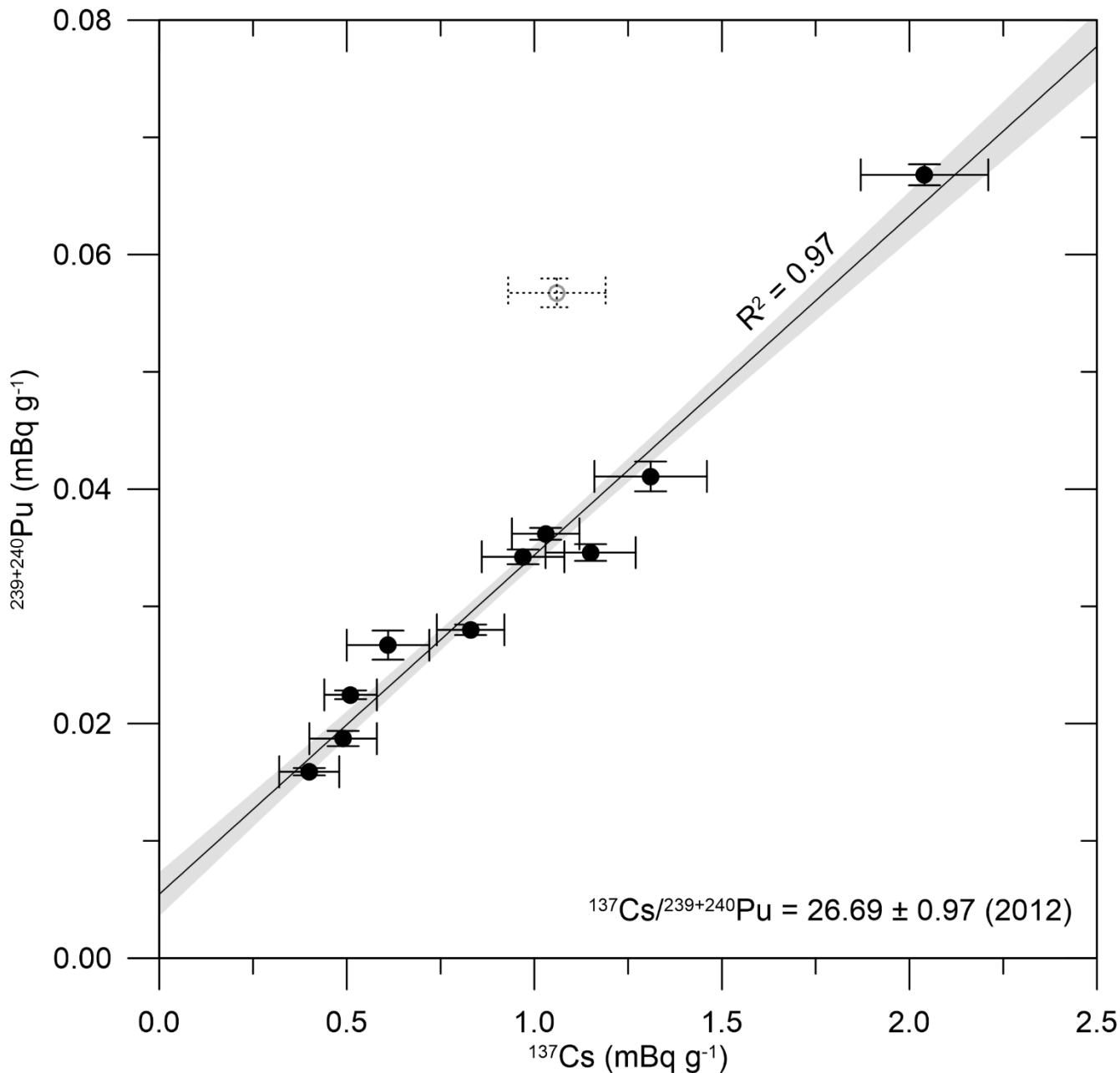
810 Figure 3: Correlation of ^{137}\text{Cs} and ^{239+240}\text{Pu} topsoil activities. ^{137}\text{Cs} data are shown with 1\sigma uncertainties (which equal the estimated measurement errors). ^{239+240}\text{Pu} activities were mostly measured in replicate, and the corresponding concentrations are weighted means and the uncertainties either dominated by AMS counting statistics (weighted mean error) or external sources of uncertainty (standard error). For single measurements, the 1\sigma measurement uncertainty provided by the AMS facilities dominates the final uncertainty. The majority of samples overlap with the linear regression (black line) and its 68% confidence interval (in grey). Sample HS0/0-20 has been excluded from the regression (greyed out; for discussion see text). The extrapolated regression intersects the ordinate at about 0.0050 \text{ mBq g}^{-1} ( 0.50 \text{ mBq kg}^{-1} ; unit conversion to \text{mBq g}^{-1} due to lower level precision achieved by \gamma spectrometry). ^{137}\text{Cs} data have been decay-corrected to February 2012 (the time of measurement).
