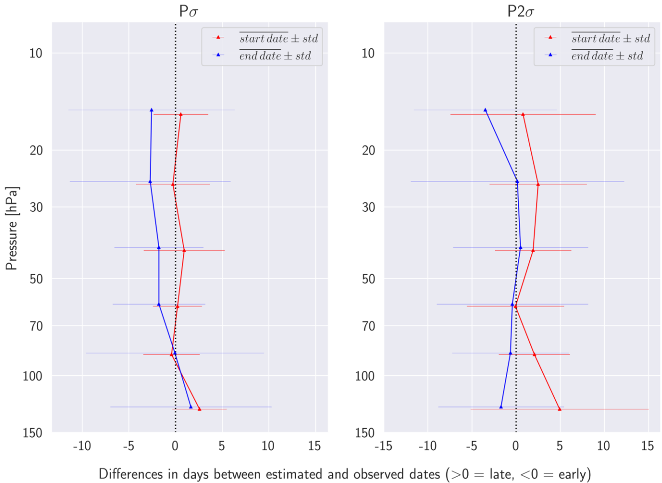
315 Figure 7: Vertical profiles of the average differences between the start (red) and end (blue) of P_\sigma (left) and P_{2\sigma} (right) periods according to CALIPSO observations and our model estimations over the 2007-2020 period. Our model is applied to MERRA2 temperatures provided by the CALIPSO PSC product. The horizontal bars represent the standard deviations of differences.
