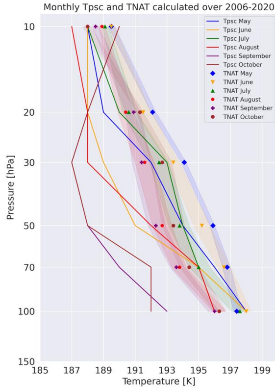
230 Figure 4: Vertical profiles of monthly T_{psc} (colored lines) and T_{NAT} (colored symbols). The colored envelopes represent the standard deviation of daily T_{NAT} .
