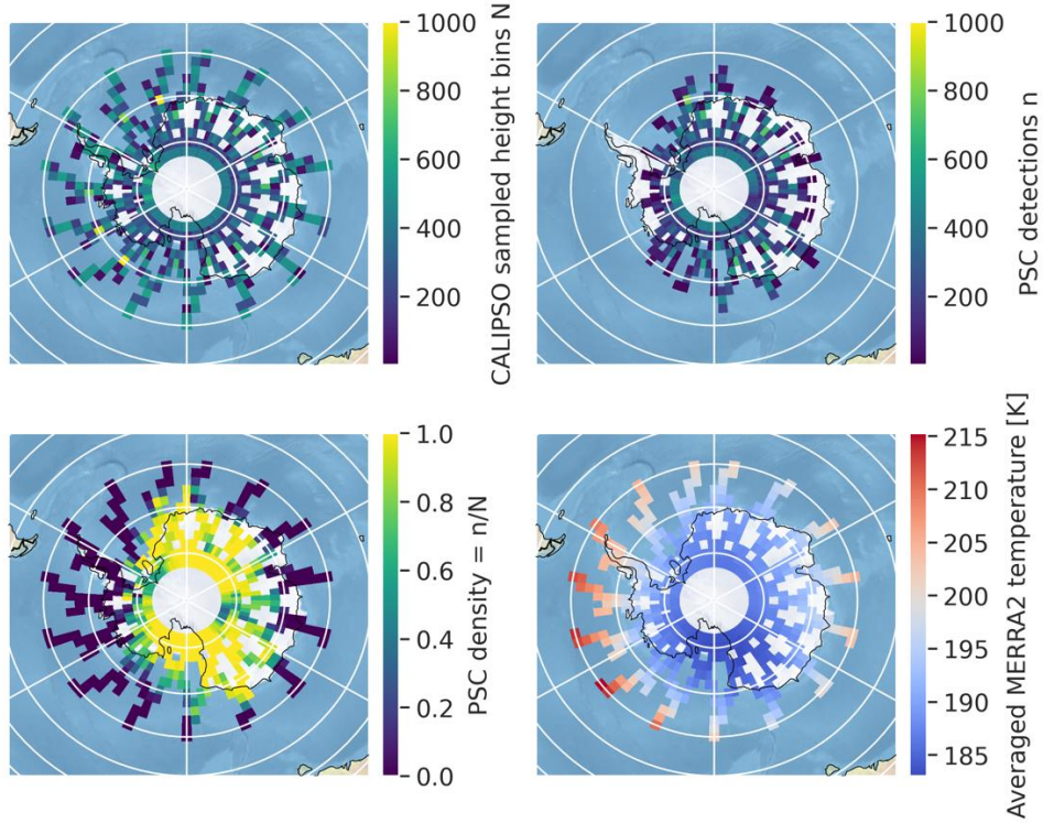
Figure 1: Output of daily gridding for July 1 st , 2009, between 50-70 hPa. (a) number of sampled points N . (b) number of PSC detections n . (c) PSC density F_{lat,lon}(P) , and (d) mean stratospheric temperature \langle T_{lat,lon} \rangle from MERRA2.
