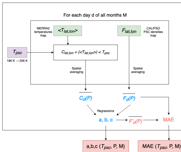
Figure 2: Flow chart describing the methodology. Green rectangles are input variables, in purple the temperature thresholds which vary and in red the output parameters.
