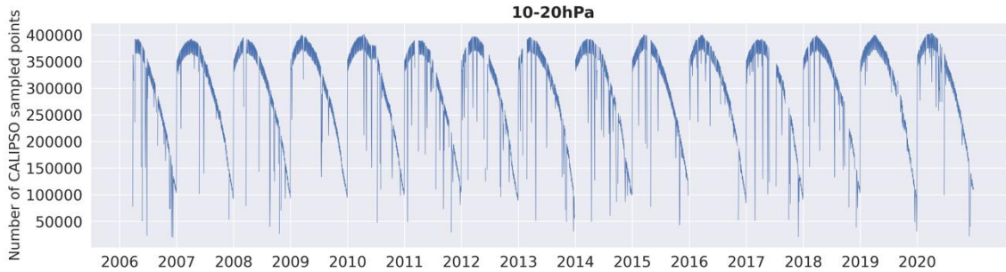
745 Figure A1: Total daily number of CALIPSO points from 2006 to 2020 at 10-20 hPa.
