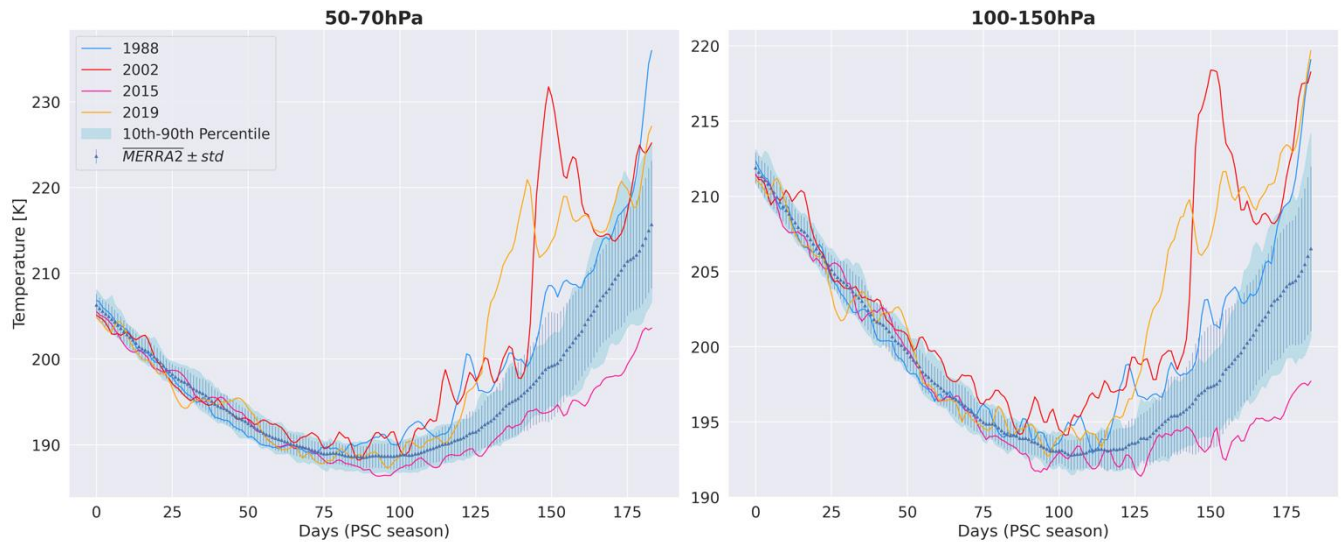
790 Figure E2: Daily MERRA2 gridded stratospheric temperature average between 60° S-90° S and over each PSC season from 1980 to 2021, at 50-70 hPa (a) and at 100-150 hPa (b). The time series goes from 1 st May (day 0) to 31 st October (day 184). The mean of MERRA2 (blue triangles) and its standard deviation (blue vertical lines).
