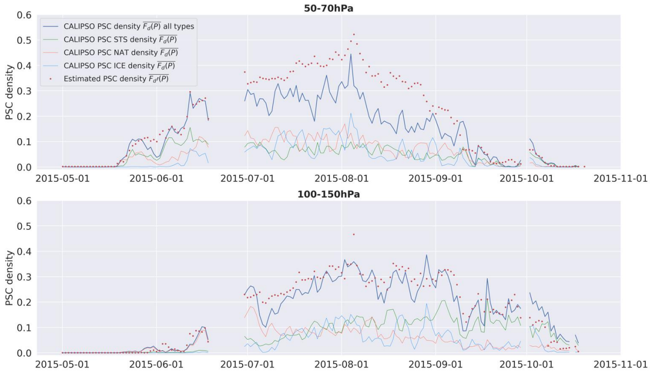
785 Figure E1: Time series of daily average PSC densities \overline{F_d(P)} observed by CALIPSO (blue curve) and PSC densities estimated by our model \overline{F_d'(P)} (red dots) at 50-70 hPa (a) and at 100-150 hPa (b) for the year 2015. Colored lines represent the different PSC types. Green is for STS, orange for NAT and blue for ICE.
