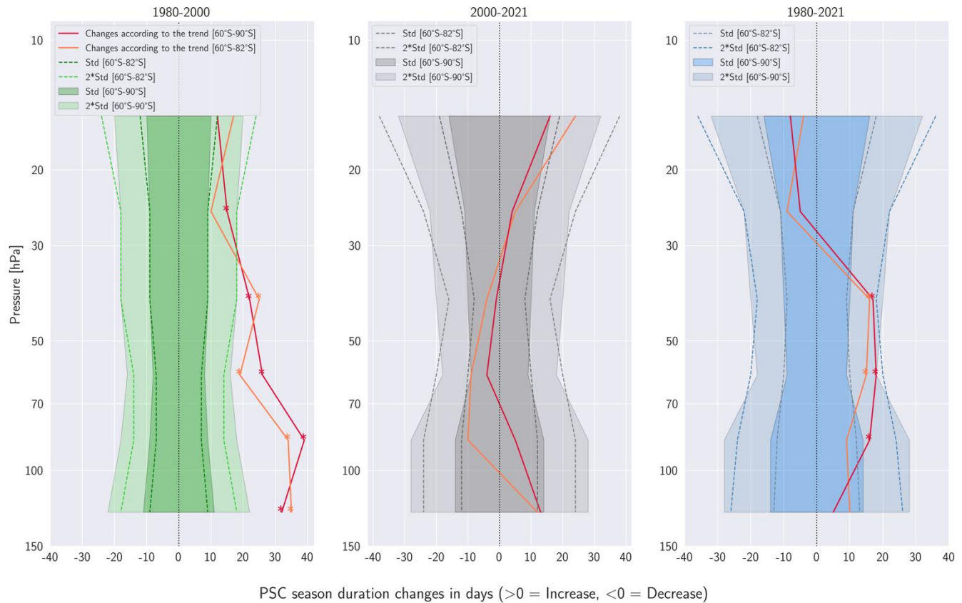
Figure 9: PSC season duration changes between 1980-2000 (a), 2000-2021 (b) and 1980-2021 (c) for each pressure level over all the polar region (60° S-90° S) and over the CALIPSO sampling region (60° S-82° S) derived from trend analyses using from linear regressions. The red (pink) lines represent the changes in the number of days of the PSC season duration in the 60° S-90° S (60° S-82° S) region. The envelopes represent the standard deviations associated with the time series of the PSC season duration. The stars indicate significant trends.
