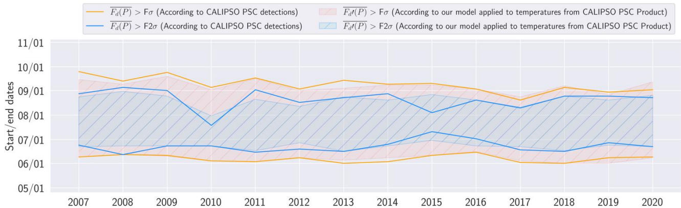
300 Figure 6: Start and end dates of P_\sigma (orange) and P_{2\sigma} (blue) for the 50-70 hPa pressure level for the time period 2007-2020. Full lines are based on PSC densities \overline{F_d(P)} retrieved from CALIPSO PSC detections, hatched surfaces are based on PSC densities \overline{F_d'(P)} derived from our model applied to MERRA2 temperatures provided by the CALIPSO PSC product.
