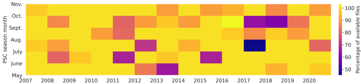
750 Figure A2: Percentage of available daily files for each month of the PSC season from 2007 to 2020.
