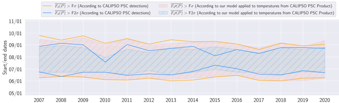
300 Figure 6: Start and end dates of P_\sigma (orange) and P_{2\sigma} (blue) for the 50-70 hPa pressure level over 2007-2020. Full lines are based on PSC densities \overline{F_d(P)} retrieved from CALIPSO PSC detections, hatched surfaces on PSC densities \overline{F_d'(P)} derived from our model applied to MERRA2 temperatures contained in the PSC product.
