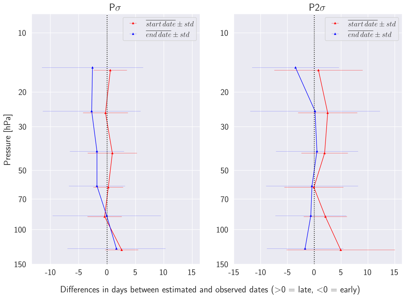
Figure 7: Vertical profiles of the average differences between the start (red) and end (blue) of P_\sigma (left) and P_{2\sigma} (right) periods according to CALIPSO observations and our model estimations over the 2007-2020 period. Our model is applied to MERRA2 temperatures contained in the PSC product. The horizontal bars represent the standard deviations of differences.
