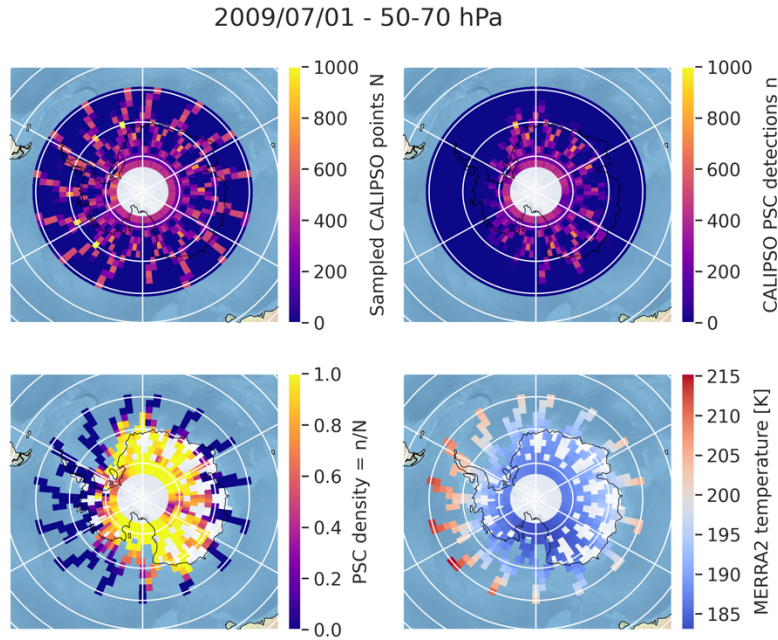
160 Figure 1: Output of daily gridding for July 1 st , 2009, between 50-70 hPa. (a) number of sampled points N . (b) number of PSC detections n . (c) PSC density F_{lat,lon}(P) , and (d) mean stratospheric temperature \langle T_{lat,lon} \rangle from MERRA2.
