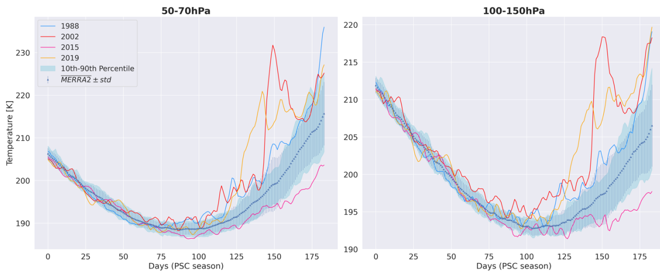
785 Figure E2: Daily MERRA2 gridded stratospheric temperature average between 60° S-90° S and over each PSC season from 1980 to 2021, at 50-70 hPa (a) and at 100-150 hPa (b). The time series goes from 1 st May (day 0) to 31 st October (day 184). The mean of MERRA2 (blue triangles) and its standard deviation (blue vertical lines).
