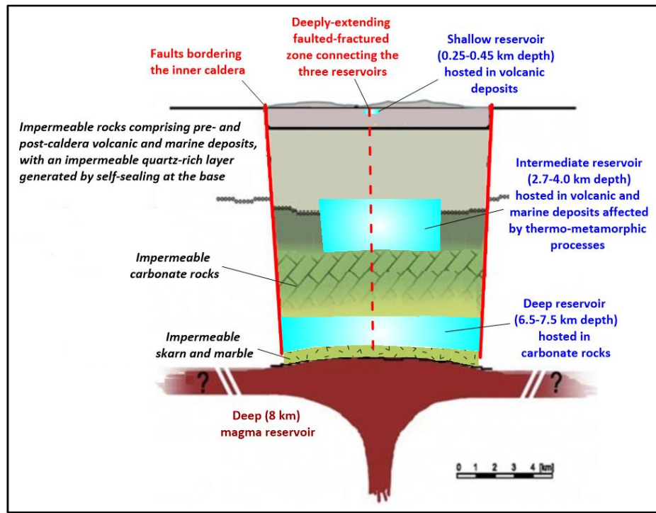
Figure 5. Conceptual model cross-section of the Solfatara hydrothermal-magmatic system at Campi Flegrei caldera (modified from Moretti et al., 2020; Elsevier license number 5234800567871 on Jan 23, 2022), showing the shallow, intermediate, and deep reservoirs.
