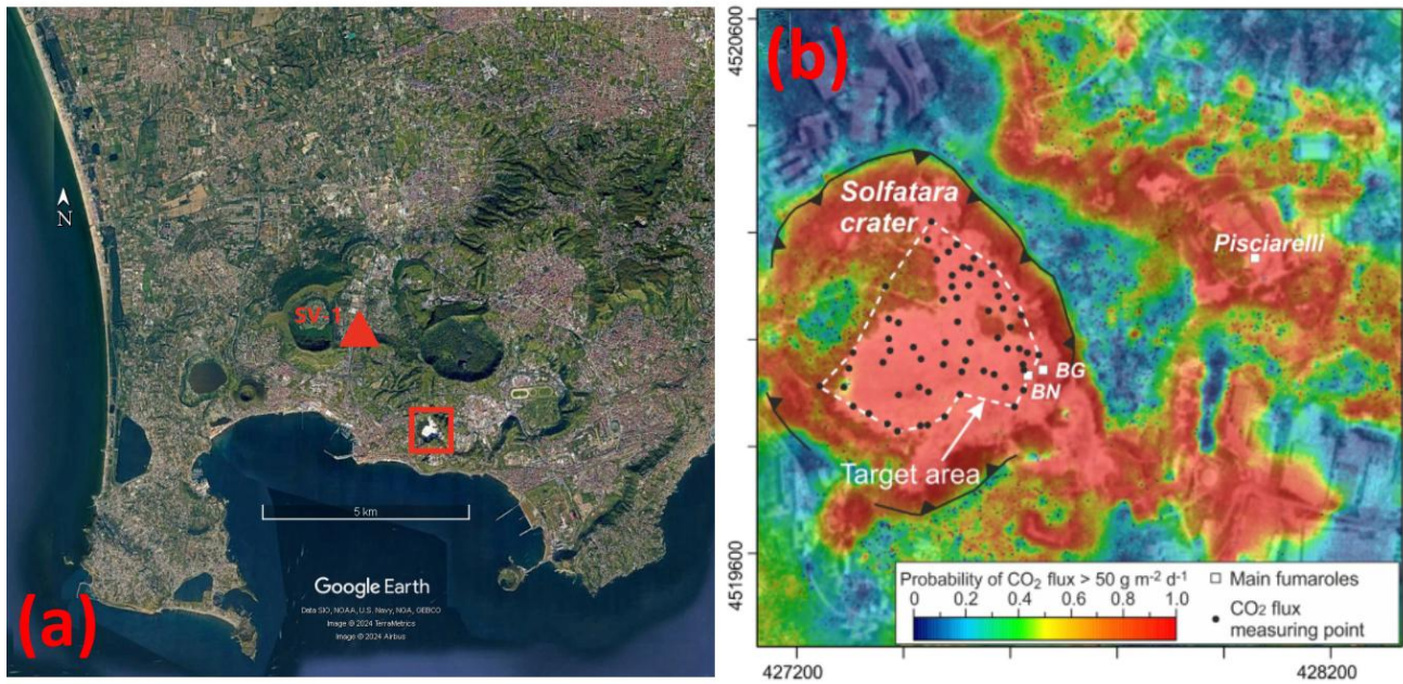
45 Figure 1: (a) © Google-Earth image of Campi Flegrei, showing the location of the deep geothermal well San Vito 1 (SV-1). The red square indicates Fig. 1b. (b) Map of the Solfatara-Pisciarelli diffuse degassing structure elaborated from the 1998-2016 dataset of CO 2 fluxes also showing the location of the Bocca Grande (BG), Bocca Nuova (BN), and Pisciarelli (Pi) fumarolic vents (from Chiodini et al., 2021; Elsevier license number 5601960223358 on Aug 04, 2023). Kilometric coordinates are reported on the two axes.
