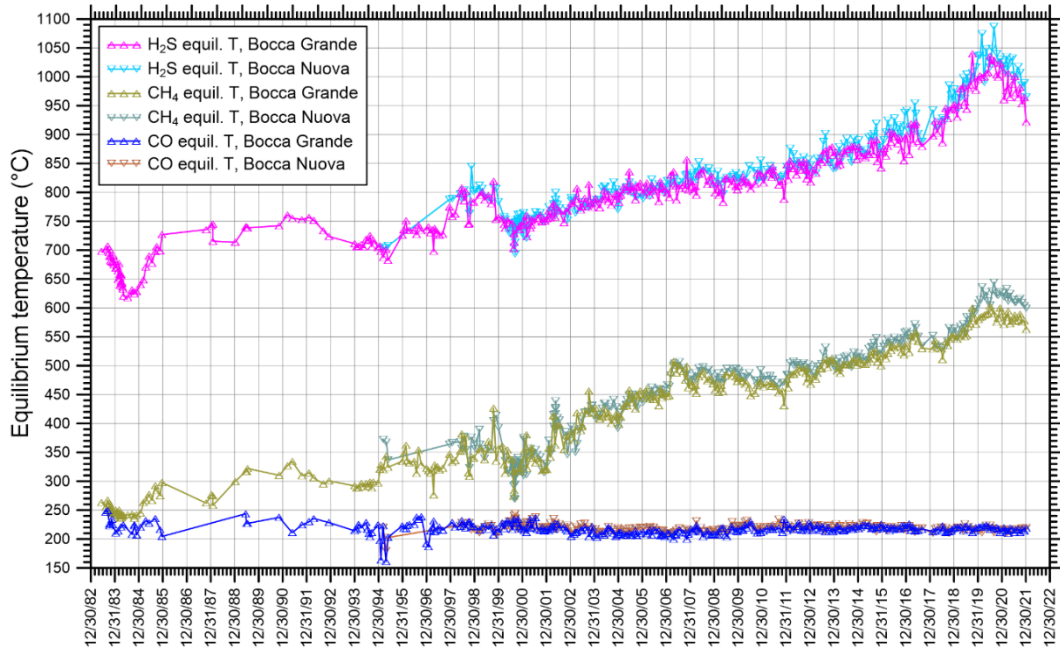
205 Figure 2: Chronogram of CO-, CH 4 - and H 2 S equilibrium temperatures for Bocca Grande, from June 1983 to January 2022, and from Bocca Nuova, from March 1995 to January 2022, calculated from the data of Cioni and coworkers and Chiodini and coworkers (Buono et al., 2023 and references therein).
