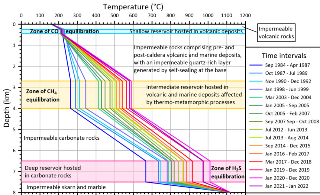
Figure 56. Time changes in September 1984-January 2022 of the temperature vs. depth profile along a hypothetical borehole drilled in the Solfatara crater. Also shown are the main lithological characteristics of the three reservoirs, where CO 2 , CH 4 , and H 2 S equilibrate, and of the impermeable zones interposed between the three reservoirs, positioned above the shallow reservoir, and situated below the deep reservoir (see text for details).
