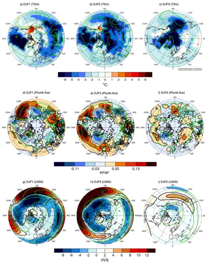
Figure 8. a) Response of 2-meter air temperature ( ^{\circ}\text{C} ) in cpl (color), and sea-level pressure (green contours), for winter 1. b) Same as a) but for winter 2. c) Same as a) but for winter 3. d) Response of 850 hPa vertical component of the Plumb flux ( \text{m}^2/\text{s}^2 ) in cpl , and the climatology as green contours from -8 to 12 by 2, for winter 1. e) Same as d) but for winter 2. f) Same as d) but for winter 3. g) Response of 200 hPa zonal wind ( \text{m/s} ) in cpl , and the climatology as green contours from -0.15 to 0.15 by 0.04, for winter 1. h) Same as g) but for winter 2. i) Same as g) but for winter 3. Contours and colored areas indicate significance at the 95% confidence interval according to a Student's t-test.
