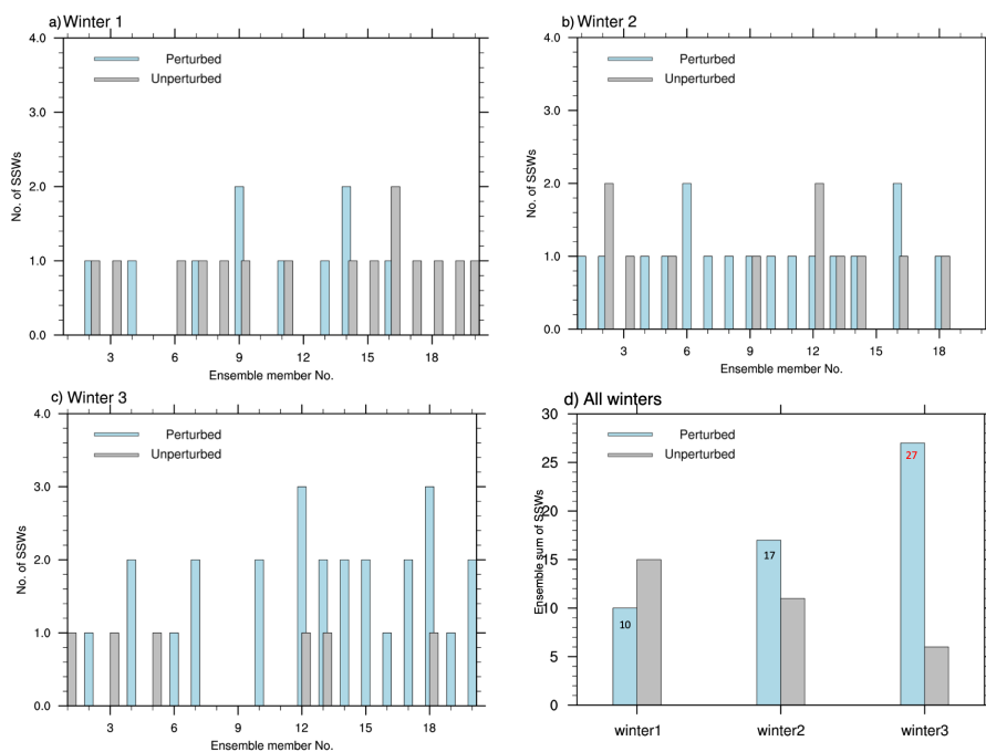
Figure 6: a-c) The number of SSWs during winters 1-3 for each ensemble member in the cpl experiment and d) The sum of all SSWs in each experiment for all 20 ensemble members of winters 1-3 both for cpl (light-blue bars) and control (gray bars). The color red indicates 95% significance according to a two-sided student's t test.
