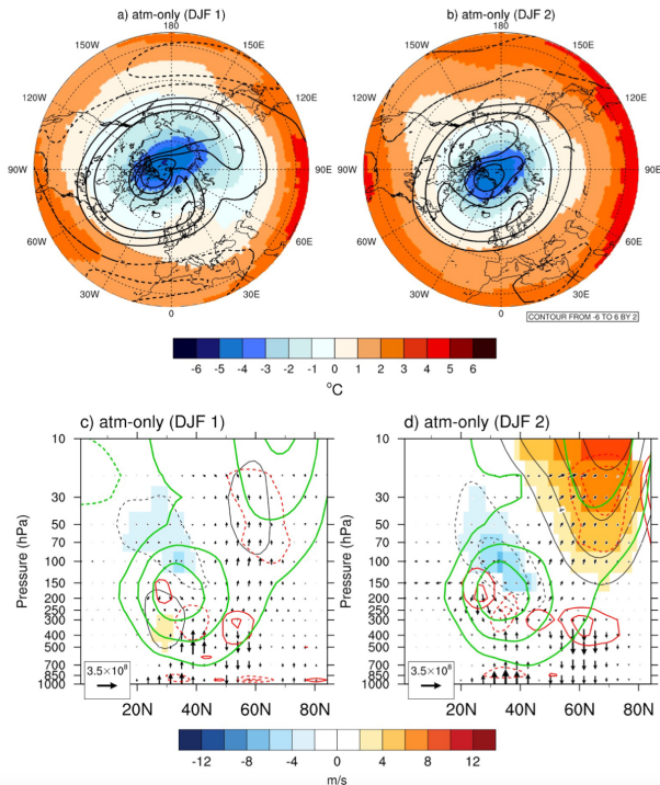
Figure 5: The same as Fig. 4 but for the atm-only experiment. a-b) Zonal wind (contours) and temperature (shading) response at 50 hPa for winter 1 and winter 2, respectively. c-d) EP flux (arrows) and divergence (red contours) response along with zonal-mean zonal wind (black contours) and climatology (green contours, 2m) in winters 1-2, respectively. Contours and colored area indicate 95% significance according to a student's t-test.
