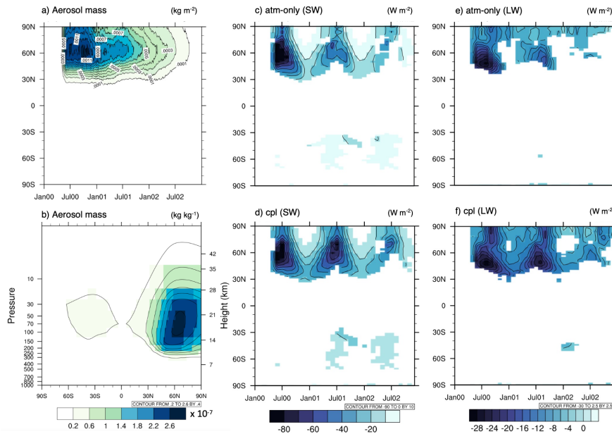
Figure 2: Left panels: a) Average aerosol column mass time evolution in kg/m² and b) pressure vs. latitude slice of the aerosol mass in kg/kg (3-year average). Aerosol mass is the same in cpl and atm-only. c) and d) show the time evolution of the net SW flux (downward) anomaly at the top of the atmosphere, and e) and f) the same but for net LW flux anomaly, resulting from the volcanic
