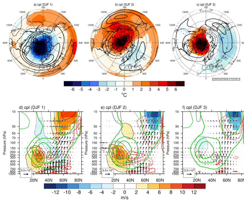
Figure 4: Winter stratospheric response in the cpl experiment. a-c) U_{50} (contours) and T_{50} (shading: red = warming, blue = cooling) response for winters 1-3, respectively. d-f) EP flux (arrows) and divergence (red contours) response, along with zonal-mean zonal wind response (black contours and shading: red = strengthening, blue = weakening) and climatology (green contours) in winters 1-3, respectively. Contours and color-shaded areas indicate 95% significance according to a student's t-test. Only vectors that are significant at the 95% confidence interval are shown.
