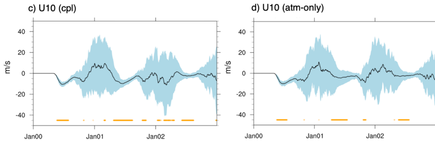
Figure 3. a,b ) Latitude versus time response of T50 anomalies in a) cpl and b) atm-only . Contours are significant in 95% confidence intervals according to a student's t-test. c,d ) Stratospheric polar vortex response shown as the zonal mean U10 anomalies between 70 and 80° N for c) cpl and d) atm-only . Black lines show the ensemble mean anomalies and blue shadings show the ensemble \pm 2 standard deviation anomaly range. Orange markers indicate when the difference between perturbed and unperturbed experiments becomes significant ( p < 0.05 ) according to a Kolmogorov-Smirnov test.
