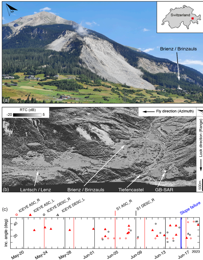
Figure 1: (a) Picture of the Brienz slope acquired from the GB-SAR station (see location in panel 1b) after the failure occurred on Jun-15, 2023. (b) Reference SAR (May-22, 2023) backscattering image in dB, after radiometric terrain correction. Some points of interest are indicated for spatial orientation. (c) Sentinel-1 and ICEYE imagery acquired over Brienz with indication of orbit direction (ascending or descending) and sensor look direction (left or right).
