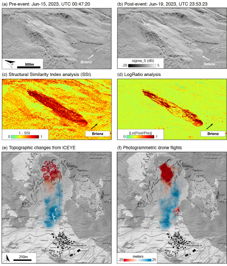
Figure 3: Comparison between (a) pre- and (b) post- event ICEYE images acquired over Brienz. (c) and (d) show the results of analytical change detection attempts with SSI and log-ratio methods, respectively. Comparison between (e) ICEYE interferometry and (f) DSM-of-Difference (DoD) generated from photogrammetric drone flights. Note that the negative height difference in (f) in the lower part above the village are trees cut down by the landslides.
