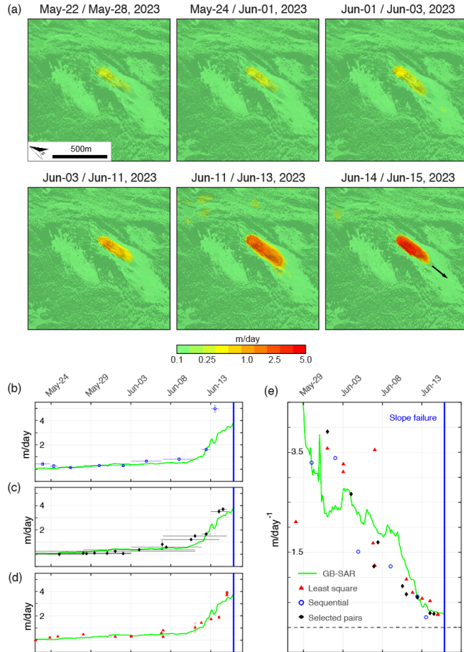
220 Figure 2: (a) Selected results showing the 2D surface velocities over Brienz measured with pixel-offset (PO) applied to the ICEYE data. Note that the colour scale is logarithmic to show the extreme differences in velocities occurred within few days a factor six larger compared to the one showed in (a). (b-d) Time series of maximum surface velocities measured with PO vs. velocities recorded with GB-SAR. Horizontal bars in b and c show the time span of the images paired. Error bars, in most cases smaller than the symbol size, are related to the median PO measured in an area considered stable (e) Inverse velocity plot to show failure forecasting potential of ICEYE PO results vs. GB-SAR. 225
