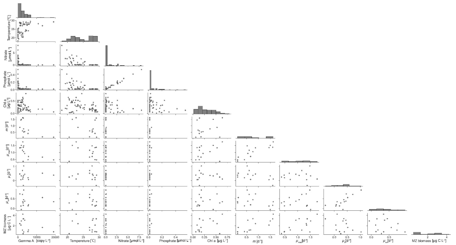
Figure S6. The paired scattered plots of Gamma A, each water property, and the parameters derived from the dilution experiments for Gamma A.
