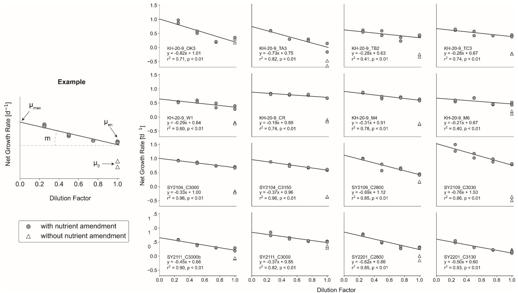
Figure S2. The example (left) and results of linear regression in dilution experiments at each station with statistical values for the least-square regression. ( \mu_{max} : maximum growth rate. m : mortality rate by microzooplankton grazing. \mu_0 : net growth rate measured in the nonenriched and nondiluted bottles. \mu_{en} : net growth rate measured in the enriched and nondiluted bottles)
