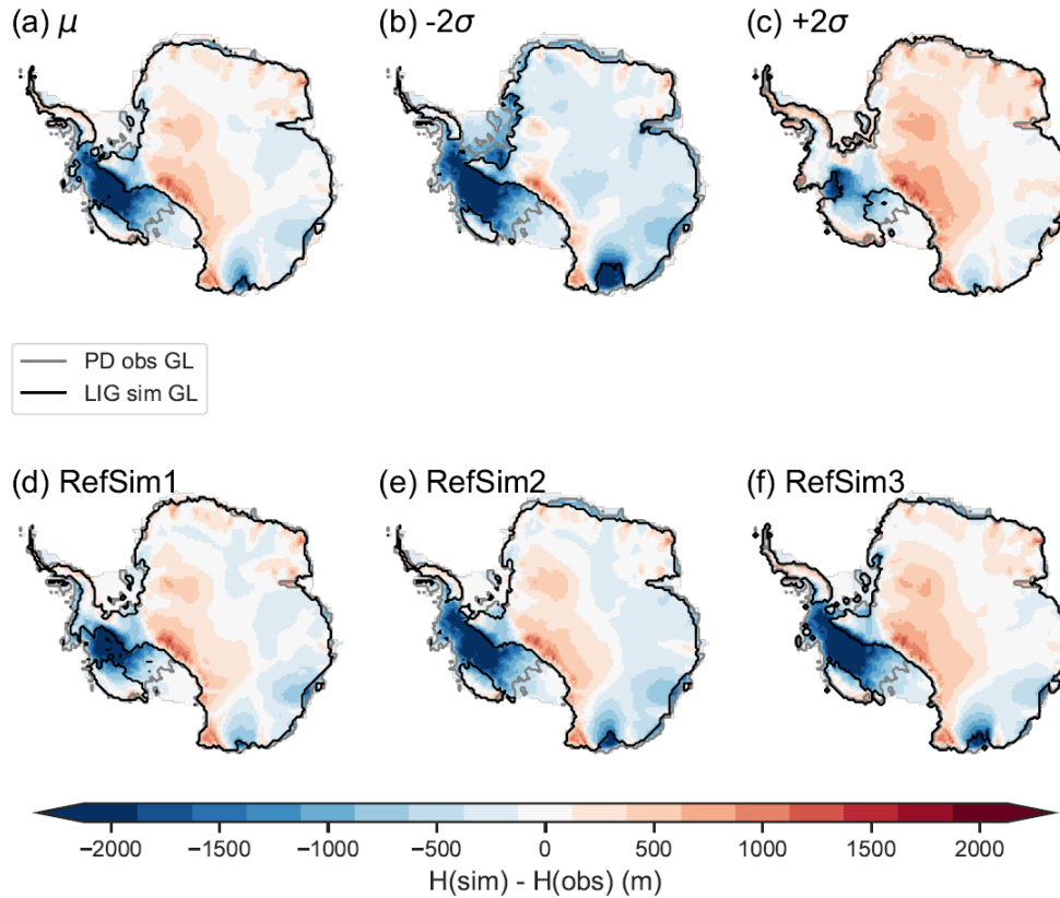
Figure 11: The not-ruled-out-yet (NROY) AN3sig sub-ensemble a) mean and b-c) 2\sigma range are shown during the LIG. Three glaciology self-consistent simulations chosen from a NROY high variance subset (HVSS) are showcased: d) RefSim1; e) RefSim2; f) RefSim3. The 2\sigma ranges are the nominal 95% ensemble intervals based on the equivalent Gaussian quantiles.
