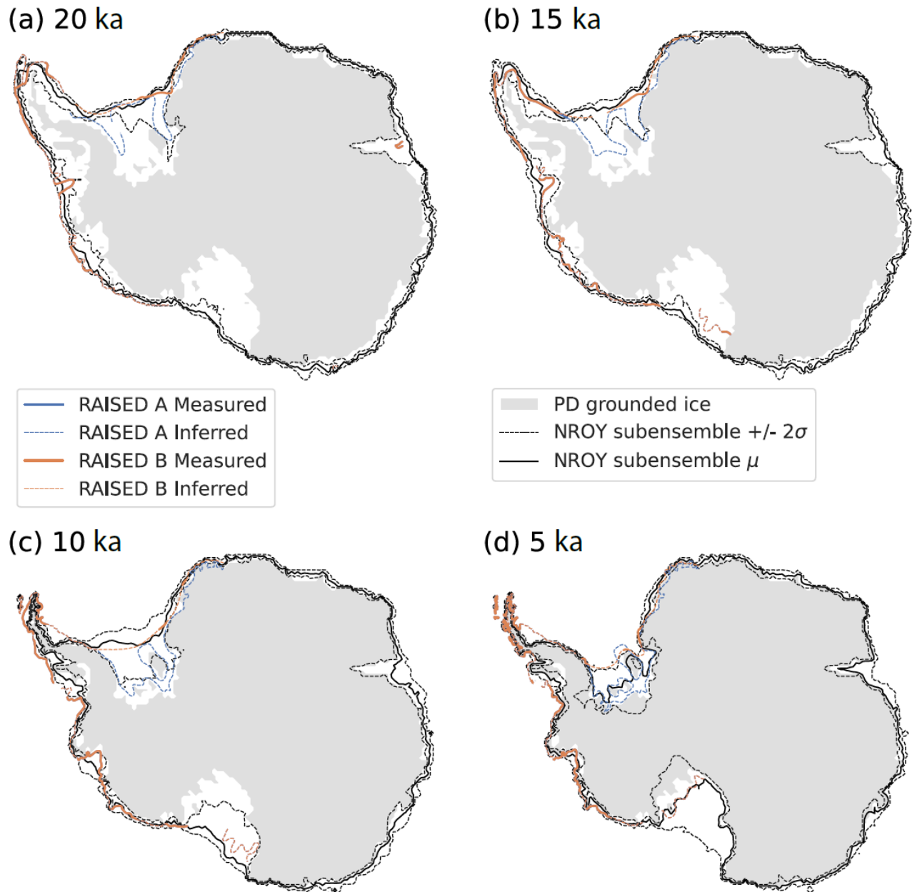
600 Figure 5: The mean and 2\sigma range grounded ice extent for the not-ruled-out-yet (NROY) AN3sig sub-ensemble is shown by the black and dashed black line, respectively. It is compared against the RAISED consortium scenario A and B measured and inferred contours at a) 20 ka, b) 15 ka, c) 10 ka, and d) 5 ka. The 2\sigma ranges are the nominal 95% ensemble intervals based on the equivalent Gaussian quantiles.
