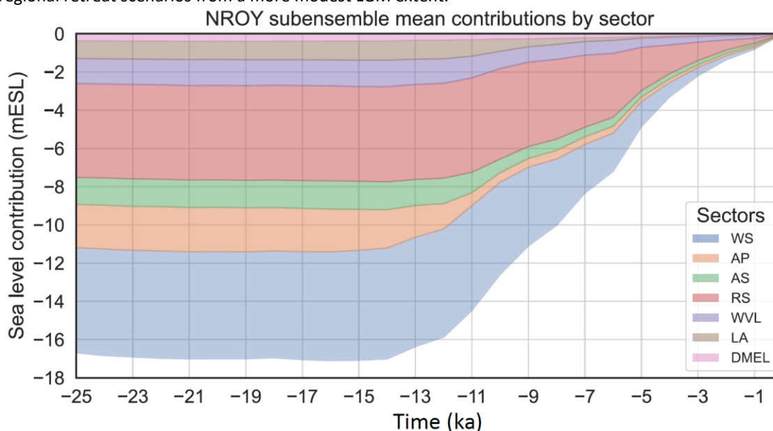
910 Figure 13: AIS grounded ice volume equivalent sea-level contributions since the LGM for the Weddell Sea (WS), Antarctic Peninsula (AP), Amundsen Sea (AS), Ross Sea (RS), Wilkes – Victoria Land (WV), Lambert – Amery (LA), Dronning Maud-Enderby Land (DMEL) as defined in Fig. 3.1 during the deglaciation based on the NROY AN3sig subensemble mean.
