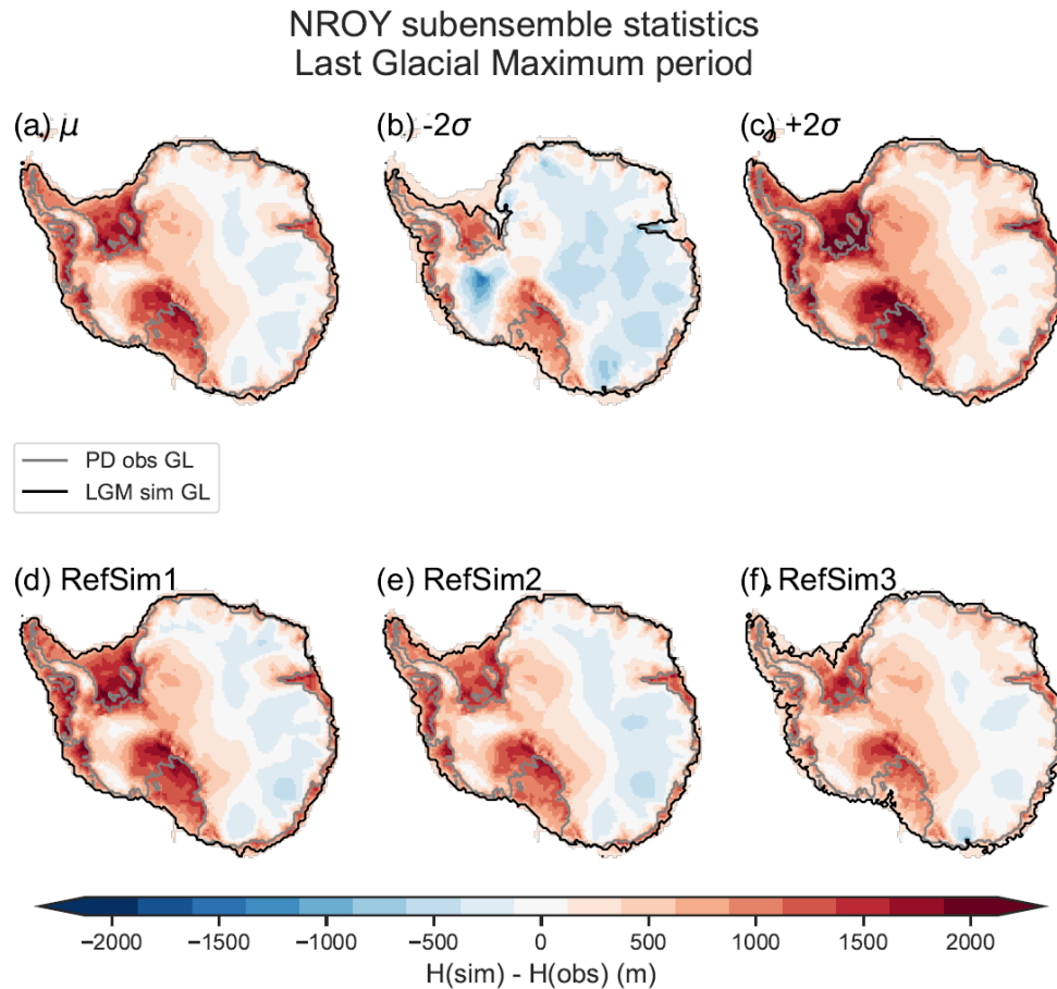
Figure 12: The not-ruled-out-yet (NROY) AN3sig sub-ensemble a) mean and b-c) 2\sigma range are shown during the LGM. Three glaciology self-consistent simulations chosen from a NROY high variance subset (HVSS) are showcased: d) RefSim1; e) RefSim2; f) RefSim3. The 2\sigma ranges are the nominal 95% ensemble intervals based on the equivalent Gaussian quantiles.
