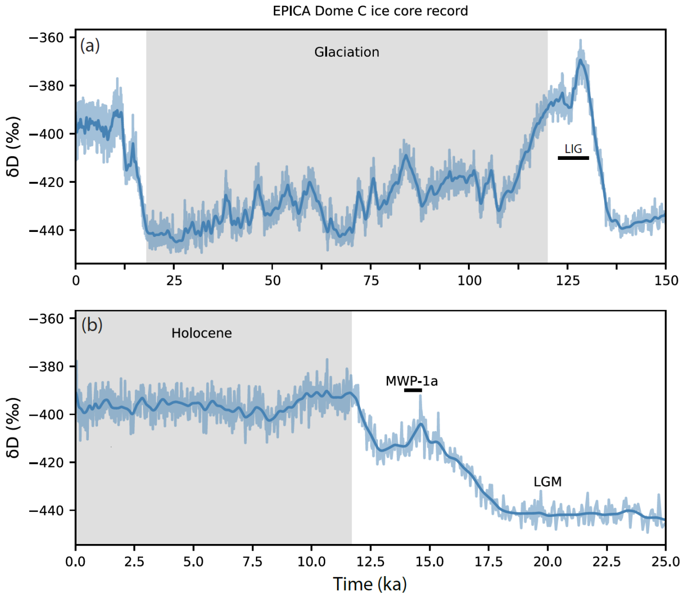
85 Figure 2: The EPICA Dome C deuterium record spanning (a) the time since the Last Interglacial (LIG), and b) the Last Glacial Maximum (LGM), post-LGM deglaciation (including Meltwater Pulse 1a, MWP1a) and the Holocene.
