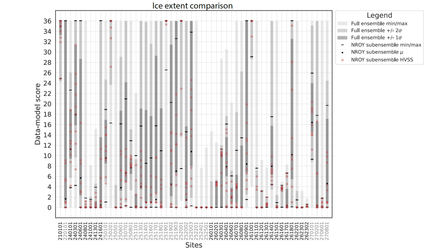
Figure 4: Past ice extent data-model comparison scores for the highest quality tier-1 data in AntICE2. The grey shading represents the min/max, 1\sigma and 2\sigma ranges of the full ensemble. The solid black circles and lines are the mean and min/max ranges for the not-ruled-out-yet (NROY) AN3sig sub-ensemble. Simulations consisting of a high variance subset (HVSS) of the NROY AN3sig sub-ensemble are shown as red circles. The 2\sigma and 1\sigma ranges are the nominal 95% and 68% ensemble intervals based on the equivalent Gaussian quantiles, respectively. The AntICE2 paleoExt data ID are shown in Figure S1.
