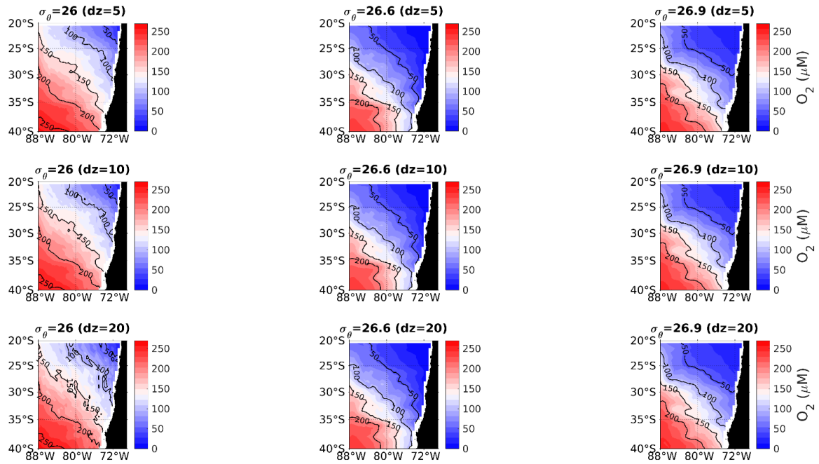
Figure 1. Comparison of isopycnals 26, 26.6, and 26.9 kg/m 3 using different vertical interpolations (dz: 5 m, 10 m, and 20 m) for the modeled average oxygen (9 years). The contours (black lines) represent oxygen concentrations of 50, 100, 150, 200, and 250 μM.
