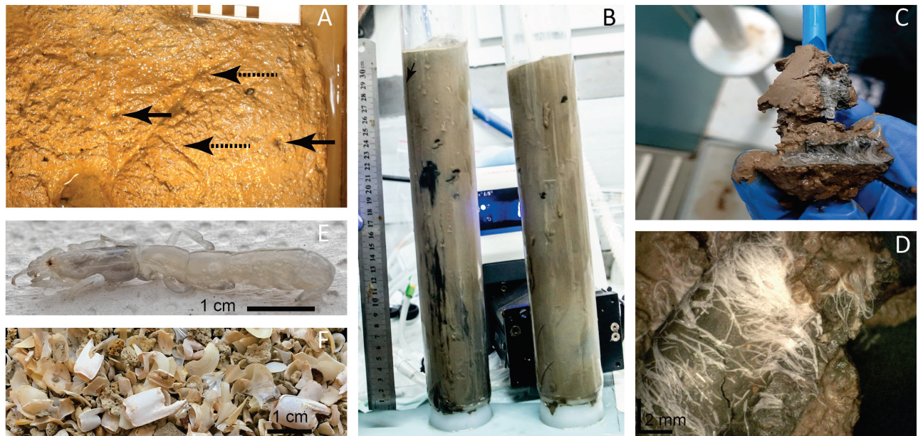
260 Figure 3. Burrows of the ghost shrimp Calliax lobata near active seepage sites within Palmahim Disturbance in the Eastern Mediterranean Sea. A) The seafloor, as exposed in the AC16-17BC1 box-core (RC1 area, 2016), shows burrow openings (black arrows) and scratches (dashed arrows) on the sediment surface. B) Image of RC20-BC1 and RC20-BC2 cores (RC1 area, 2020), showing dark coloration of burrows, unusual for the ambient sediments. C and D) Zooming into the burrows of RC20-BC1 and RC20-BC2 cores showed the presence of large filamentous microbes. E) Live C. lobata specimen found in AC16-17BC1. F) A multitude of C. lobata claws recovered through sporadic sieving (2 mm mesh) of AC16-17BC1.
