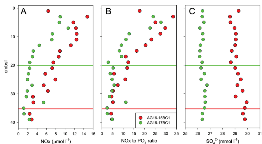
Figure 5: Pore water characteristics in cores AG16-15BC1 and AG16-17BC1: A) Nitrate+nitrite (NOx) concentration. B) NOx to phosphate ratio, C) Sulfate concentration. Red and green lines indicate the depths at which NOx concentrations appear to stabilize.
