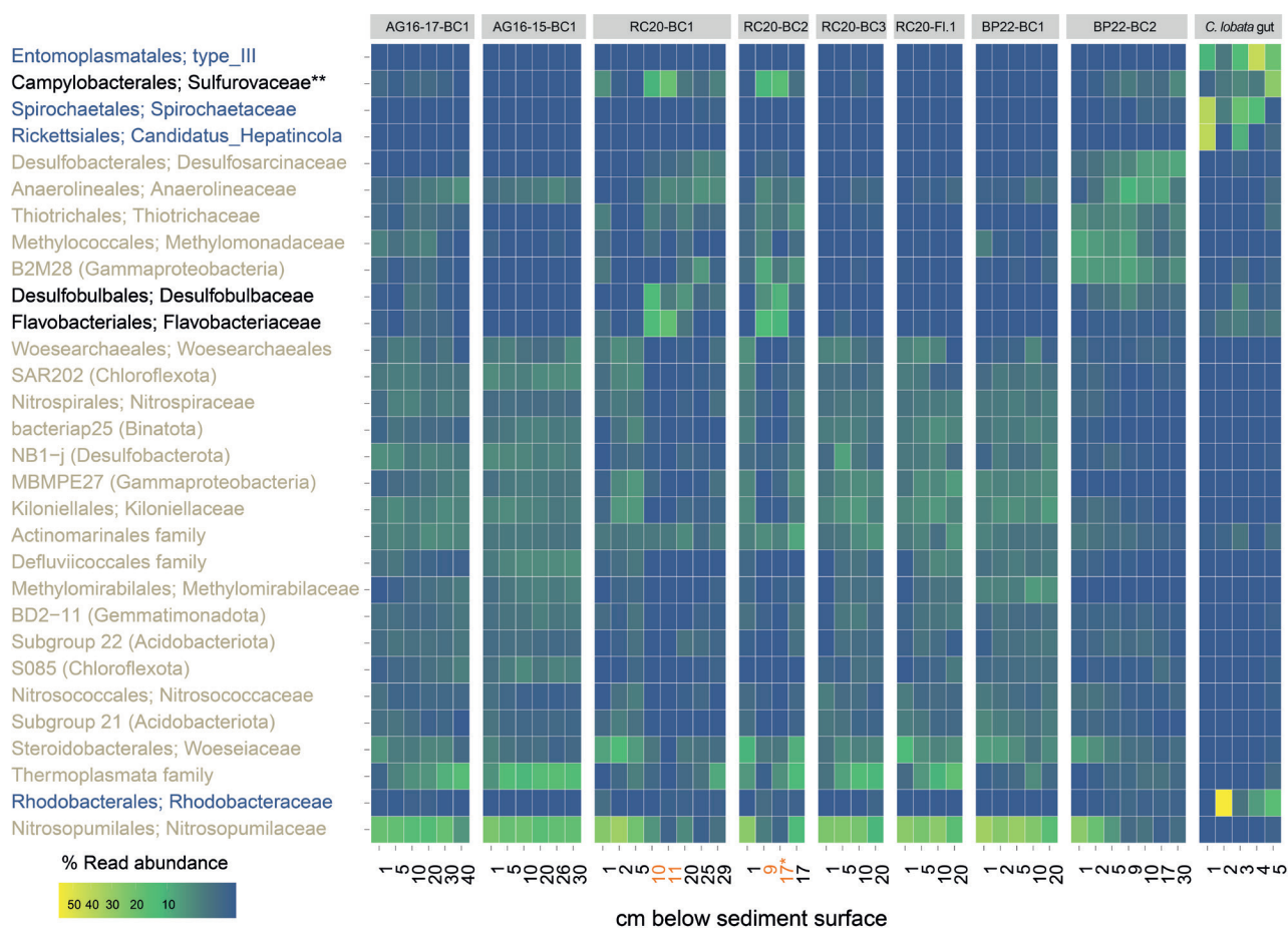
390 Figure 7: Read abundance of the top 30 most prevalent prokaryote taxa at the family level, in Palmahim sediments (see Table 1) and the hindgut of the ghost shrimp Callinectes lobata (black: enriched in burrows, blue: enriched in C. lobata , brown: enriched in sediments). Sediment depths where burrow microbes were collected are highlighted in orange. * Both samples are from the 16-17 cm section, yet the first one is taken from the burrow and the second from background sediments. ** abundant in burrows and associated with C. lobata hindgut.
