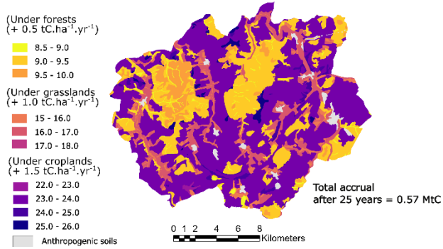
Figure F2: SOC accrual after 25 years under a scenario of additional C inputs dependent on land use, (a) with temperatures staying at their 2018 level, and (b) with a 1.0 °C increase in temperature over 25 years, increasing the C mineralization rates according to the correction factors of the AMG model. The attenuation in SOC accrual due to increased mineralization rates is (0.49 - 0.57) / 0.57 = 14\% . The 1.0 °C increase in temperature was obtained from model simulations of mean annual temperatures by the Meteo France ALADIN63_CNRM-CM5 model under scenario RCP4.5, within an 8 km radius area around Bure (55087), comparing the year intervals 2046-2055 and 2009-2019. Source: Drias, données Météo-France, CERFACS, IPSL.
