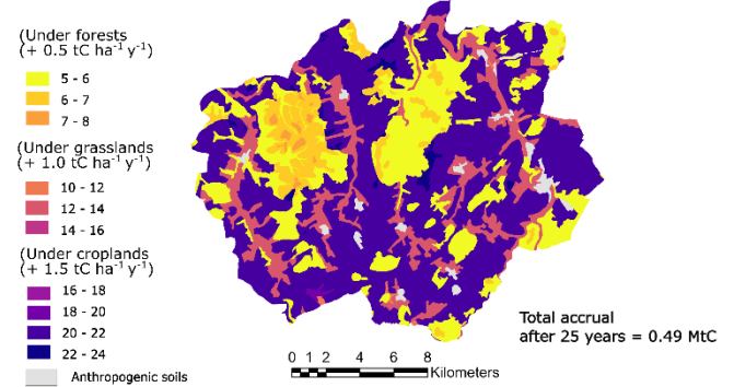
Figure F2: SOC accrual after 25 years under a scenario of additional C inputs dependent on land use, (a) with temperatures staying at their 2018 level, and (b) with a 1.0 °C increase in temperature over 25 years, increasing the C mineralization rates according to the correction factors of the AMG model. The attenuation in SOC accrual due to increased mineralization rates is (0.49 - 0.57) / 0.57 = 14\% . The 1.0 °C increase in temperature was obtained from model simulations of mean annual temperatures by the Meteo France ALADIN63_CNRM-CM5 model under scenario RCP4.5, within an 8 km radius area around Bure (55087), comparing the year intervals 2046-2055 and 2009-2019. Source: Drias, données Météo-France, CERFACS, IPSL.
