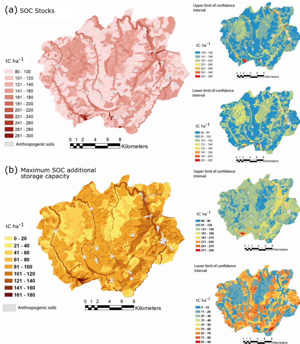
765 Figure F1: SOC stocks and maximum SOC additional storage capacity, with lower and upper confidence intervals as estimated by the bootstrap method. The SOC stock in the region of study ranges from 2.4 – 5.3 MtC and the maximum SOC additional storage capacity 1.2 - 4.1 MtC.
