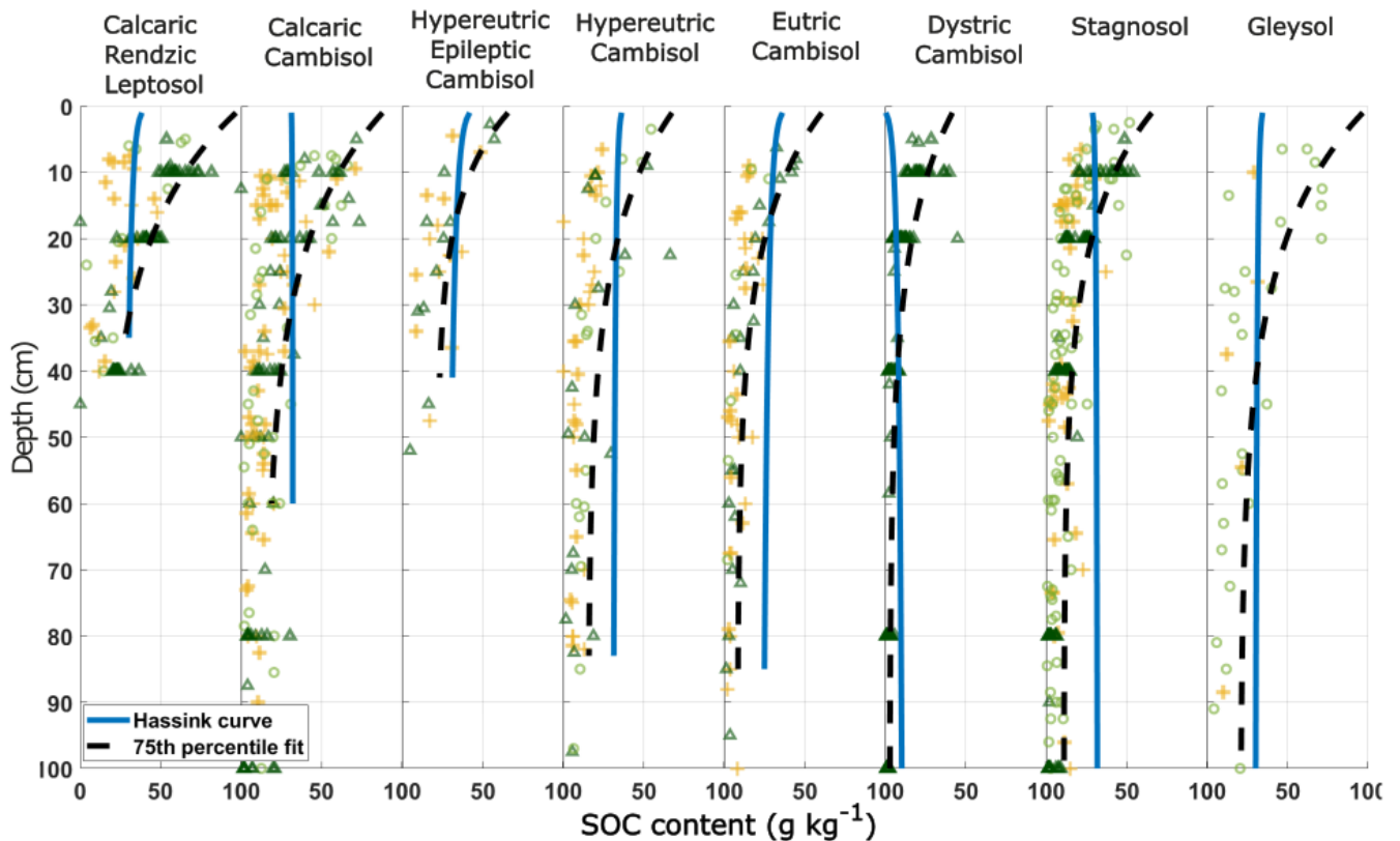
790 Figure H1: Carbon saturation curves from Hassink as a function of depth. The Hassink equation was established empirically on the basis of 20 Dutch grassland soils considered to be at the stationary state, as follows: C_{sat} = 4.09 + 0.37 * (\text{Clay} + \text{fine Silt}) (\%) where C_{sat} is the theoretical carbon saturation concentration in the fine fraction in \text{g kg}^{-1} . The Hassink equation provides unrealistic profiles of maximum SOC content distribution in the fine fraction at depth below 30 cm, especially in the Hypereutric Cambisol, Eutric Cambisol and Stagnosol, as the equation only accounts for soil texture and does not consider the biotic controls on C inputs and SOC decomposition rates. As comparison, the 75 th percentile fit represents a theoretical maximum SOC content in both the fine fraction and the particulate organic matter.
