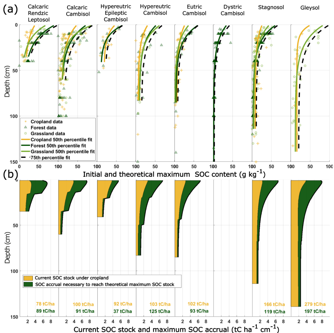
Figure 3: (a) Median (50 th percentile of the dataset for each land use) and theoretical maximum (75 th percentile of the dataset) fitted depth profiles of SOC content in each soil type. The Jreich parameters (2018) used to plot the SOC content profiles are given in Table A2. (b) Current SOC stocks under croplands and maximum SOC accrual to reach the theoretical maximum SOC stocks of each soil type.
