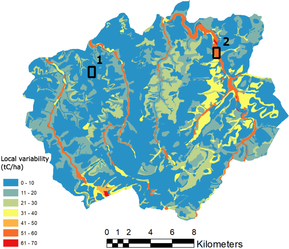
750 Figure D1: Local uncertainty of SOC linked to the non-explicit repartition of soil types within the cartographic units. As an example, in zone 1, which is under forest, the represented soil types are 80% Eutric cambisol (157 tC ha -1 ) and 20% Stagnosol (172 tC ha -1 ). In zone 2, which is under grassland, the represented soil types are 80% Stagnosol (161 tC ha -1 ) and 20% Gleysol (333 tC ha -1 ). For this reason, the local variability of SOC stocks is higher in zone 2 than zone 1.
