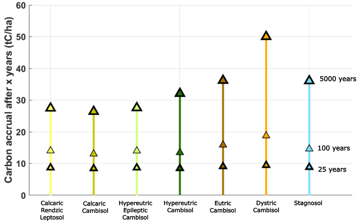
Figure 4: Model results of SOC accrual after 25, 100 and 5000 years under forests for a scenario of +0.5 \text{ tC ha}^{-1} \text{ y}^{-1} compared to the initial C inputs, temperature remaining constant.
