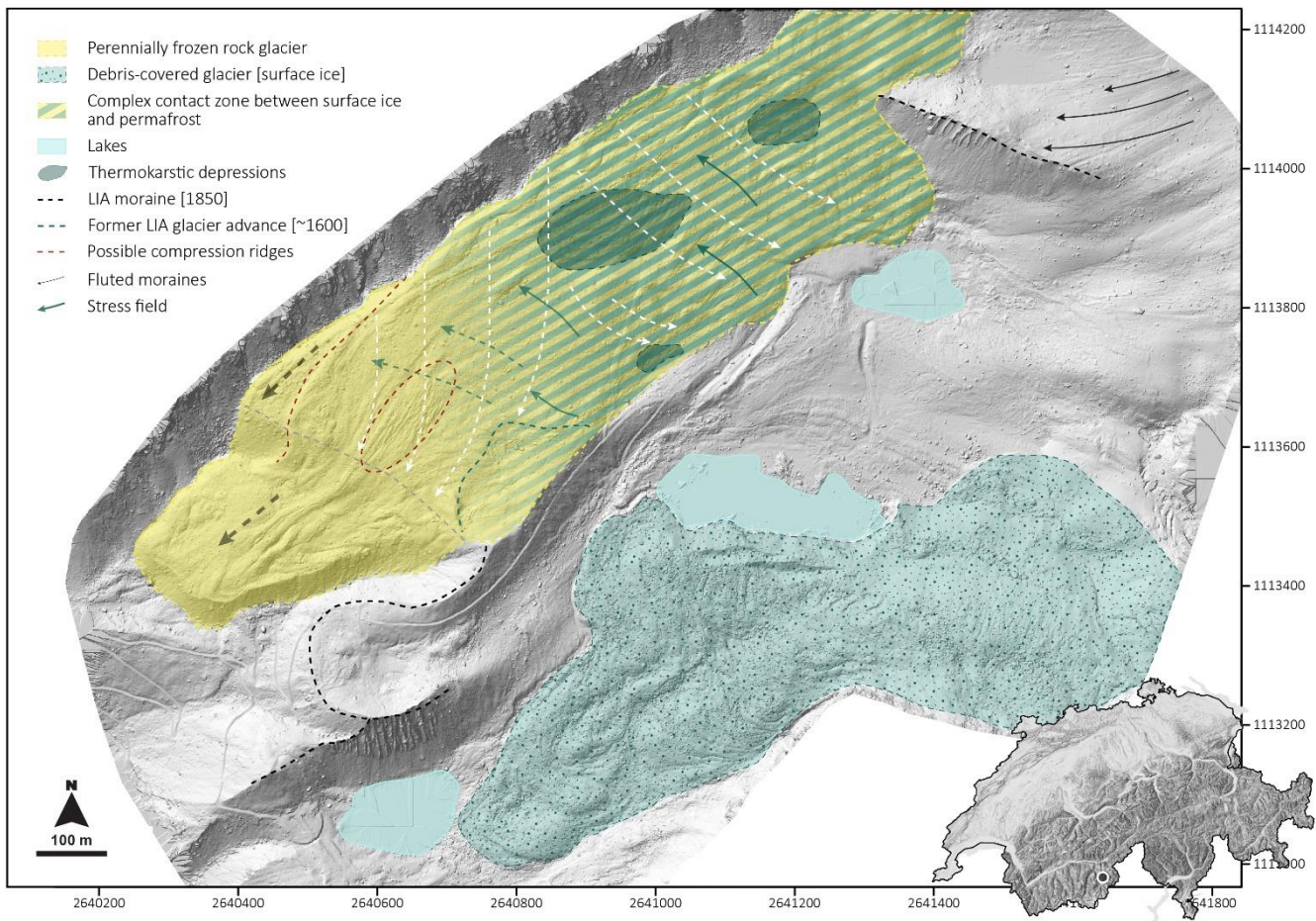
595 Figure 13: Interpretation of the influence of the LIA glacier-permafrost interaction on the mechanical behaviour of the rock glacier and its adjacent complex contact zone based on the analysis of high-resolution photogrammetry. The dashed black line represents the LIA (1850) moraine, and consequently the maximal extent of the Gruben glacier during its LIA apogee. The dashed grey line represents the topographical rupture. The dark blue arrows represent the stress exerted by the glacier onto the rock glacier. The white dashed arrows show the reoriented flow trajectories of the rock glacier and complex contact zone as a response to the stress exerted by the LIA glacier, while the grey dashed arrows show the unchanged flow trajectory of the rock glacier. The blue dashed line shows the probable extent of a prior stage (~1600) of LIA glacier advance. The dark red dashed line on the orographic right side of the rock glacier and the dashed ellipse shows compression ridges likely due to the glacier stress. Background: UAV-derived hillshade (06.10.2022). 600
