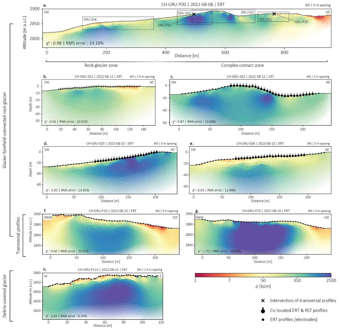
Figure 4: The main longitudinal ERT profile GRU-P00 is presented in the uppermost panel (a). ERT profiles GRU-S01, GRU-S02, GRU-S03 and GRU-S04 are presented in panels (b-e) and represent the profiles where both ERT and RST measurements were carried out. The transversal profiles GRU-P10 and GRU-P23 are presented in panels (f-g). Profile GRU-P115, carried out on the debris-covered glacier is presented in panel (h).
