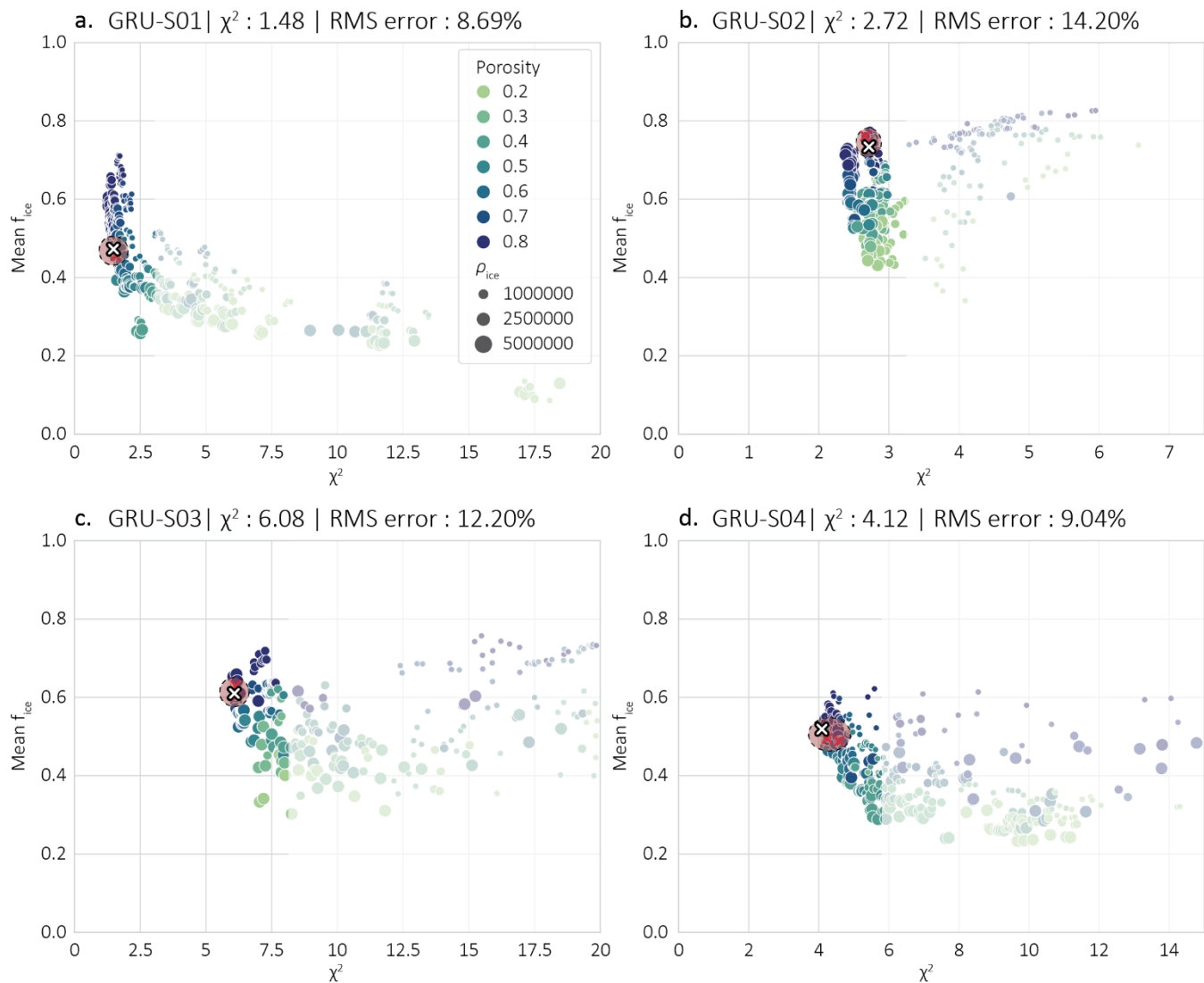
530 Figure 11: Sensitivity analysis of mean ice content ( f_{ice} ) for the entire tomogram and model-fit \chi^2 to the prescribed porosity and resistivity of ice ( \rho_{ice} ) for profiles GRU-S01 (a), GRU-S02 (b), GRU-S03 (c) and GRU-S04 (d). \chi^2 and RMS error indicated in the title correspond to the PJI chosen for interpretation. The white cross represents the chosen model, and the red crosses represent the models with the same set of prescribed parameters aside from \rho_w . The red circle represents the uncertainty range for \rho_w on the estimated mean ice content.
