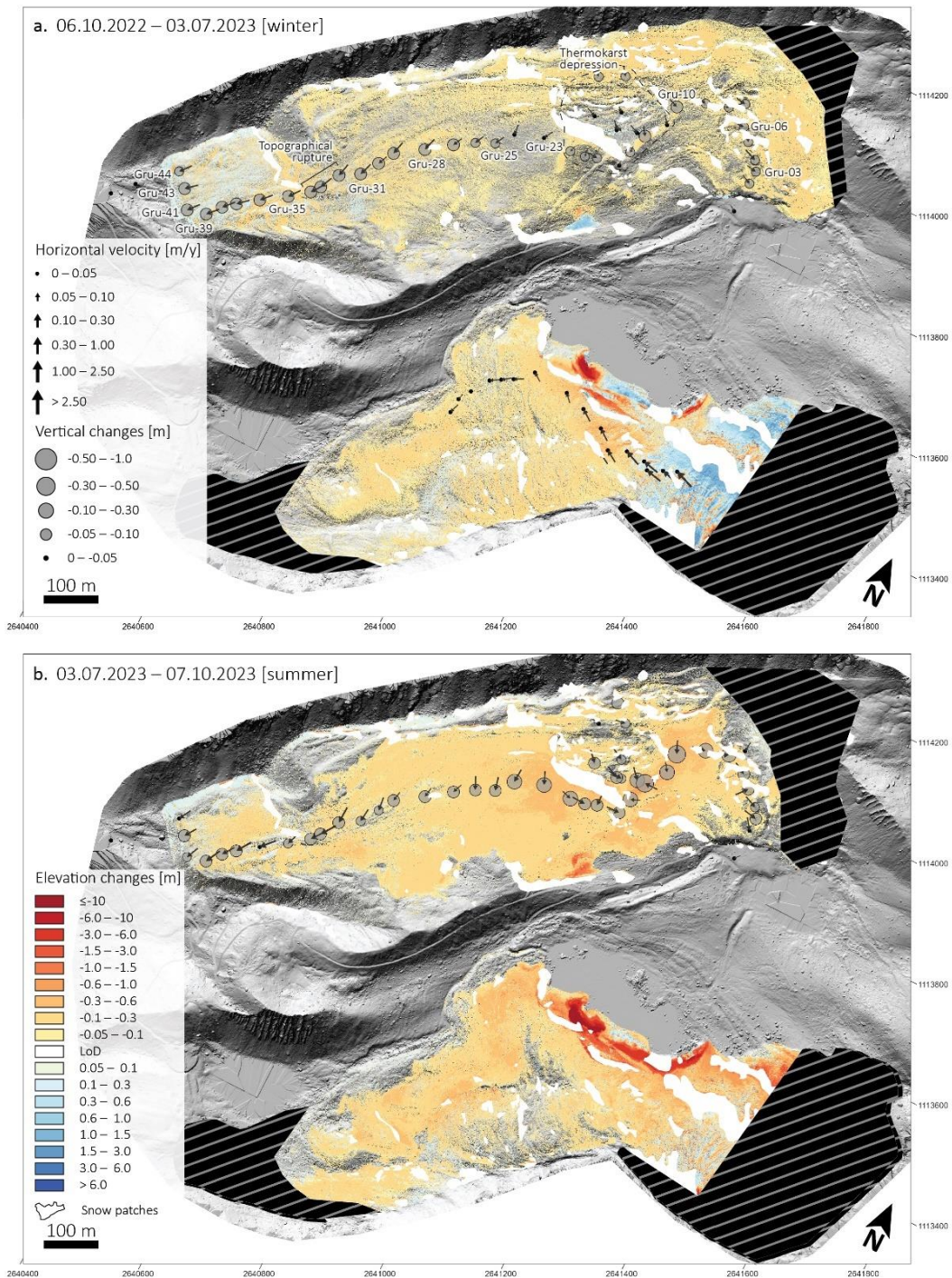
440 Figure 7: Seasonal elevation changes derived from DoD. Vertical changes and horizontal surface displacements derived from TGS. The measured points are identified by their corresponding number (Gru-xx, only in panel (a)). The winter period (06.10.2022 to 03.07.2023) is presented in panel (a) and the summer period (03.07.2023 to 07.10.2023) is presented in panel (b). Background: UAV-derived hillshade (06.10.2022).
