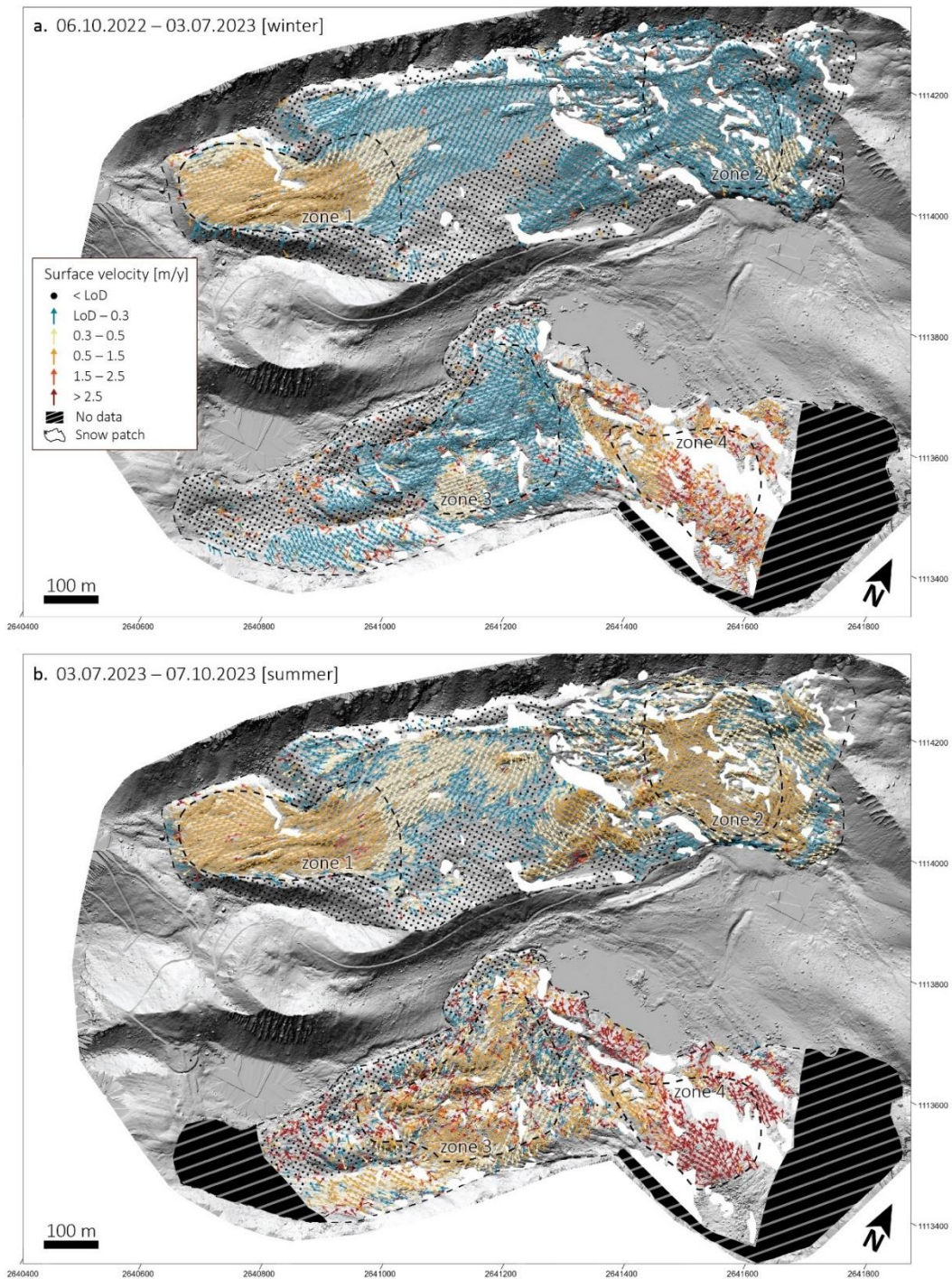
Figure 6: UAV-derived horizontal surface displacements. The winter period (06.10.2022 to 03.07.2023) is presented in panel (a) and the summer period (03.07.2023 to 07.10.2023) is presented in panel (b). The zones (1-4) from which the mean velocities are derived from are highlighted by the dashed polygons. Background: UAV-derived hillshade (06.10.2022).
