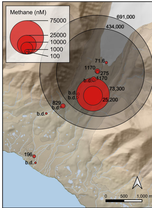
320 Figure 9. Methane concentrations (nM) of groundwater springs in the forefield of Vallåkrabreen. Bubble size is proportional to methane concentration. Red bubbles represent springs sampled during one-time spatial sampling, while black bubbles represent the average methane concentrations of the GW1 and GW2 springs (Kleber et al., 2024), with bubble size extrapolated on the same bubble size scale. Concentrations below the detection limit of 18 nM are indicated by b.d.
