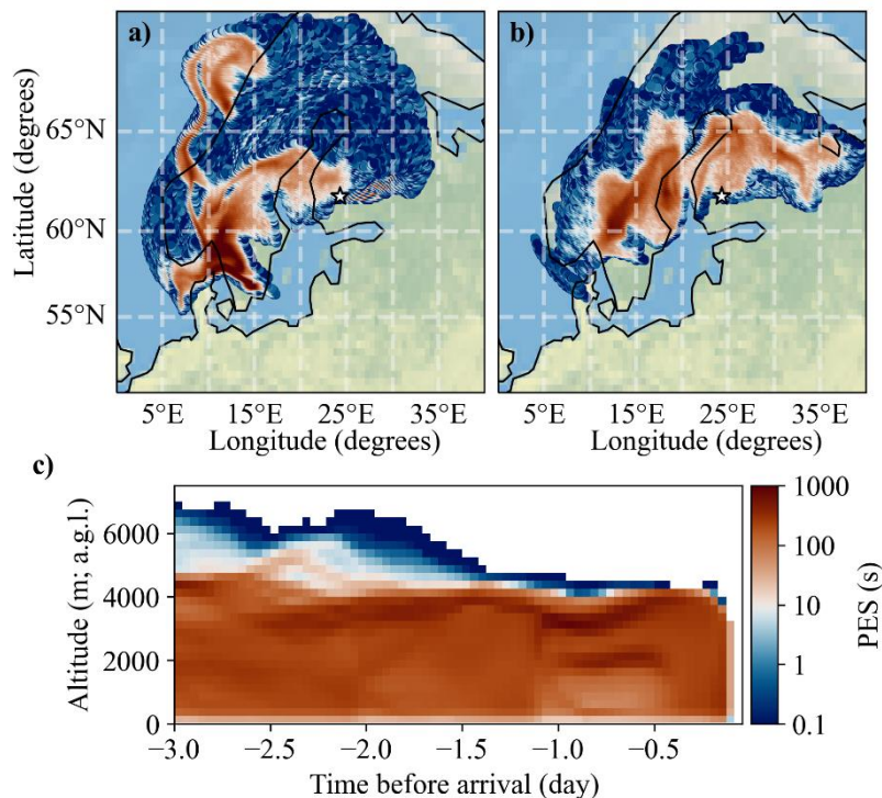
705 Figure 11. Airmass origin for the elevated layer at 3 km a.g.l. observed on 16.05.2018 at 14 (UTC+2) in SMEAR II. a) PES summed up for all heights above 3 km a.g.l. for 3 days before arrival at SMEAR II. b) Sum of PES in the lowest 1 km a.g.l. for 3 days before arrival at SMEAR II. c) Vertical distribution of PES for 3 days before arrival at SMEAR II.
