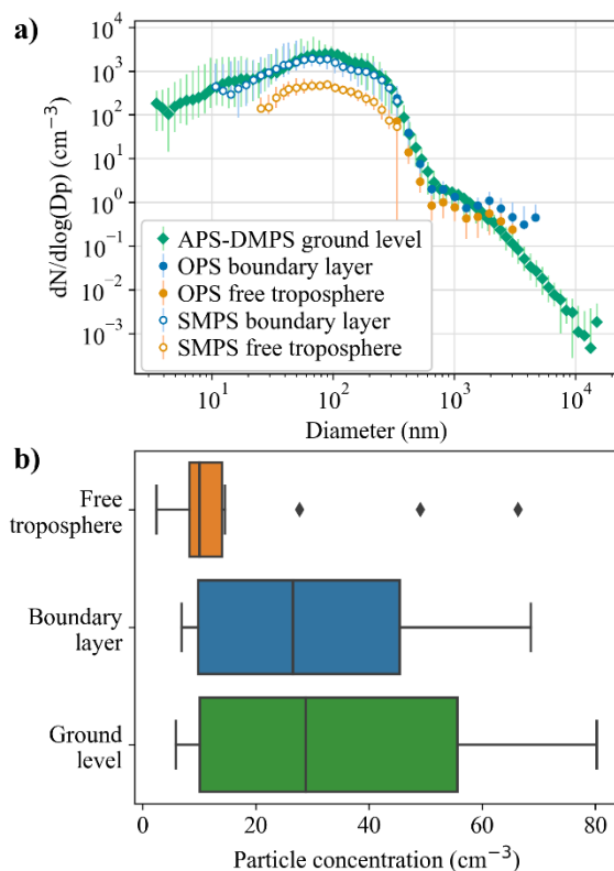
440 Figure 5: a) Median particle number size distributions calculated from ground-level measurements (SMEAR II APS and DMPS) as well as boundary layer and free troposphere measurements (aircraft SMPS and OPS) over the 19 flights of the campaign. The error bars represent the 25 th and 75 th percentiles. The size distribution shown with a linear scale can be seen in Fig. A4. b) Box plots of the concentration of particles > 300 nm measured at ground level, in the boundary layer and in the free troposphere calculated over all the flights.
