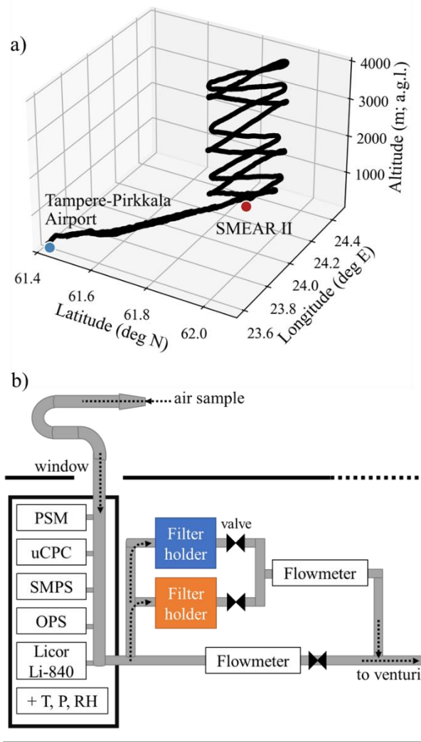
155 Figure 1: a) Example of a flight track from Tampere-Pirkkala airport to SMEAR II. The distance from the airport to the station is approximately 60 km. The location of SMEAR II with respect to Northern Europe is given in Fig. A1. b) Schematic of the instrumental setup viewed from above inside the Cessna 172, described in detail in Section 2.1.1.
