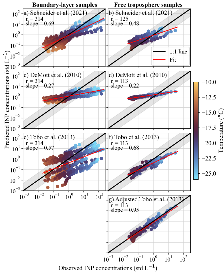
510 Figure 7. Comparison between the INP concentrations observed in the boundary layer (left side) and the free troposphere (right side) and the INP concentrations predicted using the parameterizations from a) and b) Schneider et al. (2021), c) and d) DeMott et al. (2010), and e) and f) Tobo et al. (2013). The black solid line represents the 1:1 line while the grey shaded area indicates a range of a factor of 5 from the 1:1 line. The red solid lines show a linear regression fit through the logarithmically transformed data points. The slope of the fit and the number of data points used is shown in each panel.
