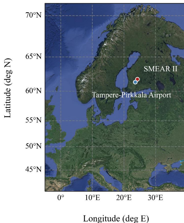
740 Figure A1. Location of the Tampere-Pirkkala airport and SMEAR II with respect to Northern Europe.
