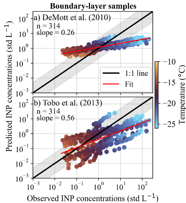
775 Figure A5. Comparison between the INP concentrations observed in the boundary layer and the INP concentrations predicted using the parameterizations from a) DeMott et al. (2010), and b) Tobo et al. (2013) using the aircraft OPS data. DeMott et al. (2010) reproduces 60 % and 32 % of the data points within a factor of 5 and 2, respectively. Tobo et al. (2013) reproduces 49 % and 17 % of the data points within a factor of 5 and 2, respectively. The black solid line represents the 1:1 line while the grey shaded area indicates a range of a factor of 5 from the 1:1 line. The red solid lines show a linear regression fit through the logarithmically transformed data points. The slope of the fit and the number of data points used is shown in each panel.
