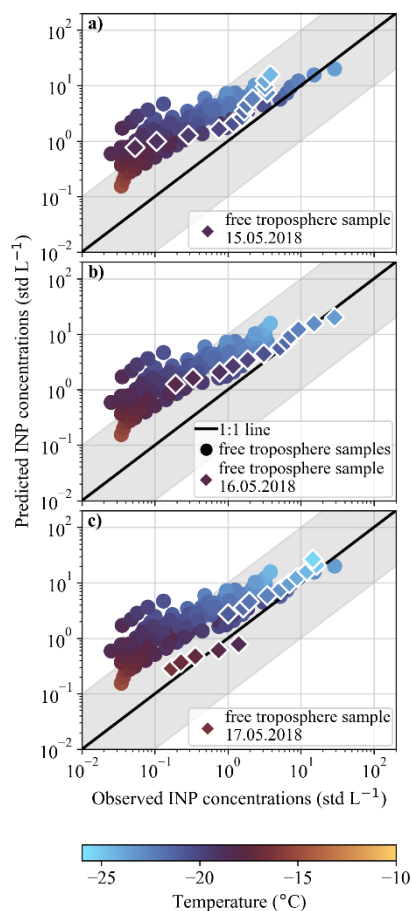
Figure A7. Comparison between the observed and the predicted INP concentrations calculated using the parameterization from Schneider et al. (2021) for the free troposphere samples collected on the three consecutive days of the case study. In each panel, the diamond markers represent a specific free troposphere sample sampled on a) 15 May, b) 16 May, and c) 17 May 2018, plotted on top of all the free troposphere samples collected during the campaign. The black solid line represents the 1:1 line while the grey shaded area indicates a deviation of 1 order of magnitude from the 1:1 line. The parameterization from Schneider et al. (2021) was calculated using the ground-level ambient air temperature measured at 4.2 m a.g.l. and averaged over the sampling time of each sample.
