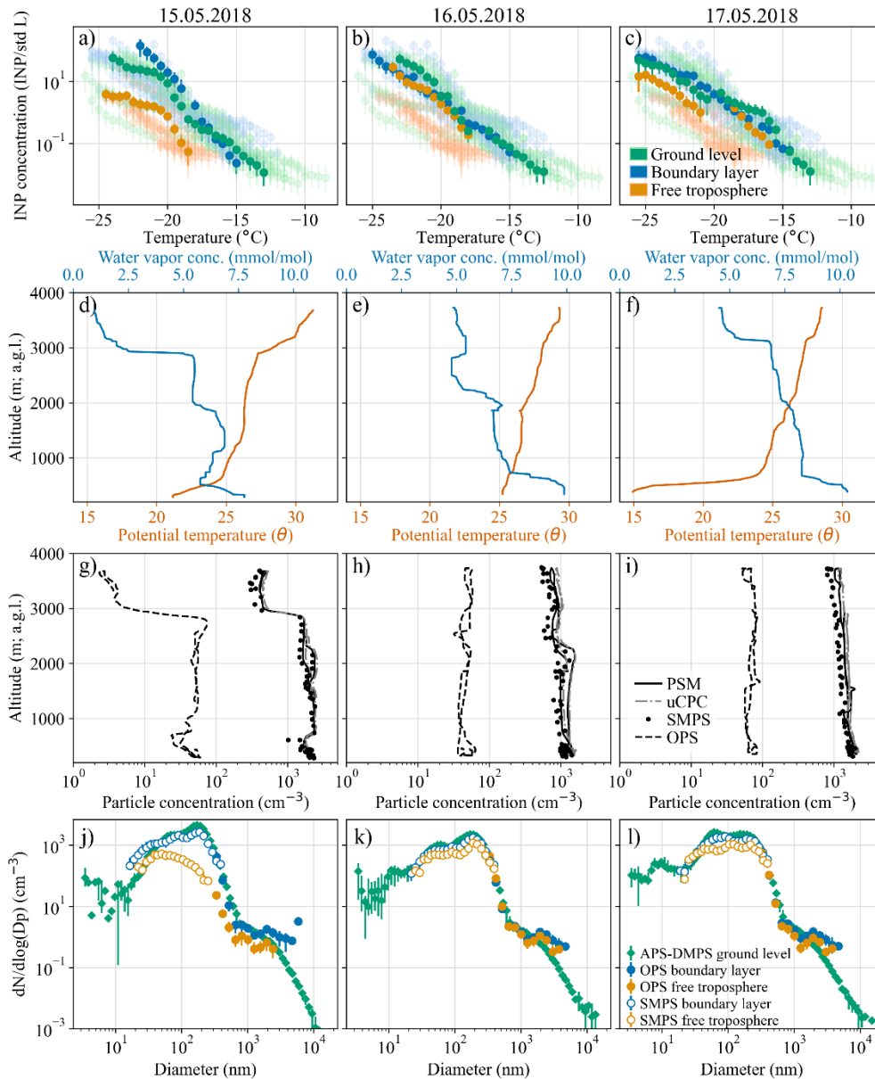
620 Figure 9. a), b) and c) INP temperature spectra for the three flights of the case study (15, 16 and 17 May 2018), plotted on top of the complete dataset (transparent data points) as in Fig. A2c. d), e) and f) Potential temperature and water vapor concentration plotted as a function of altitude during the ascents, which occurred between 05:30 and 06:20 (UTC+2) on 15 May; between 13:40 and 14:20 (UTC+2) on 16 May; and between 08:40 and 09:20 (UTC+2) on 17 May 2018. g), h) and i) Particle concentrations as a function of altitude. j), k) and l) Median particle number size distributions for the three consecutive flights of the case study. The size ranges of the particle counters used onboard the aircraft are > 1.5 nm for the PSM, > 3 nm for the uCPC, > 10 nm for the SMPS and > 300 nm for the OPS. 625
