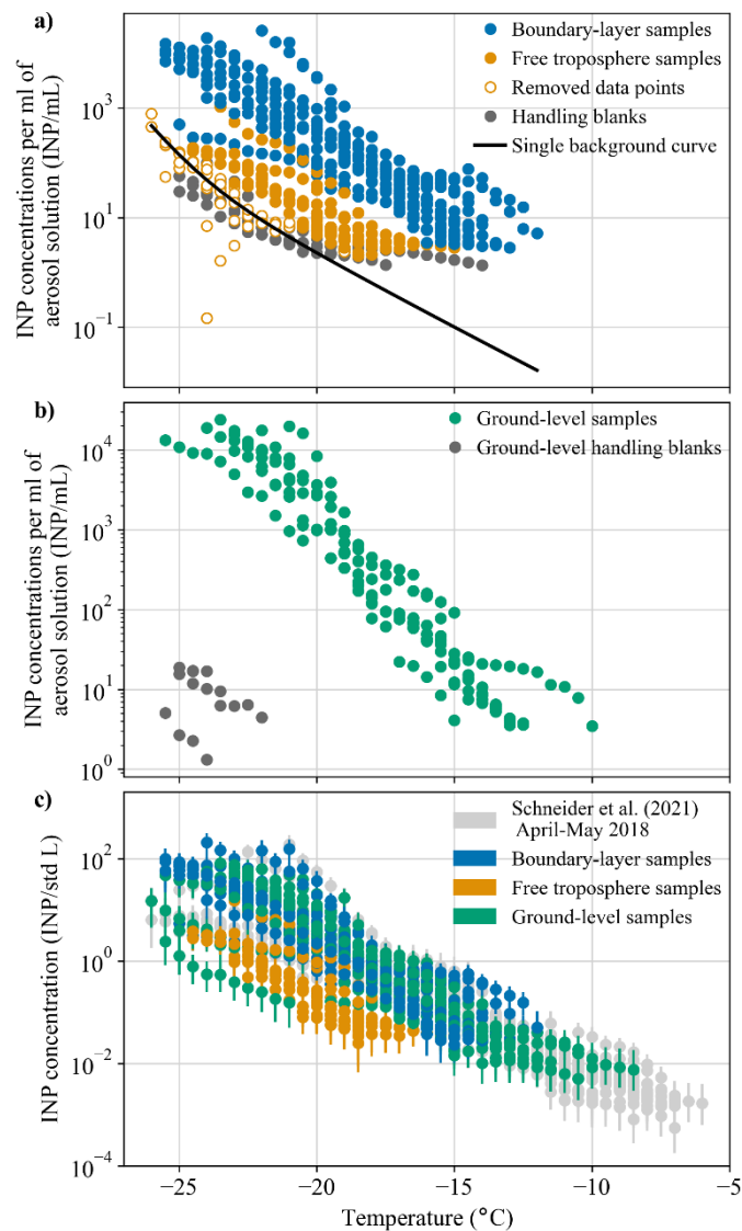
750 Figure A2. a) INP concentrations per ml of aerosol solution from the aircraft samples compared to the background signal derived 755 from the handling blank filters collected onboard the aircraft. b) INP concentrations per ml of aerosol solution from the ground- level samples collected at SMEAR II at the same time as the aircraft samples compared to the ground-level handling blank filters. c) INP temperature spectra of all the samples collected during the aircraft measurement campaign together with the ground-level data from Schneider et al. (2021) collected in Hyytiälä during April and May 2018. The error bars represent the statistical as well as the systematic error of the INSEKT assay. More details related to the calculation of these error bars is given in Schneider et al. (2021).
