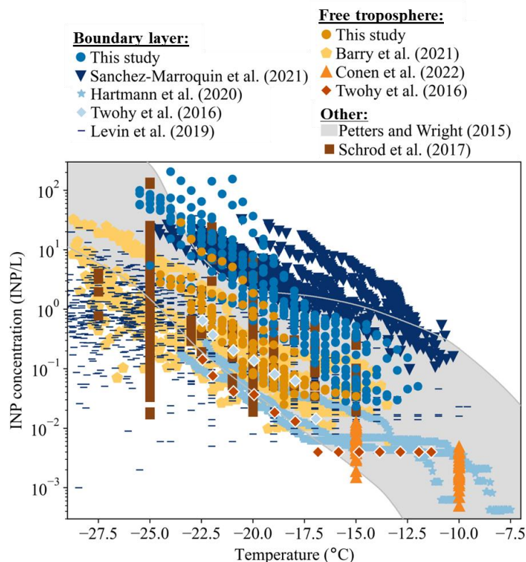
575 Figure 8. INP concentrations from the present study compared with literature data. The measurements from Sanchez-Marroquin et al. (2021) were conducted in the boundary layer in the South East of the British Isles, while Hartmann et al. (2020) conducted their measurements in the High Arctic boundary layer. For the Twohy et al. (2016) data collected in the western United States, the light blue diamonds represent a filter sampled within the boundary layer (at 1067 m a.g.l.), while the dark orange diamonds represent a filter sampled primarily in the free troposphere (between 897 and 3638 m a.g.l.). For the Levin et al. (2019) study conducted in California, the data represented here correspond to the measurements made in the boundary layer (below 2 km). The measurements from Barry et al. (2021) were conducted between 1300 and 5100 m above sea level in the western United States. The measurements from Conen et al. (2022) were conducted under free troposphere conditions at Jungfrauoch (3580 m above sea level) in the Swiss Alps. The grey band represents the data range given in Petters and Wright (2015) derived from precipitation samples collected around the world. The measurements from Schrod et al. (2017) were conducted between 500 and 2500 m a.g.l. (likely both in the boundary layer and in the free troposphere) over the Eastern Mediterranean.
