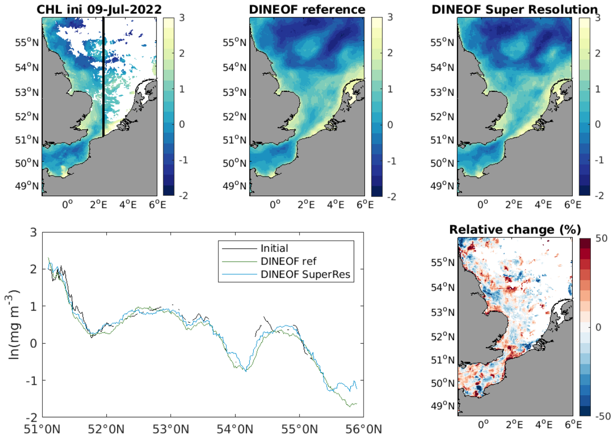
Figure 14. Top left: initially cloudy data with a 1 km resolution, on 9 July 2022. Top center: DINEOF reconstruction of the 1 km data (reference run). Top right: DINEOF run of the mixed dataset. Bottom: north-south transect for the three datasets (black: initial data at 1 and 5 km; green: reference run at 1km; blue: super-resolution run). Bottom right: percentage difference map between the initial data and the DINEOF estimate. Data in logarithmic scale.
