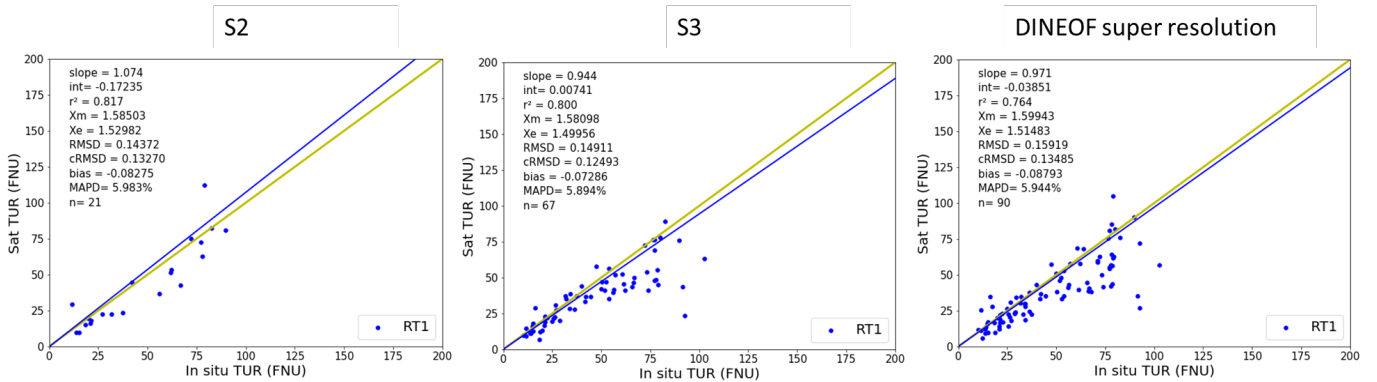
Figure 11. Matchup results of daily Sentinel-2, Sentinel-3 and DINEOF super resolution TUR products against in situ observations obtained from the autonomous PANTHYR system at the RT1 station in the Belgian Coastal Zone.
