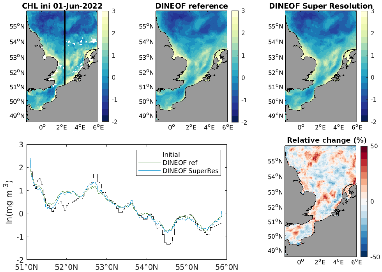
Figure 12. Top left: initially cloudy data with a \pm 5 km resolution, on 1 June 2022. Top center: DINEOF reconstruction of the \pm 5 km data (reference run). Top right: DINEOF run of the mixed dataset. Bottom left: north-south transect for the three datasets (black: initial data at 1 and 5 km; green: reference run at 1 km; blue: super-resolution run). Bottom right: percentage difference map between the initial data and the DINEOF estimate. Data in logarithmic scale.
