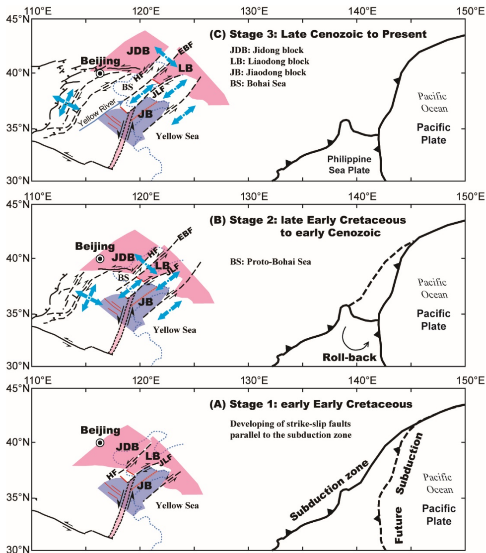
365 Figure 9: Proposed three-stage model for the formation of the Bohai Sea Basin as a result of complex faulting in Bohai Sea area and roll-back of the West Pacific and Philippine Sea plate subduction. JDB, the Jidong Block. LB, the Liaodong Block. JB, the Jiaodong Block. BS, the Bohai Sea Basin.
