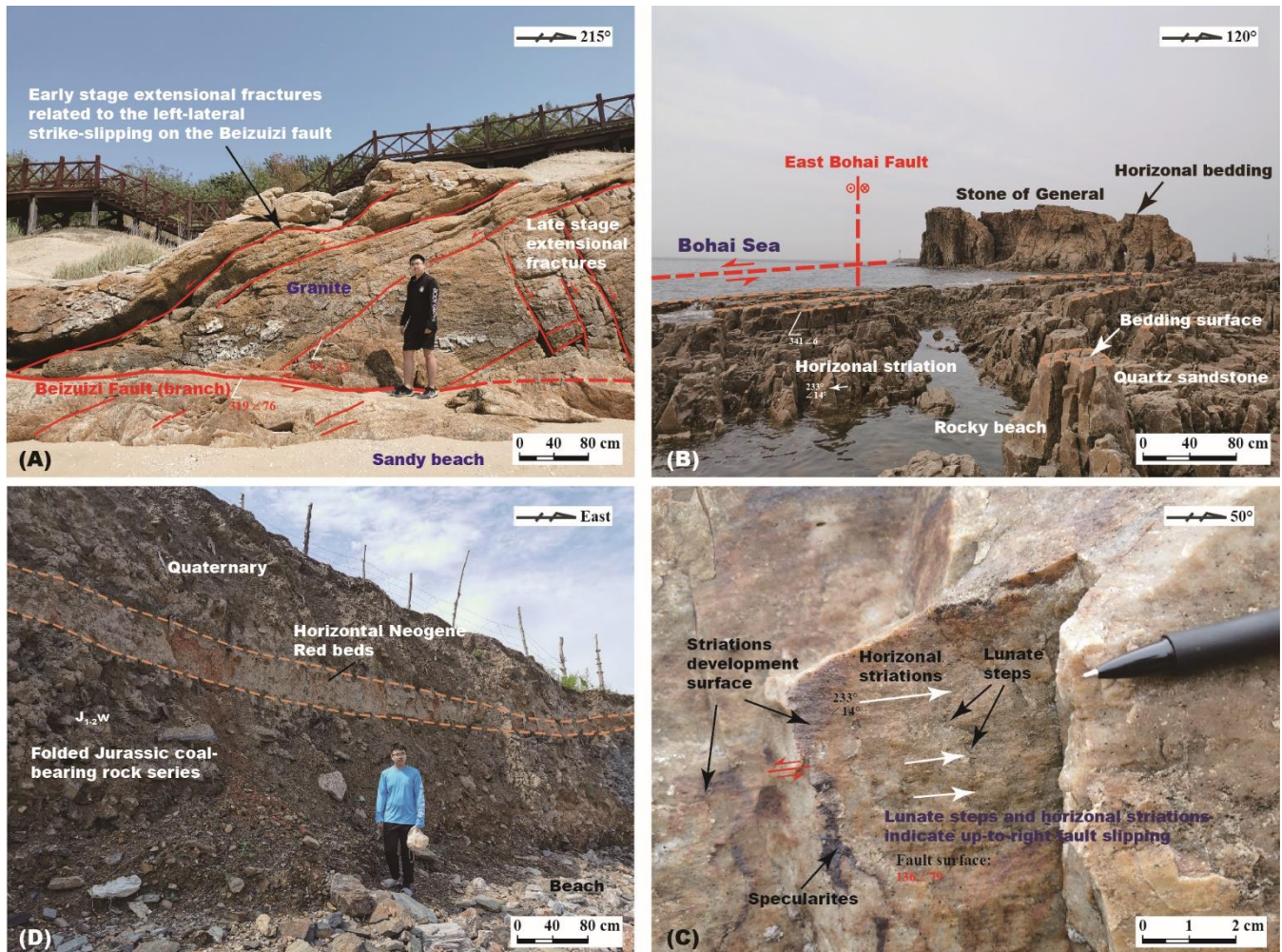
260 Figure 7: (A) The Beizuizi fault, a branch of the East Bohai fault, occurs in northwestern coast of the Liaodong Peninsula, showing a left-lateral strike-slip movement similar to that on the Honglazi fault in Fig. 5. Section view. Both the Beizuizi and Honglazi faults are considered as relic faults formed before the opening of the Bohai Sea. (B) Topographic feature in western coast of the Liaodong Peninsula, showing geometric properties of the East Bohai fault. (C) Near horizontal striations indicate early stage left-
