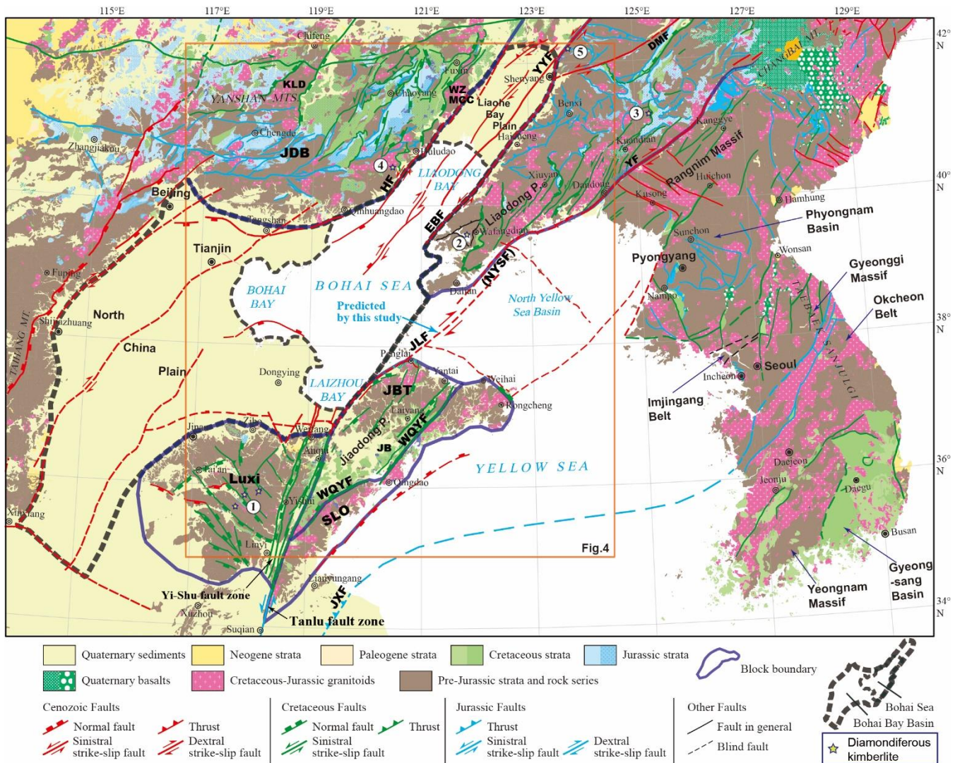
100 Figure 3: Sketched structural geological map of the Bohai Bay Basin and surrounding region (modified from Allen et al., 1997, China Geological Survey, 2004, Ren et al., 2013, Yin et al., 2015, Kim et al., 2018, Zhai et al., 2019, Yang et al., 2020, Lin et al., 2021, Ren et al., 2023, and Zhu et al., 2024). The Tan-Lu and Yi-Shu fault zones share a common segment of western boundary of the Sulu orogen. Diamondiferous kimberlites are from Liu et al., 2019. JDB, Jidong block. JBT, Jiaobei terrane. JB, Jiaolai basin. SLO, Sulu orogen. WZMCC, Waziyu (also named Yiwulvshan) MCC (Sun et al., 2022). KLD, Kalaqin Dome (Yang et al., 2020). HF, Honglazi fault. EBF, East Bohai fault. JLF, Jiao-Liao fault as the boundary faults of the Jiaodong and Liaodong peninsulas predicted in this study. NYSF, North Yellow Sea fault (Tian et al., 2007). YYF, Yilan-Yitong fault. DMF, Dun-Mi fault. YF, Yalvjiang fault. WQYF, Wulian-Qingdao-Yantai fault. JXF, Jiashan-Xiangshui fault. Diamondiferous kimberlites: 1, Mengyin; 2, Wafangdian; 3, Huanren; 4, Huludao; 5, Tieling. 105
