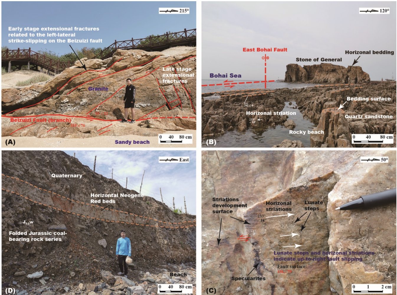
Figure 76: (A) The Beizuizi fault, a branch of the East Bohai fault, occurs in northwestern coast of the Liaodong Peninsula, showing a left-lateral strike-slip movement similar to that on the Honglazi fault in Fig. 5. Section view. Both the Beizuizi and Honglazi faults are considered as relic faults formed before the opening of the Bohai Sea. (B) Topographic feature in western coast of the Liaodong Peninsula, showing geometric properties of the East Bohai fault. (C) Near horizontal striations indicate early stage
