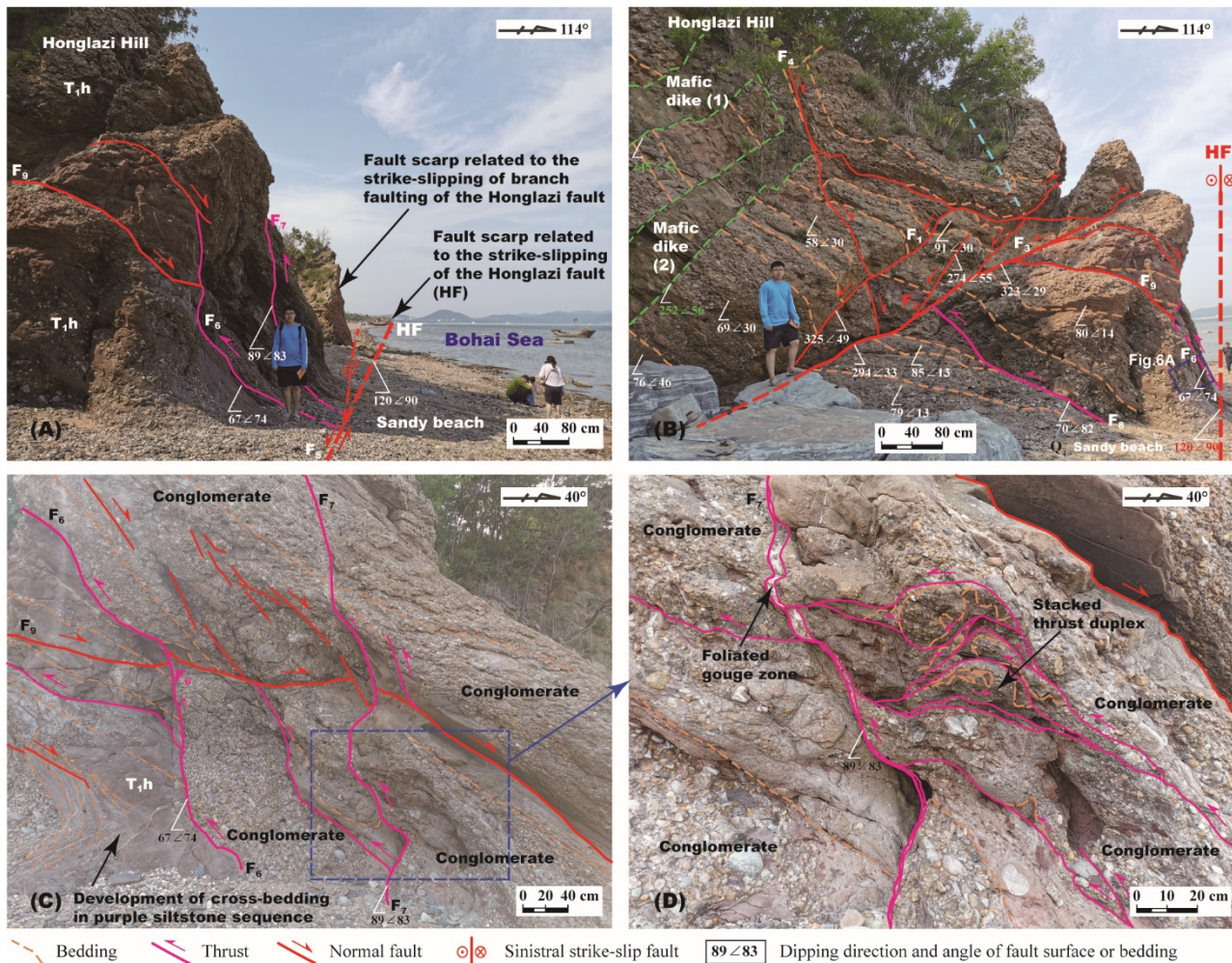
Figure 5: Structural analyses in northwestern coast of the Bohai Sea. (A) The Honglazi fault (HF) with flower structure in western coast of the Bohai Sea, formed in the Early Cretaceous. The flower structure is truncated by normal fault system. T 1,h , Honglazi Formation of the Lower Triassic. (B) Interpretation: Development of the extensional normal fault system with intrusion of mafic dikes later than the HF and the flower structure. (C) The western half thrust system of the flower structure related to the HF. (D) Duplex in the Lower Cretaceous related to the flower structure of the Honglazi fault. See Fig. 5B for location. (C) Uninterpreted picture of (B). T 1,h , Honglazi Formation of the Lower Triassic. Section view.
