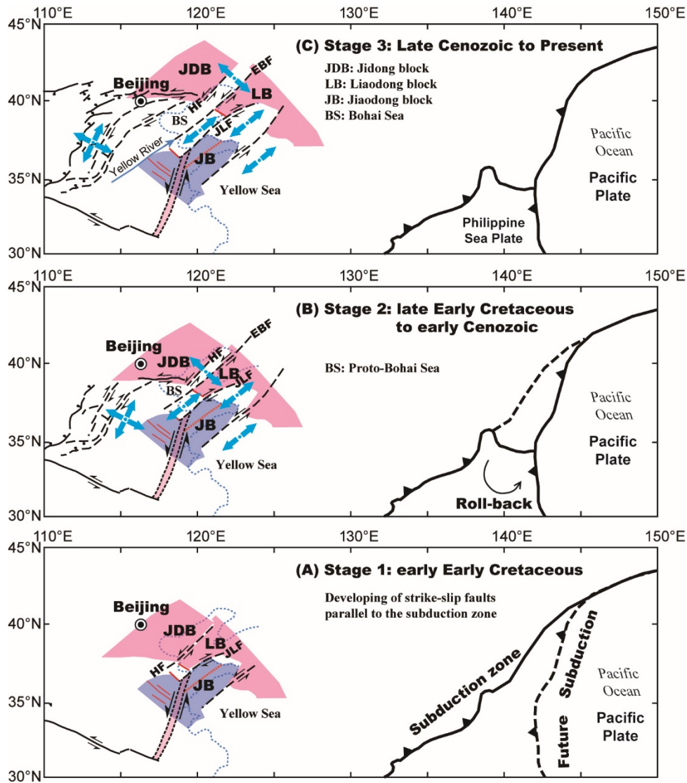
375 Figure 109: Proposed three-stage model for the formation of the Bohai Sea Basin as a result of complex faulting in Bohai Sea area and roll-back of the West Pacific and Philippine Sea plate subduction. JDB, the Jidong Block. LB, the Liaodong Block. JB, the Jiaodong Block. BS, the Bohai Sea Basin.
