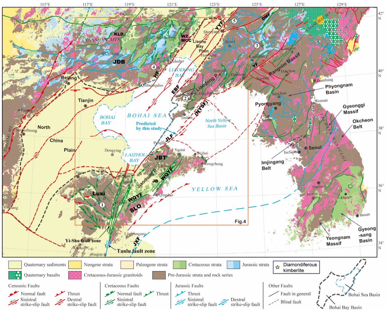
105 Figure 3: Sketched structural geological map of the Bohai Bay Basin and surrounding region (modified from Allen et al., 1997, China Geological Survey, 2004, Ren et al., 2013, Yin et al., 2015, Kim et al., 2018, Zhai et al., 2019, Yang et al., 2020, Lin et al., 2021, Ren et al., 2023, and Zhu et al., 2024). The Tan-Lu and Yi-Shu fault zones share a common segment of western boundary of the Sulu orogen. Diamondiferous kimberlites are from Liu et al., 2019. JDB, Jidong block. JBT, Jiaobei terrane. JB, Jiaolai basin. SLO, Sulu orogen. WZMCC, Waziyu (also named Yiwulvshan) MCC (Sun et al., 2022). KLD, Kalaqin Dome (Yang et al., 2020). HF, Honglazi fault. EBF, East Bohai fault. JLF, Jiao-Liao fault as the boundary faults of the Jiaodong and Liaodong peninsulas predicted in this study. NYSF, North Yellow Sea fault (Tian et al., 2007). YYF, Yilan-Yitong fault. DMF, Dun-Mi fault. YF, Yalvjiang fault. WQYF, Wulian-Qingdao-Yantai fault. JXF, Jiashan-Xiangshui fault. Diamondiferous kimberlites: 1, Mengyin; 2, Wafangdian; 3, Huanren; 4, Huludao; 5, Tieling. 110
