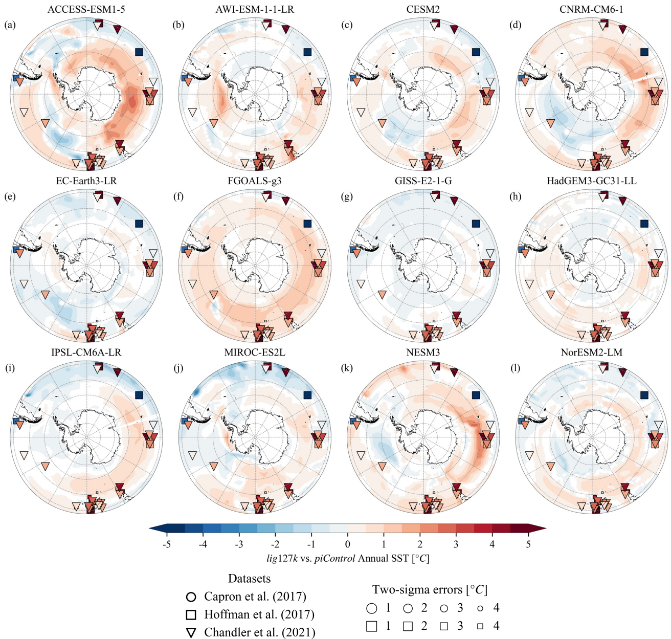
Figure 3. Differences in annual SST between lig127k and piControl simulations. Paleoproxies in each subfigure are from Fig. 1a. We only show differences-temperature anomalies that are significant at 5% level based on the student's t-test with Benjamini-Hochberg Procedure controlling false discovery rates (Benjamini and Hochberg, 1995).
