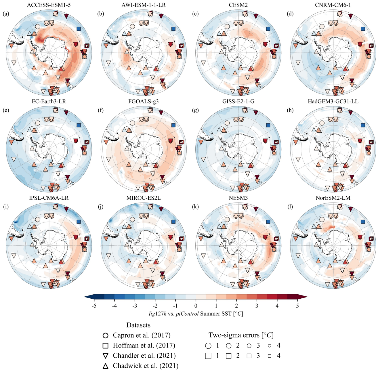
Figure 4. Differences in summer SST between lig127k and piControl simulations. Paleo proxies in each subfigure are from Fig. 1b. We only show differences temperature anomalies that are significant at 5% level based on the student's t-test with Benjamini-Hochberg Procedure controlling false discovery rates (Benjamini and Hochberg, 1995).
