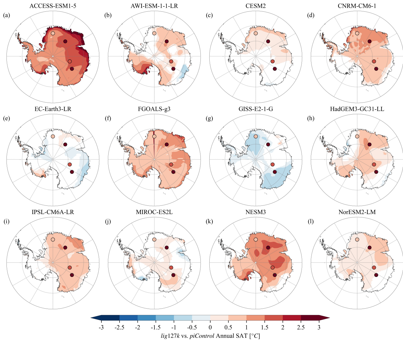
Figure 5. Differences in annual SAT between lig127k and piControl simulations. Paleo proxies in each subfigure are from Fig. 1a. We only show differences-temperature anomalies that are significant at 5% level based on the student's t-test with Benjamini-Hochberg Procedure controlling false discovery rates (Benjamini and Hochberg, 1995).
