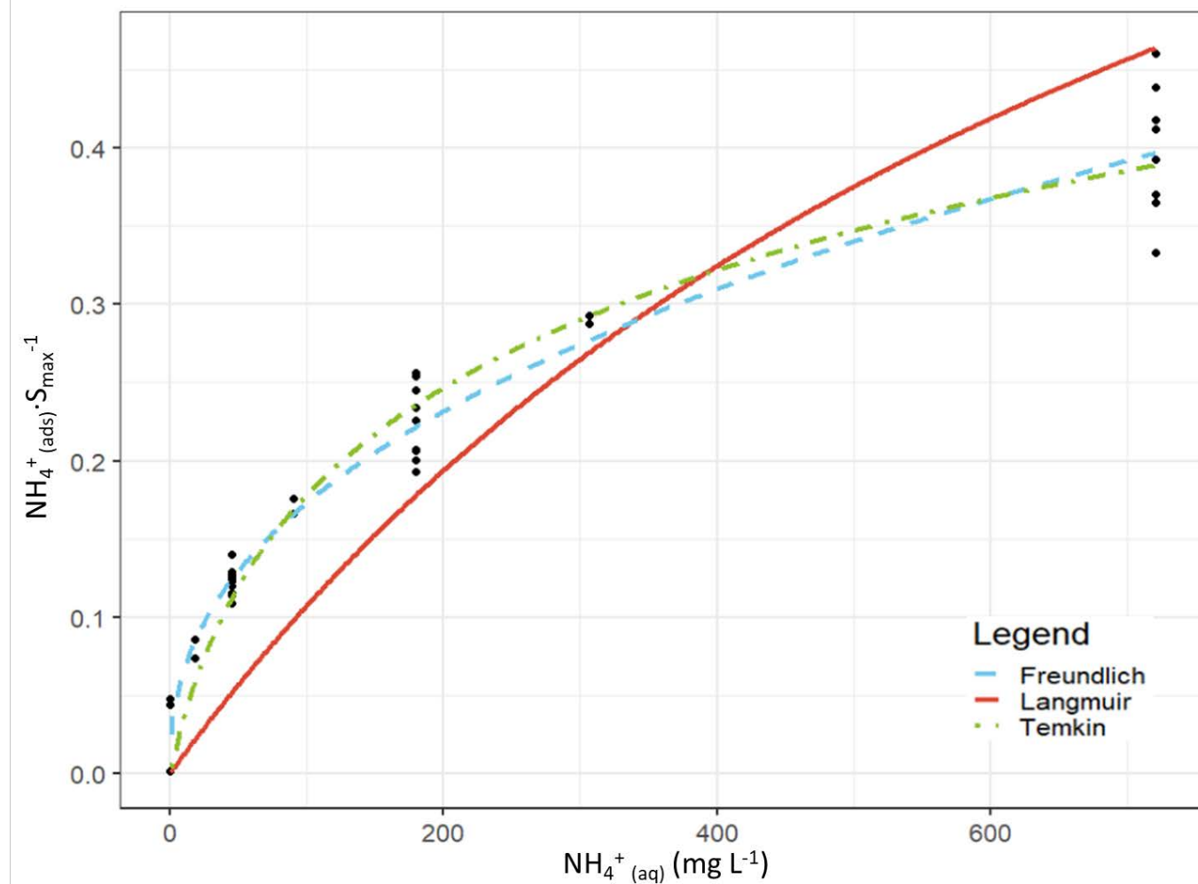
170 Figure 2: Curve-fitting comparison between the Langmuir (red, solid), Freundlich (blue, -- --), and Temkin (green, · - · -) equations. The curves are plotted using the experimental data from all eight soil adsorption experiments, but only using the extraction solutions of \leq 40 mM for fitting, the y-axis is normalized to the maximum adsorption achieved during each experiment. The Toth equation could not be fit to the experimental data under these conditions.
