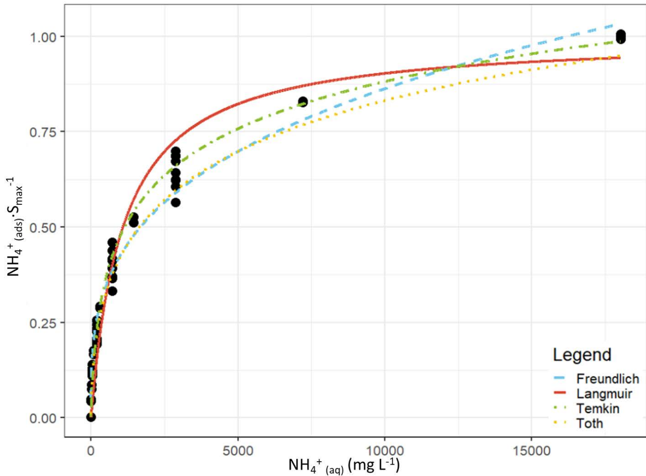
165 Figure 1: Curve-fitting comparison between the Langmuir (red, solid), Freundlich (blue, ---), Temkin (green, - · - ·), and Toth (orange, · · ·) equations. The curves are plotted using the experimental data from all eight soil adsorption experiments, the y-axis is normalized to the maximum adsorption achieved during each experiment.
