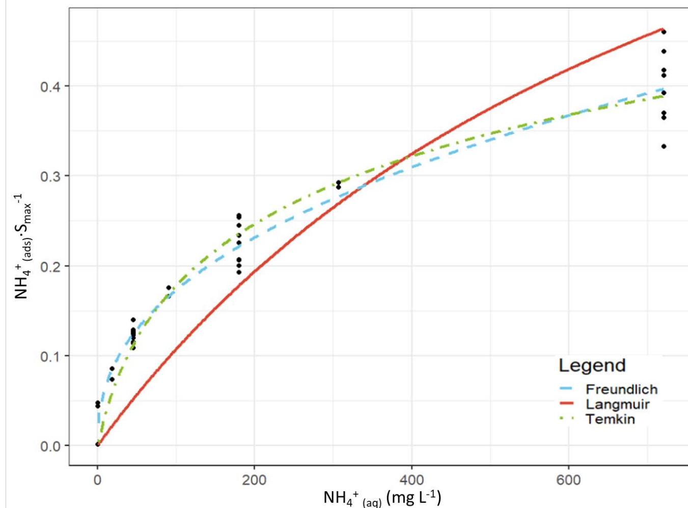
170 Figure 2: Curve-fitting comparison between the Langmuir (red, solid), Freundlich (blue, ---), and Temkin (green, ·-·-) equations. The curves are plotted using the experimental data from all eight soil adsorption experiments, but only using the extraction solutions of \leq 40 mM for fitting, the y-axis is normalized to the maximum adsorption achieved during each experiment. The Toth equation could not be fit to the experimental data under these conditions.
