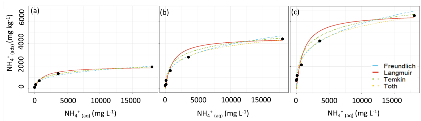
190 Figure 3: Curve-fitting comparison between the unfitted Langmuir (red, solid), Freundlich (blue, ---), Temkin (green, ·-·-), and Toth (orange, ···) equations using the fitting parameters from Table 3 applied to the test set of the a) Low CEC, b) Moderate CEC, c) High CEC samples (method ii)
