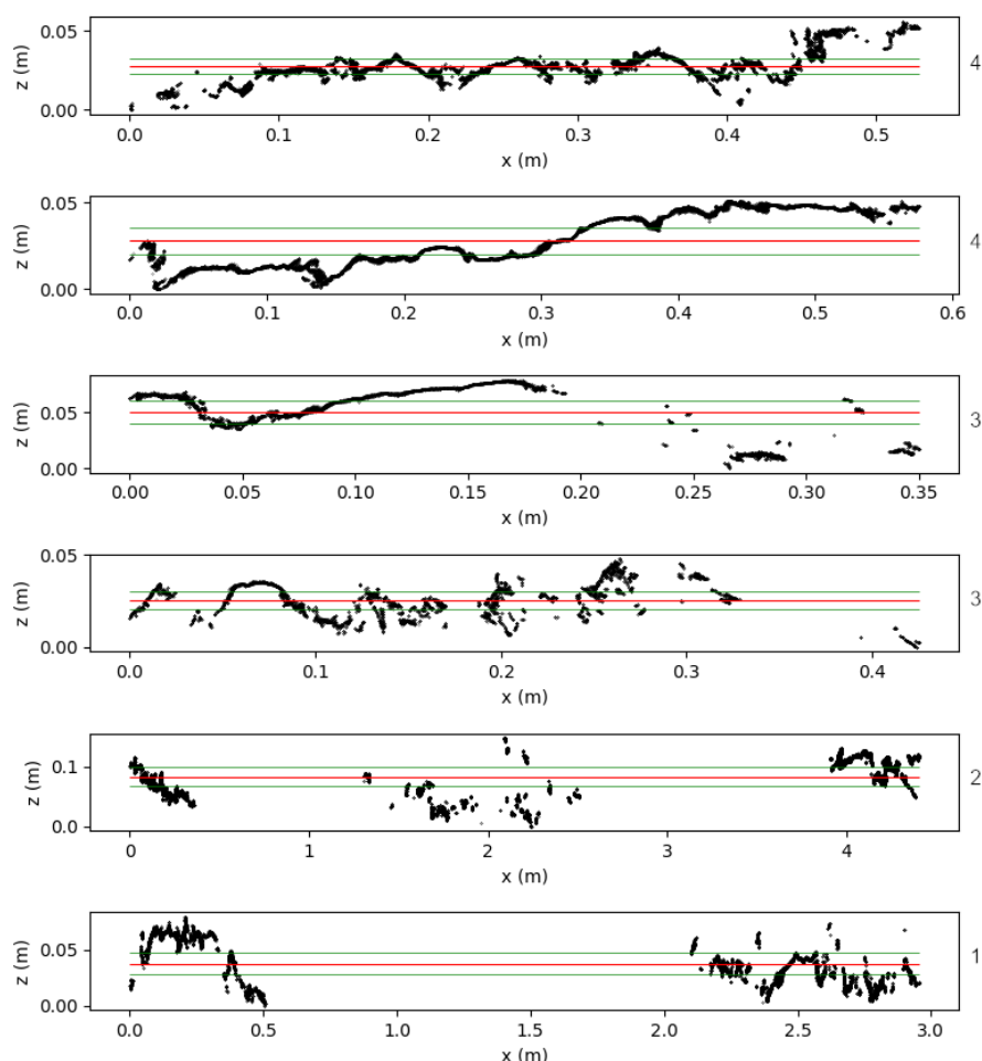
Figure 10: Plotted vertical coordinates of every 40th cross-section of the final cross-sectioned reconstruction. The topmost graph is from the upstream end of the reconstruction and lowest on the other hand from the downstream end and rest are from between in the same order. The corresponding segments are marked on the right side of each graph. Mean height value (z-coordinate) is marked with red and standard deviation of height with green.
