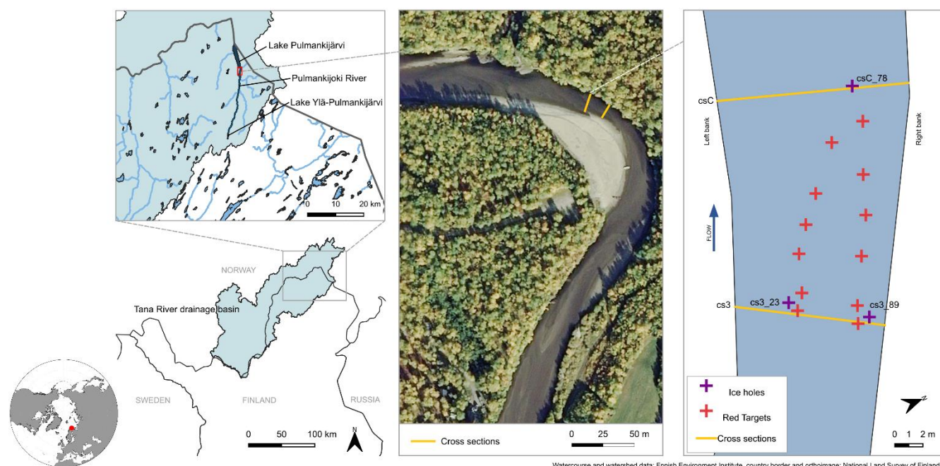
Figure 2: Pulmankijoki River study site located in northern Finland. Exact study site is located in a meander bend and the studied area covers roughly 16 m long area between two cross-sections (marked with yellow). Ice holes and targets used in the reconstruction of a digital elevation model of the ice underside are marked with purple and red in the rightmost map. The ROV was placed in water ice hole cs3_89 in cross-section cs3.
