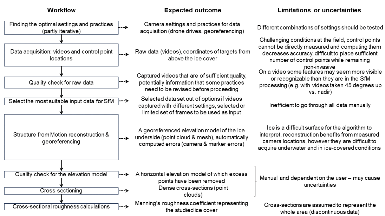
Figure 11: Overall workflow summarizing the steps required for elevation model reconstruction and calculating Manning's coefficient. Height of the frames outlining workflow steps show the relative weight of each step (considering how time-consuming and computationally demanding they were).
