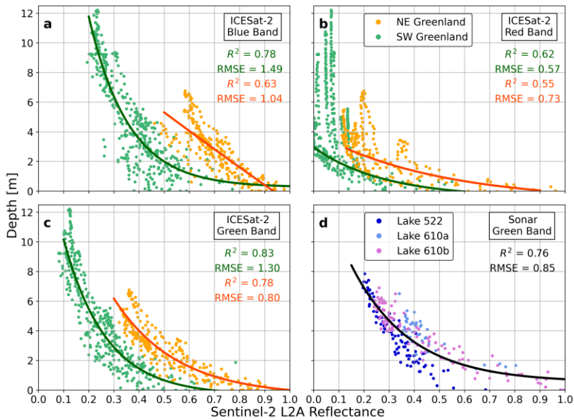
Figure 5: SGL d Depth versus reflectance plots for ICESat-2 depths (a)-(c) and sonar depths (d) against their corresponding Sentinel-2 L2A reflectance values. For (a)-(c), data gathered from ICESat-2 tracks in Southwest Greenland are represented by green points and data from Northeast Greenland are represented by orange points. For (d), each color represents a different lake from which the
