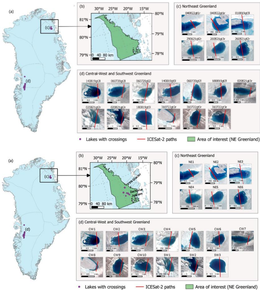
145 Figure 1: (a) An overview of Greenland, showing the locations of the supraglacial lakes with ICESat-2 crossings used in this study (purple points) labeled by (c) and (d), which are shown in further detail in the respective subimage. The gray lines represent Greenland's basin boundaries, produced by Rignot et al. (2011). (b) A closer view of Northeast Greenland, with the region over which an interannual analysis will was be produced. (c) and (d) show the ICESat-2 track paths (red) for the lakes marked in (a) for 150 Central-West/Southwest Greenland and Northeast Greenland, respectively. Each lake is labeled with its acquisition date and ICESat-2 beam ID and is represented visually with the Sentinel-2 image closest to the acquisition (listed in Table A1).
