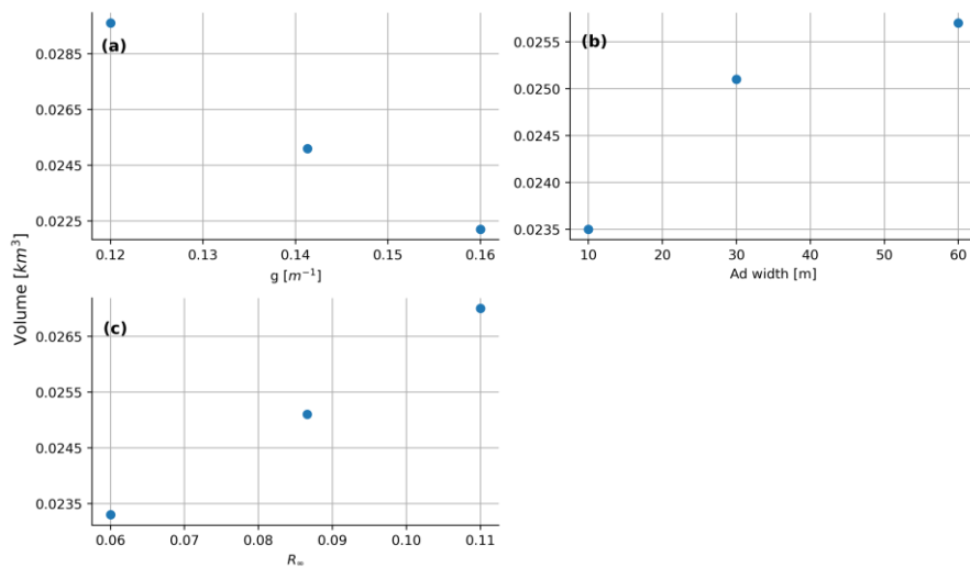
Figure B43: The sensitivity of (a) the two-way attenuation coefficient, g , (b) the width of ice around the lake considered in calculating the lake bed albedo, A_d width [m], and (c) the reflectance of optically deep water, R_{\infty} . The estimated lake volume [km 3 ] for Lake 562 is given for the different variable inputs. The central value for each parameter was used in the method comparison in Sect. 3.3.
