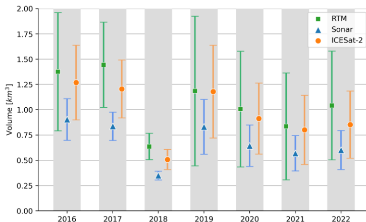
Figure 7: The total lake volume [km 3 ] over Northeast Greenland (area defined in Fig. 1(b)) for the date of peak melt area determined in Lutz et al. (2023) over the 2016 to 2022 melt seasons. The estimates from the sonar equation, ICESat-2 equation, and the RTM method are shown for each melt season, along with their estimated uncertainties.
