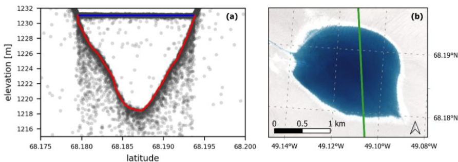
Figure 2: An example SGL in southwest Greenland captured on 18 August 2019. (a) Plotted ICESat-2 ATL03 data showing the lake surface (blue) and lake bed profile (red), created using the picking tool by Fricker et al. (2021). (b) the Sentinel-2 image from the previous day (17 August 2019), showing the ICESat-2 path crossing the lake (green).
