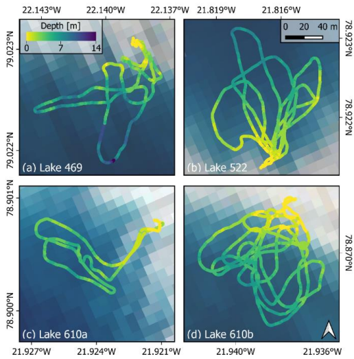
210 Figure 4: The sonar tracks captured over the four SGLs acquired in situ with a remote controlled boat. The sonar data for Lake 610a were acquired on 4 July 2022 and the other three lakes on 9 July 2022. The backgrounds are Sentinel-2 L2A RGB images from one day before the sonar acquisition date, i.e. 3 July 2022 and 8 July 2022.
