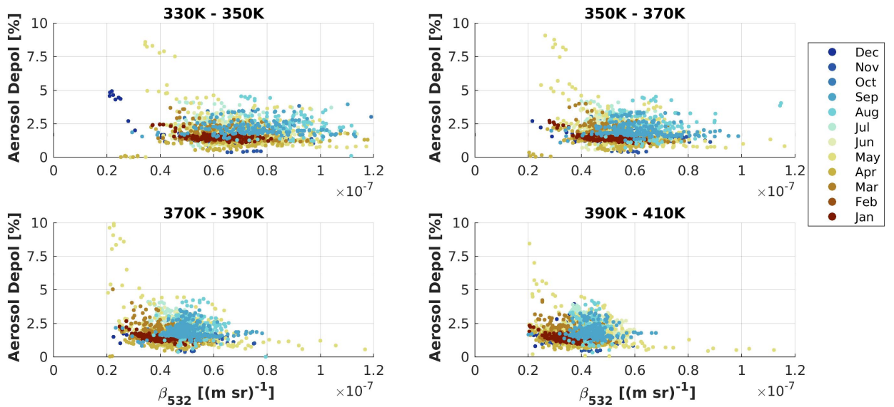
Figure 8. Dependency of \beta_{532} and \delta_{532} for the four selected altitudes in the lower stratosphere plot changed
