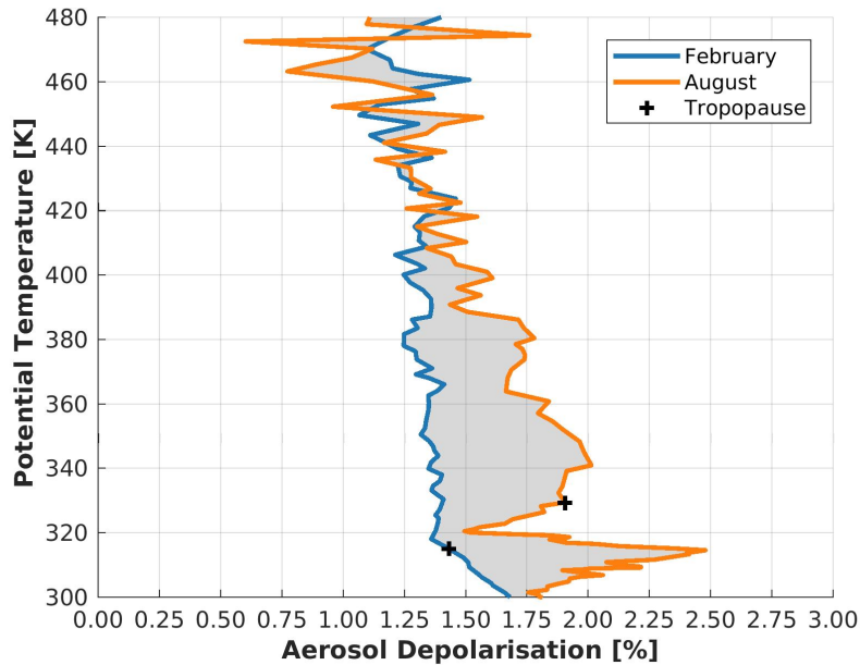
Figure 9. Mean aerosol depolarisation, \delta_{532} , for the two exemplary months February and August. The grey shaded area shows the difference between both months Plot changed
