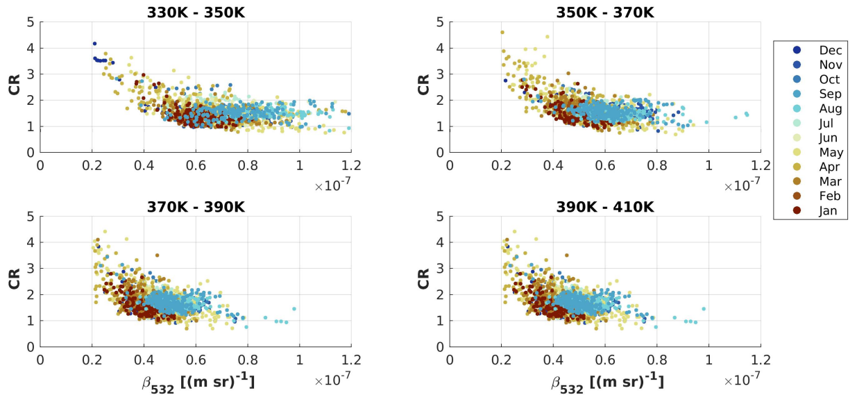
Figure 7. Dependency of CR and \beta_{532} for four selected height intervals of the lower stratosphere plot changed
