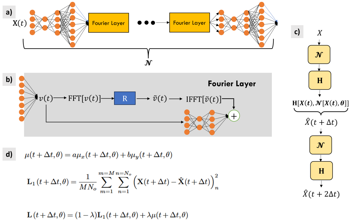
Figure 3. A schematic of the OceanNet model with input image X(t) . (a) The Fourier Neural Operator, \mathcal{N} . Prior to entering the Fourier Layers, the input image is fed through a multilayer perceptron consisting of two convolutions. The output of each of the Fourier layers is activated with the Gaussian Error Linear Units function. Following the last Fourier layer, the data is fed through two more convolutions to preserve the dimensions of the final output. (b) The Fourier Layer. A Fourier transform is performed on v(t) , the higher-dimensional representation of the input image, followed by a linear operation, R , to reduce the highest Fourier modes to zero, resulting in \tilde{v}(t) . An inverse Fourier transform brings \tilde{v}(t) back to its original space. The resulting tensor is then concatenated with the input to the Fourier layer, to which a 2D convolution has been applied. OceanNet contains four Fourier Layers (c) the two-time-step scheme with the numerical integration operator, H (d) The point-wise loss function used, constructed by the spectral regularizer \mu and MSE, L_1 , for M samples and applied to all N_o ocean points. The loss function is discussed in greater detail in Sect. 2.4.1
