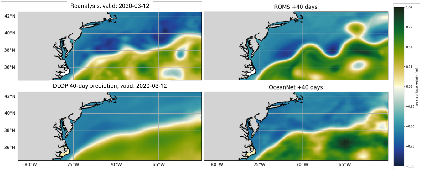
Figure 11. Prediction performance of a DLOP, ROMS, and OceanNet on the GSM region at 40 days. The SSH field 40 days after model initialization of "Run-57," referring to the 57th ensemble member (randomly selected) 2020-02-01 described in Sect. 3, for (Top-left) the reanalysis dataset, (Top-right) ROMS, (Bottom-left) DLOP, and (Bottom-right) OceanNet.
