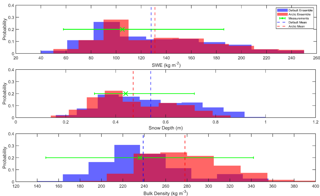
295 Figure 3: Distribution of simulated SWE (kg m -2 ), snow depth (m) and bulk density (kg m -3 ) by default and Arctic SVS2-Crocus, 1991-2023, calculated at the time of snow course measurements (around peak SWE accumulation). Dashed vertical lines represent mean values of each ensemble. Green crosses (mean) and error bars (range) represent the range of snow measurements taken around peak SWE.
