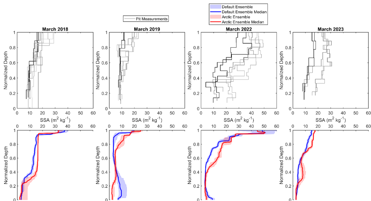
Figure 7: Comparison of measured and simulated vertical profiles of SSA ( \text{m}^2 \text{kg}^{-1} , median, interquartile range) by default and Arctic SVS2-Crocus from the March 2018, March 2019, March 2022 and March 2023 winter field campaigns. Black and grey lines indicate different pit profiles.
