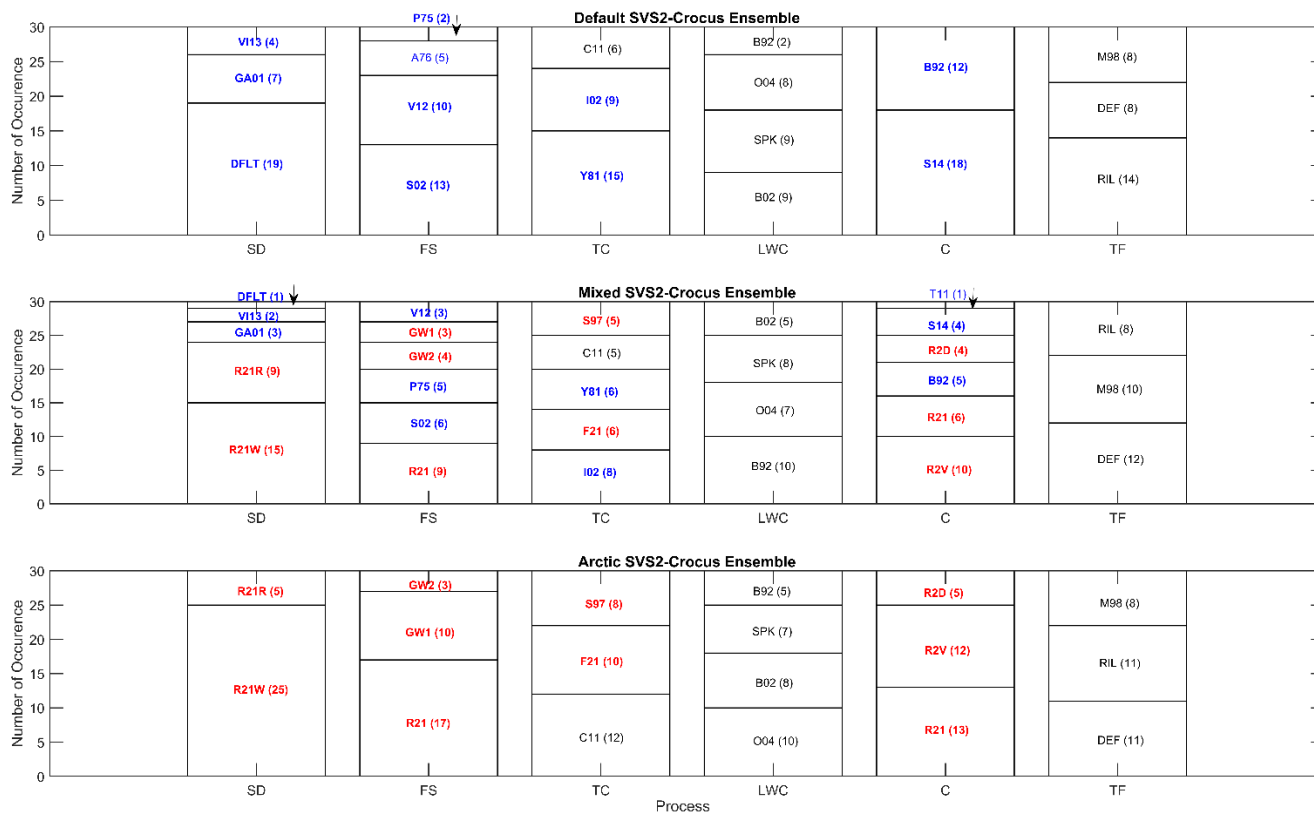
440 Figure 9: Number of occurrences of each parameterisation in the top 30 members with the lowest CRPS scores for simulation of density by default, mixed and Arctic SVS2-Crocus. Blue indicates members of the default ensemble; red indicates members of the Arctic ensemble and black indicates members of both. Numbers in brackets represent number of occurrence. SD: Snowdrift, FS: Falling Snow, TC: Thermal Conductivity, LWC: Liquid Water Content, C: Compaction, TF: Turbulent Flux. For specific combinations of parameterisations within each ensemble member see Appendix C.
