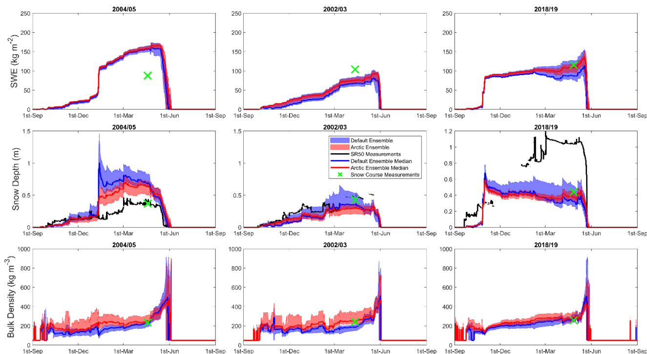
Figure 2: Evolution of simulated SWE (kg m -2 ), snow depth (m) and bulk density (kg m -3 ) during selected snow seasons: overestimation of model SWE and snow depth (2004/05), good model agreement (2002/03) and model underestimation (2018/19) for default (blue ensemble, with blue median) and Arctic SVS2-Crocus (red ensemble, with red median). Green crosses represent the average of manual snow course measurements around peak SWE accumulation. Hourly averaged SR50 measurements are represented by the black line.
