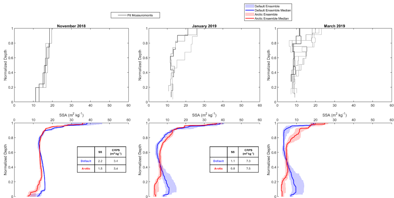
340 Figure 5: Comparison of measured and simulated vertical profiles of SSA ( \text{m}^2 \text{kg}^{-1} , median, interquartile range) by default and Arctic SVS2-Crocus from the November 2018, January 2019 and March 2019 winter field campaigns. Black and grey lines indicate different pit profiles. Tables contain statistical scores of SS and CRPS for the whole November 2018 and January 2019 profiles.
