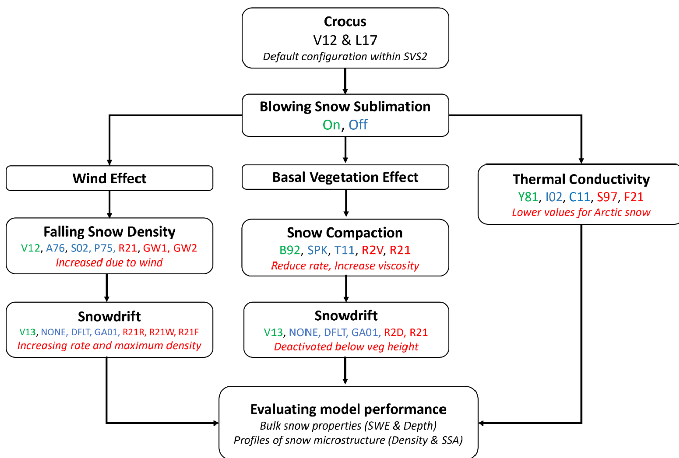
Figure 1: Model ensemble schematic showing the modified SVS2-Crocus schemes for Arctic application. Green initials illustrate default parameterisations, blue initials illustrate other existing parameterisations and red illustrate implemented Arctic-focused parameterisations. For a description of both green and blue options, see Lafaysse et al. (2017) and Vionnet et al. (2012). The options in red are described in the main text. A table describing the acronyms can be found in Appendix A.
