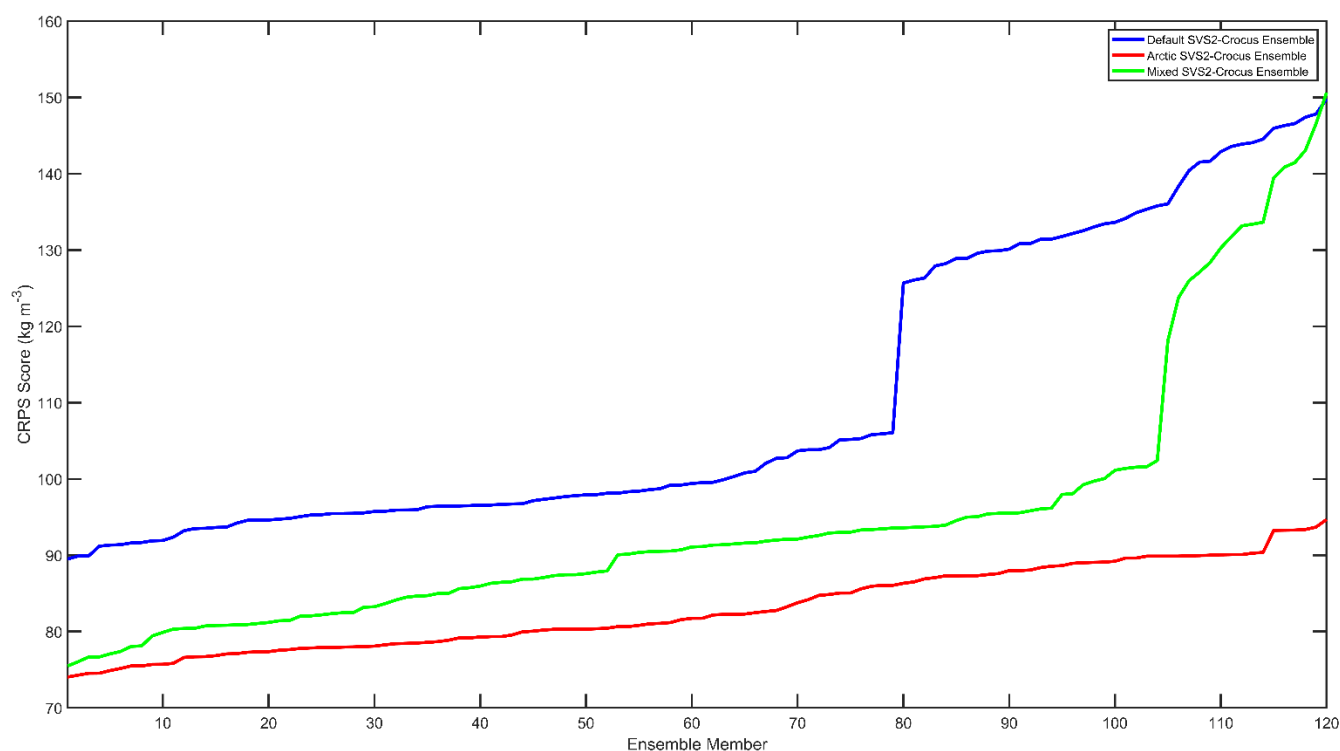
415 Figure 8: Comparison of ranked CRPS scores for all 120 members of the default, Arctic and mixed ensembles of SVS2-Crocus for the simulation of snow density ( \text{kg m}^{-3} ) averaged over the whole snowpack in March 2018, March 2019, March 2022 and March 2023.
