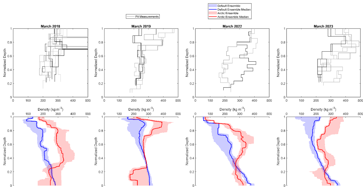
350 Figure 6: Comparison of measured and simulated vertical profiles of density ( \text{kg m}^{-3} , median, interquartile range) by default and Arctic SVS2-Crocus from the March 2018, March 2019, March 2022 and March 2023 winter field campaigns. Black and grey lines indicate different pit profiles.
