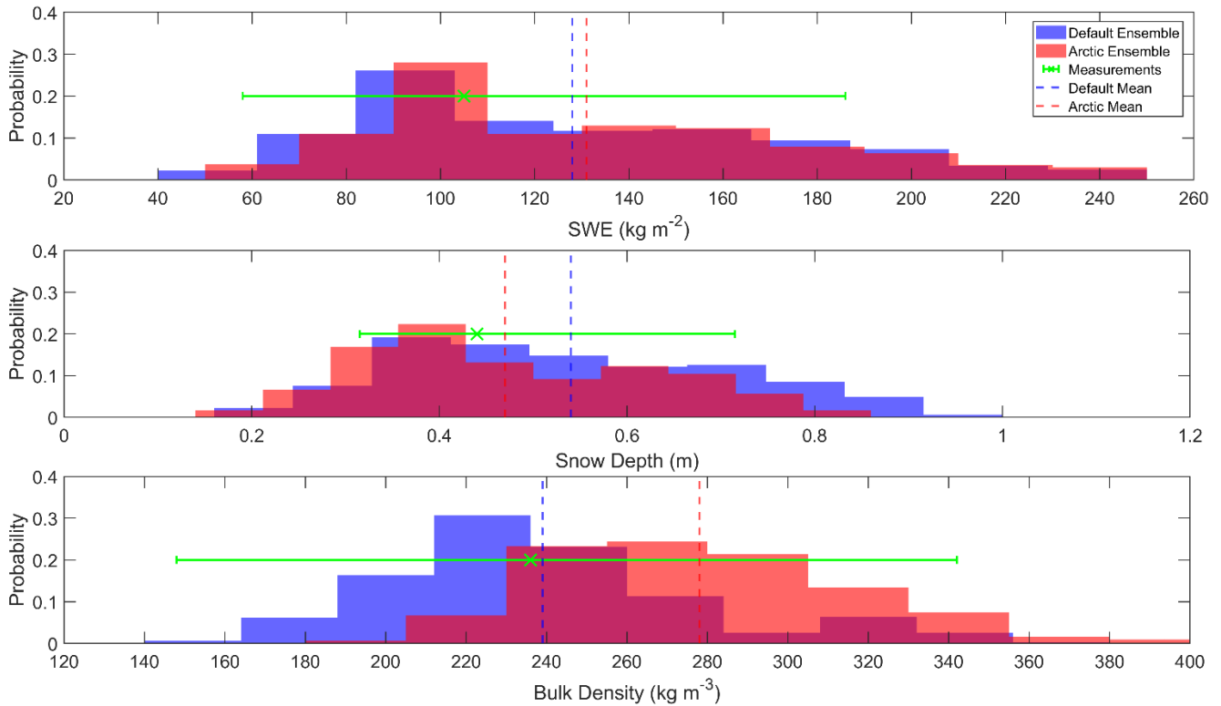
Figure 3: Distribution of simulated SWE (kg m -2 ), snow depth (m) and bulk density (kg m -3 ) by default and Arctic SVS2-Crocus, 1991-2023, calculated at the time of snow course measurements (around peak SWE accumulation). Dashed vertical lines represent mean values of each ensemble. Green crosses (mean) and error bars (range) represent the range of snow measurements taken around peak SWE.
