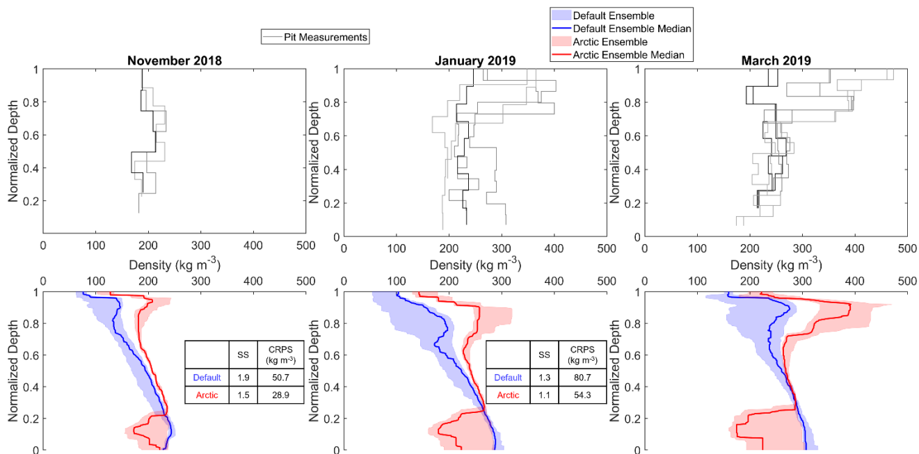
Figure 4: Comparison of measured and simulated vertical profiles of density ( \text{kg m}^{-3} , median, interquartile range) by default and Arctic SVS2-Crocus from the November 2018, January 2019 and March 2019 winter field campaigns. Black and grey lines indicate different pit profiles. Tables contain statistical scores of SS and CRPS for the whole November 2018 and January 2019 profiles.
