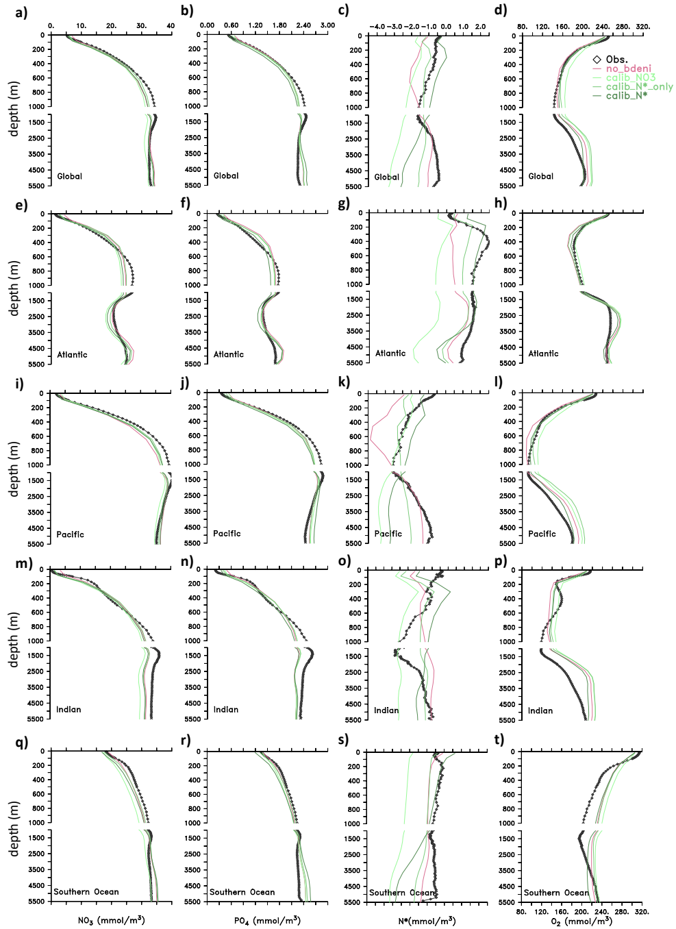
Figure 6. Vertical distributions of tracers ( \text{NO}_3^- , \text{PO}_4^{3-} , \text{N}^* , \text{O}_2 ) in the global ocean and the Atlantic, Pacific, Indian, Southern Oceans.
