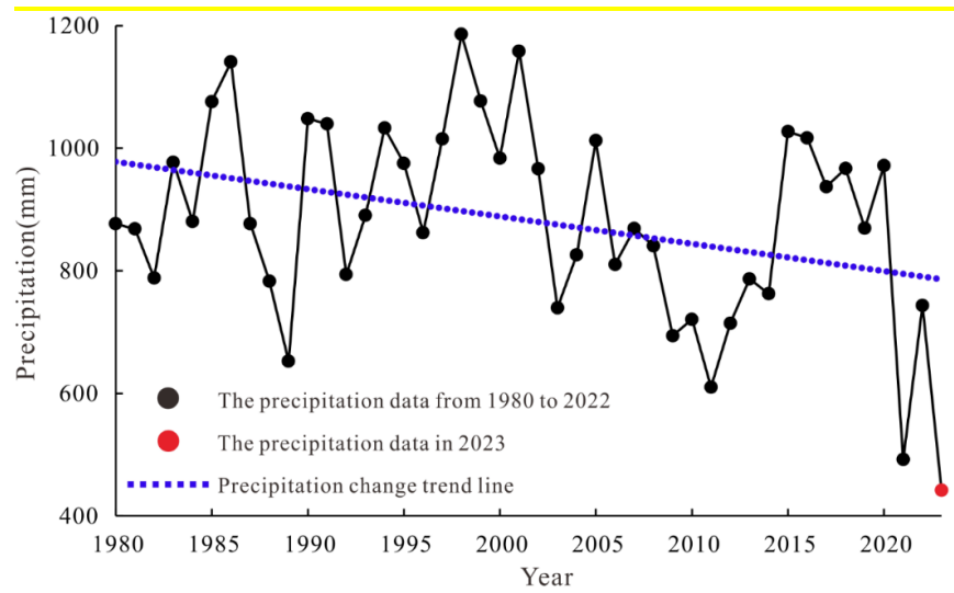
Figure 3 The precipitation changes in the study area from 1980 to 2023 (The precipitation data from 1980 to 2022 were collected from Yunnan Statistical Yearbook, and the precipitation data in 2023 were the measured data of Jinsha River Field Observation Station.).
