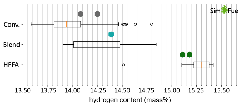
Figure 2. Hydrogen content of the fuels used during the ECLIF3 campaign compared to world average fuel data from the SimFuel platform. Both conventional Jet A-1 used during the campaign show a higher hydrogen content, the HEFA-SPK show a lower hydrogen content and the blend fuel an average hydrogen content compared to average fuels of the same type. The box in the plot extends from the first quartile to the third quartile of the data, with an orange line indicating the median. The whiskers extend from the box to the furthest data point that falls within 1.5 times the inter-quartile range. Any data points beyond the end of the whiskers are marked as empty circles, indicating outliers.
