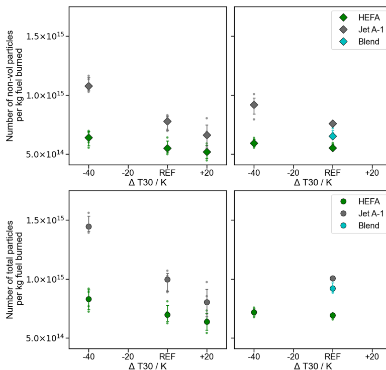
Figure 4. Emission index of non-volatile particle (top) and total particle number (bottom) with difference to a reference combustor inlet temperature (T30) in Kelvin for the different fuels probed during ECLIF3-1 (left) and ECLIF3-2 (right). The particle emission index decreases with increasing T30, with the largest decrease in emissions when using Jet A-1. The figure shows median values with upper and lower confidence intervals (75 %).
