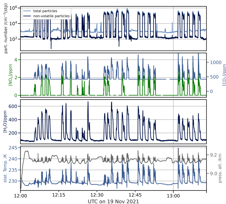
Figure 3. Timeline of the second emission flight during ECLIF3-2 on 19 November 2021 over the Atlantic. The top row shows the number concentration of total particles larger than 5 nm (light blue) and non-volatile particles larger than 14 nm (dark blue) at standard temperature and pressure, the second panel shows trace gas concentrations of CO 2 (blue) and NO y (green), the third row shows the timeline of the water vapor concentration and the bottom panel shows the ambient temperature and the altitude of the research aircraft. During the peak sequences of the timelines the Falcon was located within the plume about 100-200m behind the A350.
