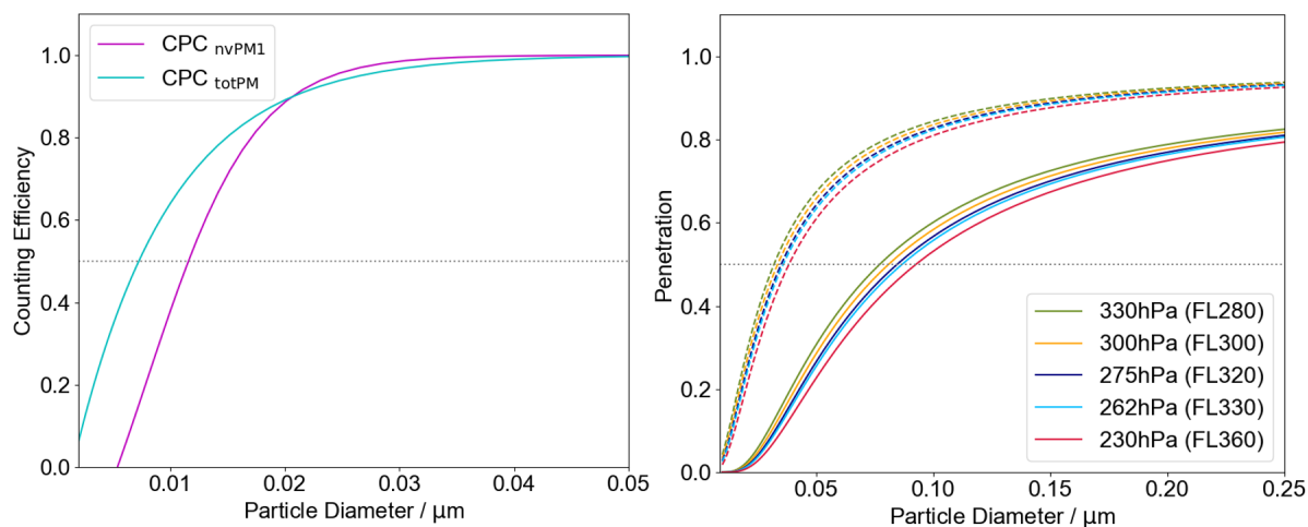
Figure A2. Counting efficiency at 300hPa of the CPC measuring nvPM and total particles (left). Penetration with particle size at different pressures using CPC_{nvPM2} (dashed line) with one or CPC_{nvPM3} (solid line) with three diffusion screen separators (right). Cut-off diameters D_{50} are reached at 50 % counting efficiency (dotted grey).
