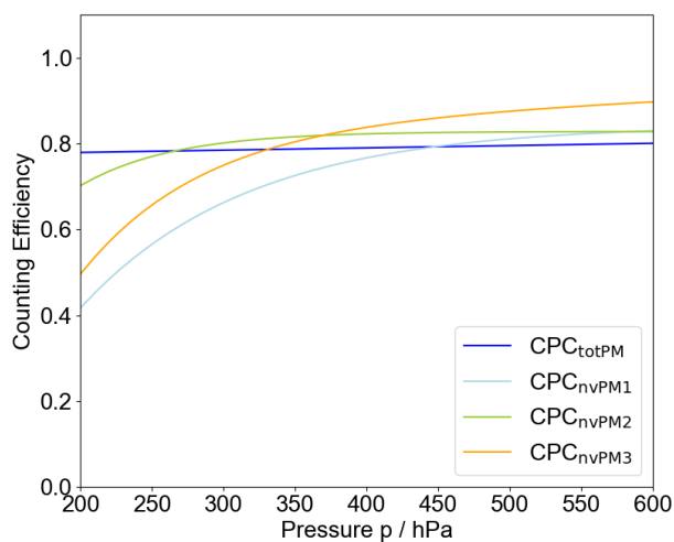
Figure A1. Counting efficiency at low pressure derived from laboratory measurements. CPC used for total particle measurements is shown in blue, CPC measuring total nvPM in light blue. CPCs used with diffusion screen separators during the flight measurements are depicted in green (1 diffusion screen) and yellow (3 diffusion screens). Diffusion screens were removed for laboratory measurements. Calibrations have been captured with inlet lines to also account for inlet line losses.
