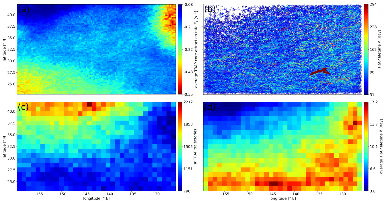
Figure 4. Distribution of TRAP characteristics over the domain and in within the period 2000-2019. (a) TRAP core attraction strength s_1 averaged over 20 years and all instances within bins of 0.25^\circ \times 0.25^\circ size. Red colours indicate high attraction. (b) Trajectories of long-living TRAPs with lifetimes \Lambda > 30 days. Trajectories are coloured by the associated TRAP lifetime \Lambda , using the respective colour scale on the right. The most persistent TRAP is indicated by a thick line. (c) Number of identified TRAP trajectories that pass through histogram bins of 1^\circ \times 1^\circ size. (d) Average lifetime \bar{\Lambda} of TRAP trajectories passing through each bin.
