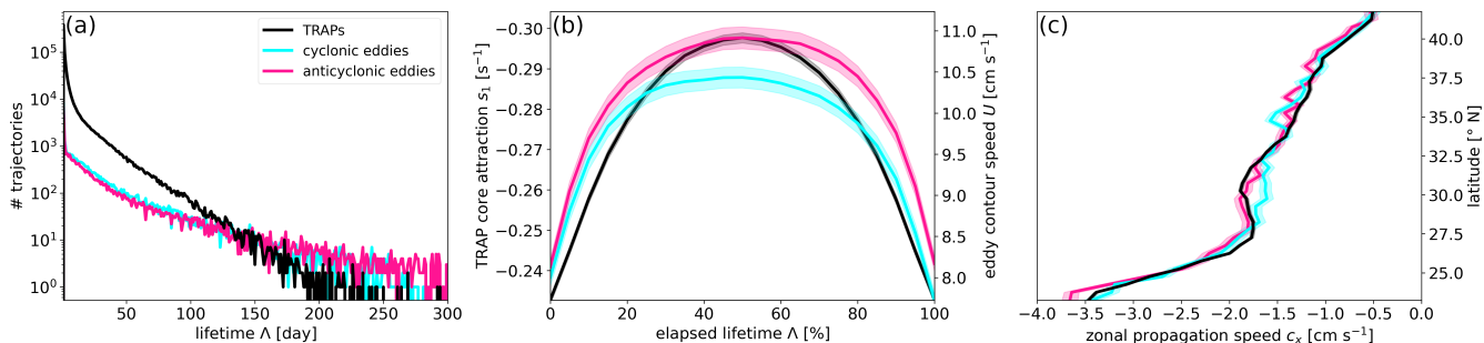
Figure 5. Comparisons between TRAPs and mesoscale eddies. (a) Distribution of lifetime \Lambda over all TRAP trajectories, cyclonic and anticyclonic eddy trajectories in the domain. The For clarity, we cut off the distributions of eddy lifetimes are cut-off at 300 days for clarity. (b) Evolution of attraction rate s_1 over TRAP lifetime and evolution of contour speed U over eddy lifetime for phenomena with lifetimes \Lambda > 30 days. (c) Latitudinal dependence of zonal propagation speed c_x for 2,951,028 TRAP, 604,296 cyclonic and 608,650 anticyclonic eddy instances. Lines in (b) and (c) indicate bin means, shaded bands their errors w.r.t. a confidence level of 95 %. Mesoscale eddies as detected by AVISO+ et al. (2022).
