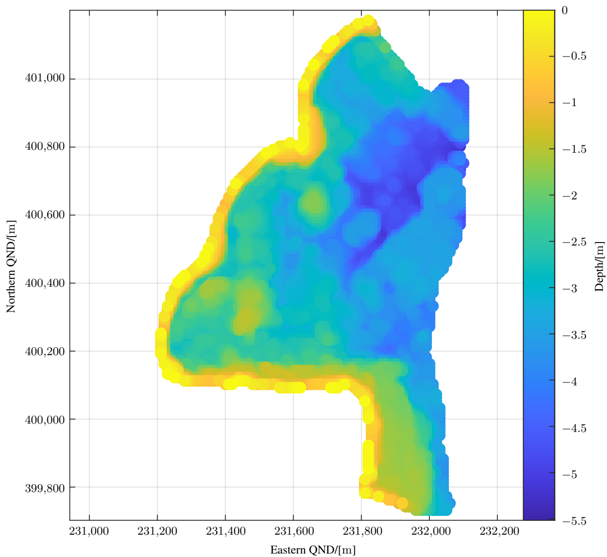
Figure A1. Bathymetry measurements during survey off Katara beaches. Not covered areas where augmented with remote sensing published separately Lawen et al. (2022).
