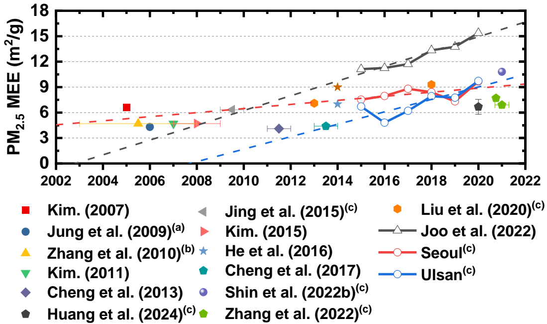
410 Figure 7: Comparison of PM 2.5 mass extinction efficiency (MEE) values from previous studies in Northeast Asia. (a) Estimated by single scattering albedo of 0.8, according to the literature. (b) The mass ratio of PM 2.5 to PM 10 was set to 0.56, and relative humidity was set to 40%, according to the literature. (c) Studies using wavelengths other than 550 nm.
