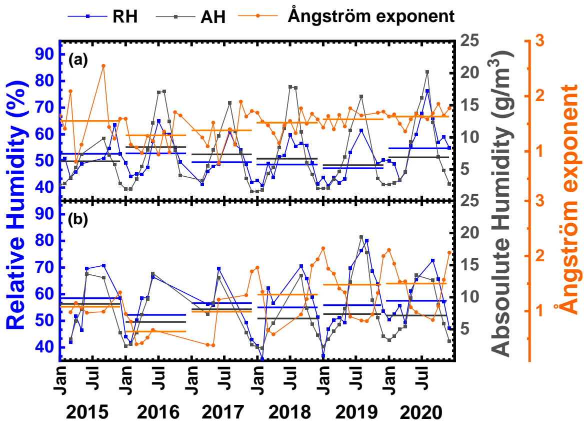
360 Figure 4: Yearly and Monthly average Ångström exponent, relative and absolute humidity in (a) Seoul and (b) Ulsan.
