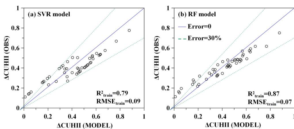
Fig. R5 The performance of the SVR model (a) and RF model (b) in predicting the \Delta CUHII .
