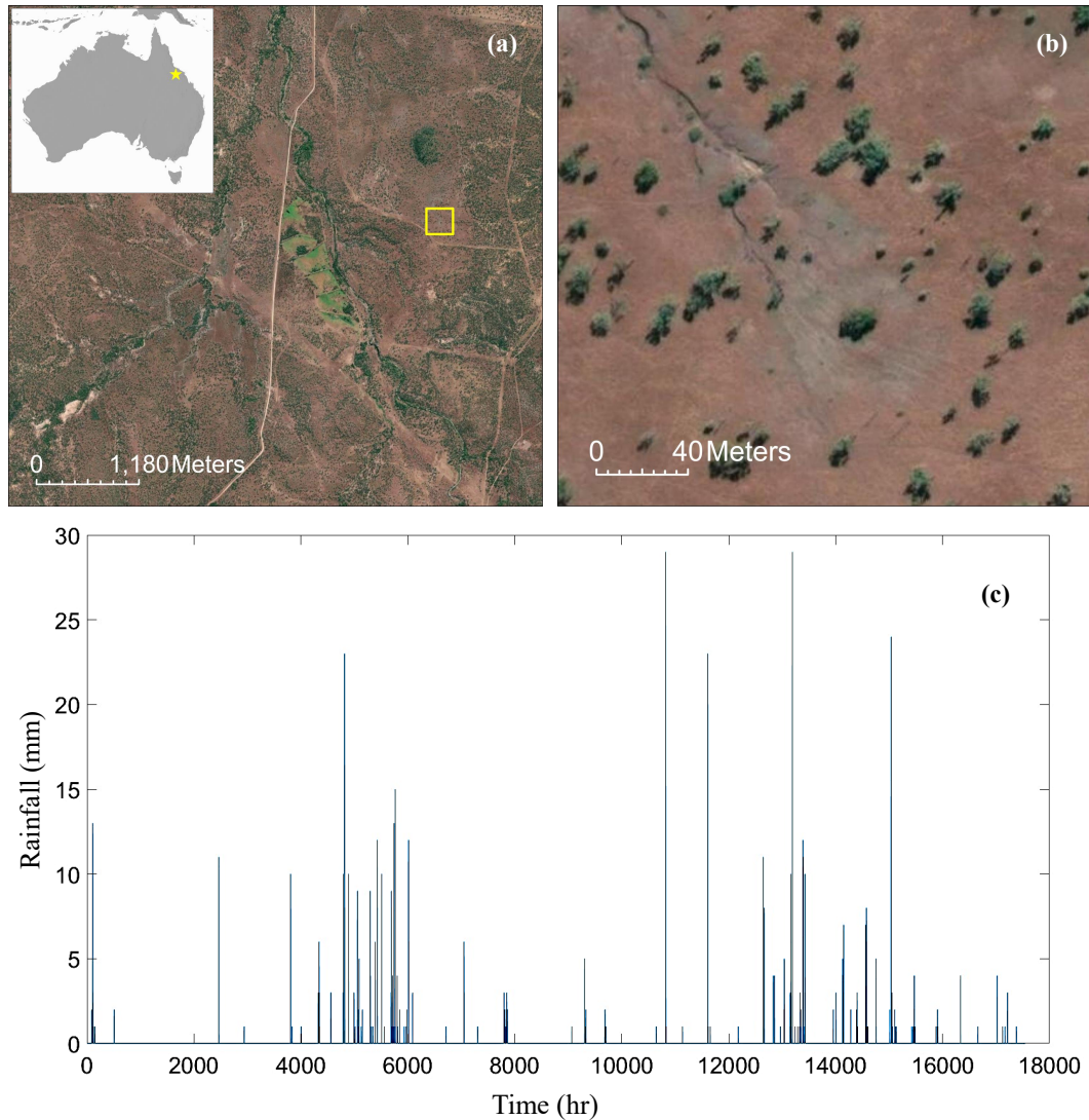
Figure 3. Study site information (a) Satellite image of the Bowen Basin, with the yellow box highlighting the study location , Inset shows the location of the Bowen basin (yellow star) in Australia. (b) Magnified (zoomed-in) view of the study region (c) Hourly rainfall data between July 2019-2021, pluviometer reading , (eSource: Basemap and data provided by Esri and its Community Map contributors. Pluviometer reading from Ernest Creek Pluvio of Burdekin basin, Queensland (WMIP), between the dates 1 st July 2019 – 2021 ) 2019 DEM of the study area, (d) 2021 DEM of the study area.
