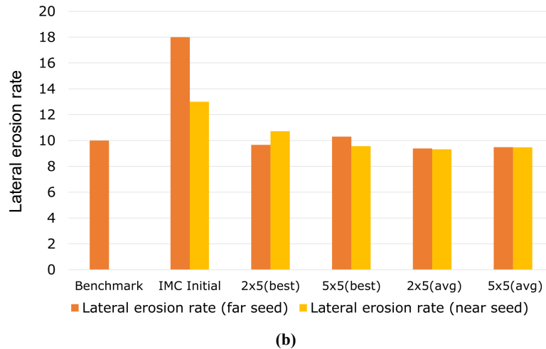
Figure 7. Estimating known optimal-numerical values ( Benchmark ) of CL parameters from their deliberately perturbed versions (a) Estimation of Max Erode Limit Max erode limit parameter (b) Estimation of Lateral Erosion Rate Lateral erosion rate parameter. Actual Benchmark refers to the “known optimal” CL parameter value and IMC initial is the perturbed version of the same, from where the IMC starts calibrating. IMC is run at different lengths ( = round \times iteration ) repeatedly and the best and average (of three separate calibration runs/epochs) of estimated parameter values are presented.
