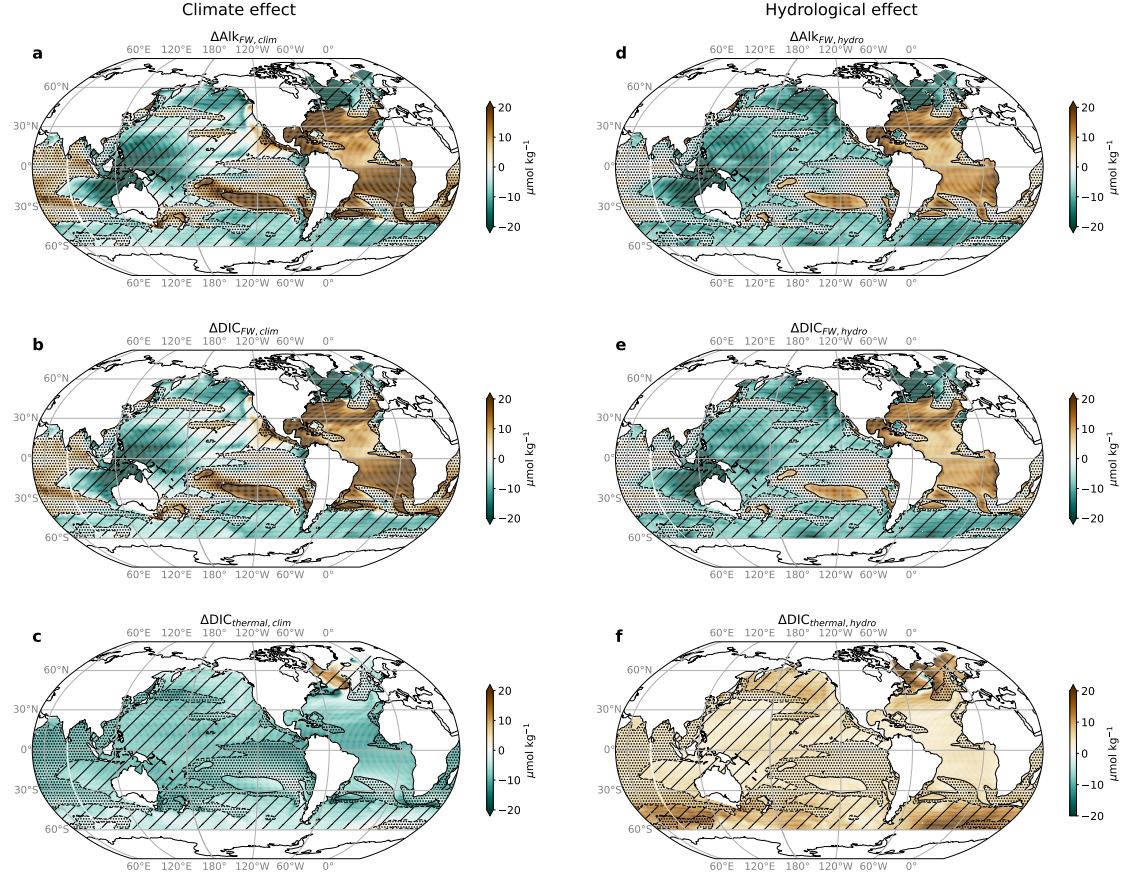
Figure A3. Thermal and freshwater components of DIC and Alkalinity changes. (a-c) change attributed to freshwater ( \Delta \text{Alk}_{FW,clim} = f_{FW,clim} \text{Alk}_{Fix-Clim} , \Delta \text{DIC}_{FW,clim} = f_{FW,clim} \text{DIC}_{Fix-Clim} ) and thermal ( \Delta \text{DIC}_{thermal,clim} = -7\Delta \text{SST}_{clim} ) components in climate effect; (d-f) change attributed to freshwater ( \Delta \text{Alk}_{FW,hydro} = f_{FW,hydro} \text{Alk}_{Fix-SSS} , \Delta \text{DIC}_{FW,hydro} = f_{FW,hydro} \text{DIC}_{Fix-SSS} ) and thermal ( \Delta \text{DIC}_{thermal,hydro} = -7\Delta \text{SST}_{hydro} ) components in hydrological effect.
