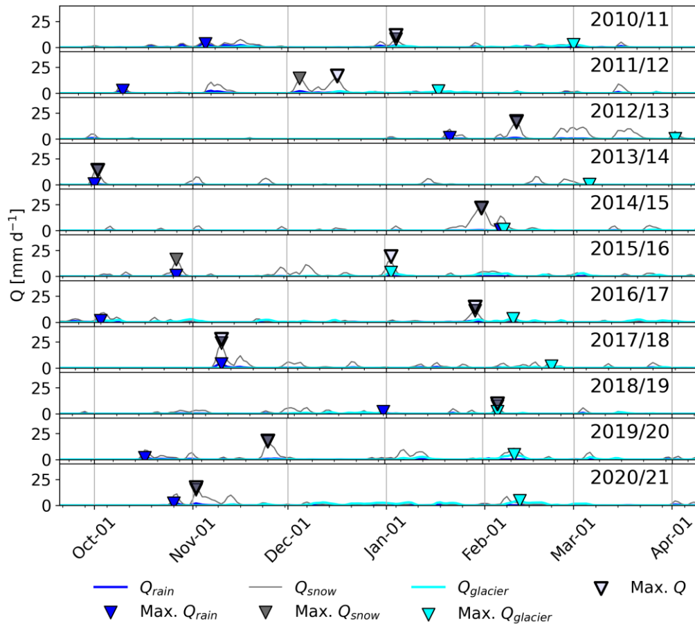
315 Figure 8: Daily rainfall runoff ( Q_{rain} ), snowmelt runoff ( Q_{snow} ), glacier melt runoff ( Q_{glacier} ) (lines) and maximal values of Q , Q_{rain} , Q_{snow} , Q_{glacier} (triangles) for individual water years.
