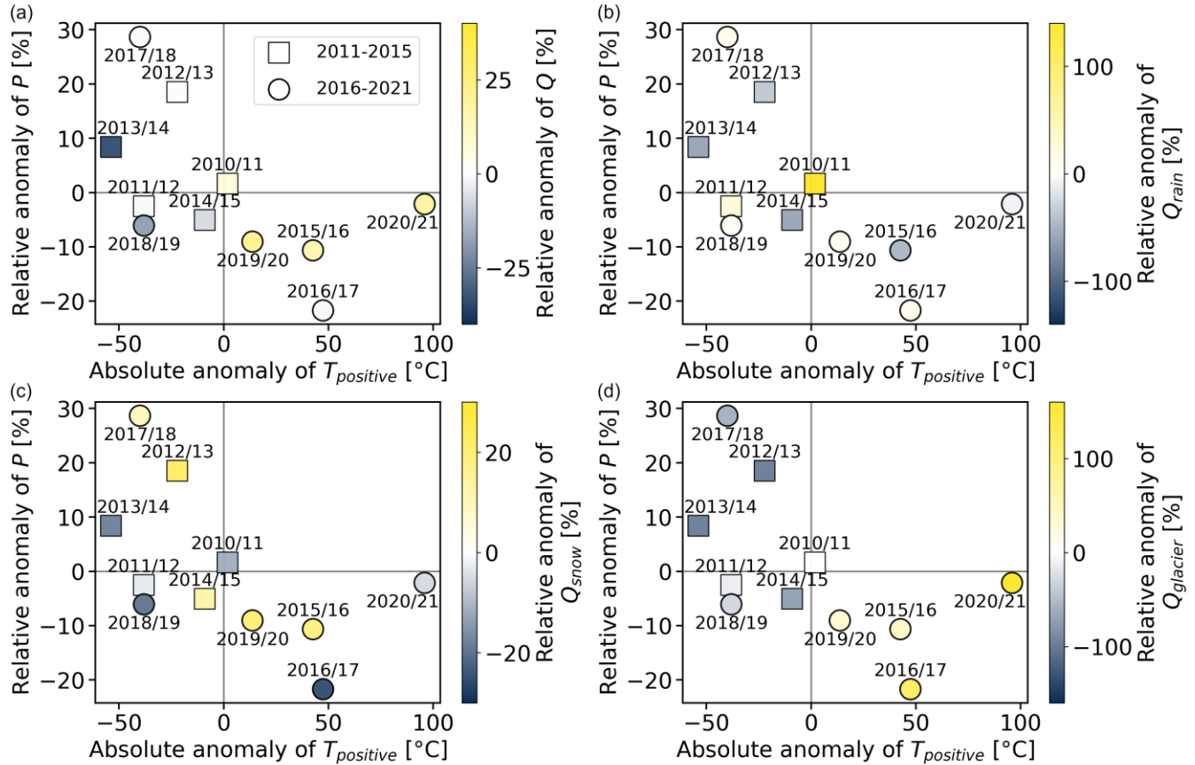
355 Figure 10: Relationship between absolute anomaly of T_{positive} , relative anomaly of P and relative anomaly of (a) mean annual runoff Q , (b) rainfall runoff Q_{rain} , (c) snowmelt runoff Q_{snow} and (d) glacier melt runoff Q_{glacier} for the years 2010/11–2014/15 (squares) and 2015/16–2020/21 (circles). Note that colour map ranges differ across panels.
