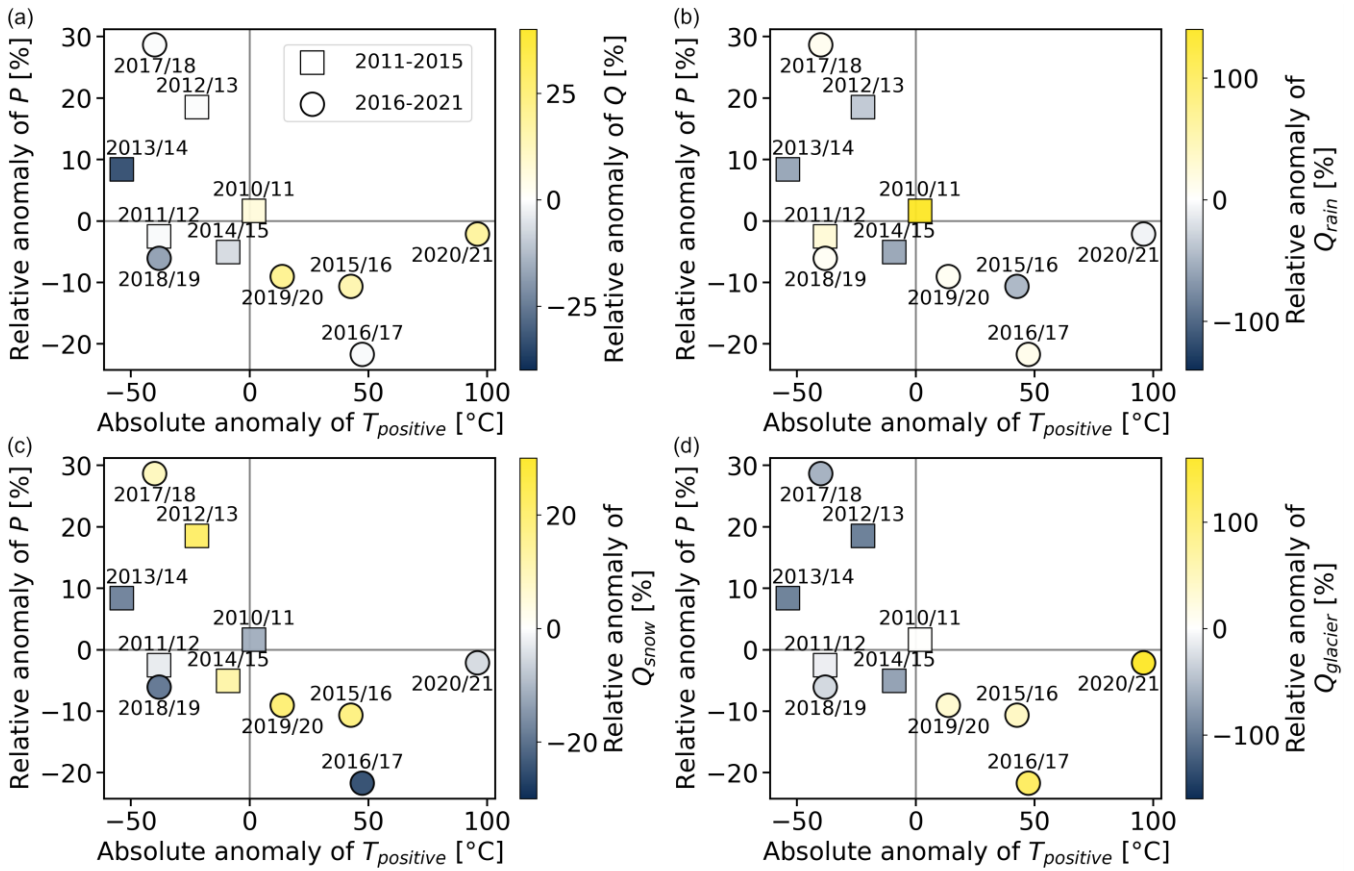
Figure 10: Relationship between absolute anomaly of T_{positive} , relative anomaly of P and relative anomaly of (a) mean annual runoff Q, (b) rainfall runoff Q_{rain} , (c) snowmelt runoff Q_{snow} and (d) glacier melt runoff Q_{glacier} for the years 2010/11–2014/15 (squares) and 2015/16–2020/21 (circles). Note that colour map ranges differ across panels.
