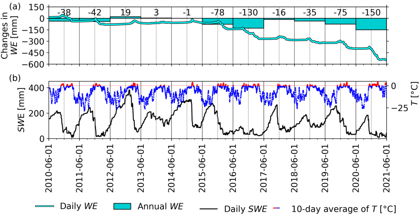
Figure 4: (a) Cumulative daily changes in glacier water equivalent (WE) from the start of the simulation (cyan line), and changes in WE in individual water years (bars). (b) Daily snow water equivalent SWE (black line) and 10-day moving average of air temperature (negative values in blue, positive values in red).
