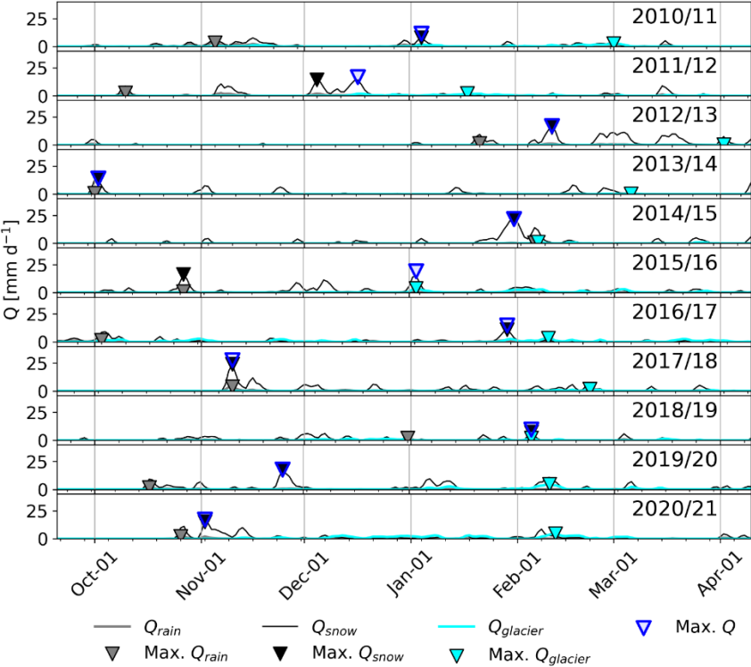
Figure 8: Daily rainfall runoff ( Q_{rain} ), snowmelt runoff ( Q_{snow} ), glacier melt runoff ( Q_{glacier} ) (lines) and maximal values of Q , Q_{rain} , Q_{snow} , Q_{glacier} (triangles) for individual water years.
