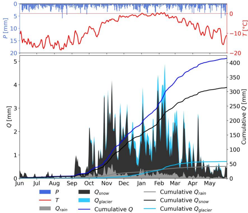
255 Figure 5: Mean daily precipitation ( P ; blue bars), 3-day moving average of air temperature ( T ; red line), mean daily rainfall runoff ( Q_{rain} ), snowmelt runoff ( Q_{snow} ), glacier melt runoff ( Q_{glacier} ; stacked areas, left axis), cumulative Q , Q_{rain} , Q_{snow} , and Q_{glacier} (lines, right axis) in the Triangular catchment for the period 2010/11–2020/21
