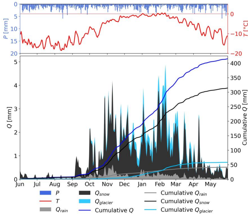
250 Figure 5: Mean daily precipitation ( P ; blue bars), 3-day moving average of air temperature ( T ; red line), mean daily rainfall runoff ( Q_{rain} ), snowmelt runoff ( Q_{snow} ), glacier melt runoff ( Q_{glacier} ; areas, left axis), cumulative Q , Q_{rain} , Q_{snow} , and Q_{glacier} (lines, right axis) in the Triangular catchment for the period 2010/11–2020/21
