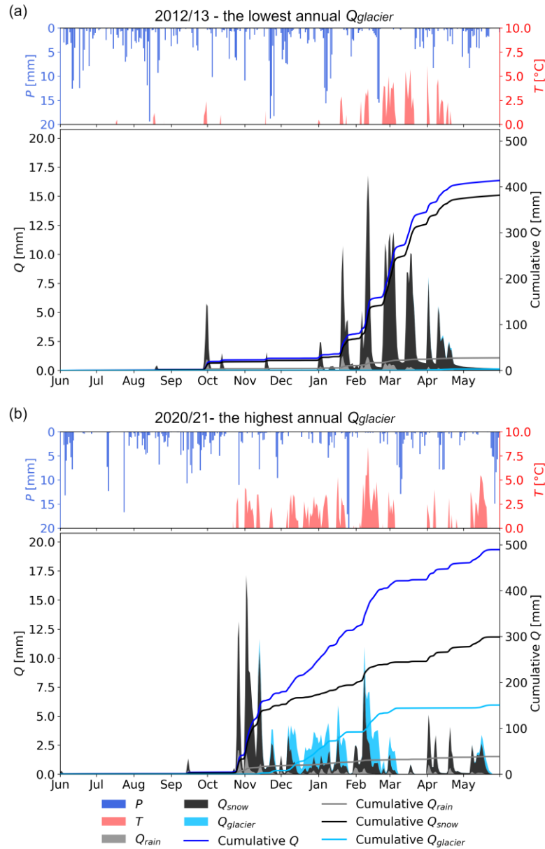
280 Figure 7: Contribution of rainfall runoff ( Q_{rain} ), snowmelt runoff ( Q_{snow} ), glacier melt runoff ( Q_{glacier} ) to total runoff ( Q ) during two selected years; (a) the year 2012/13 with the lowest annual glacier melt contribution and (b) the year 2020/21 with the highest glacier melt contribution.
