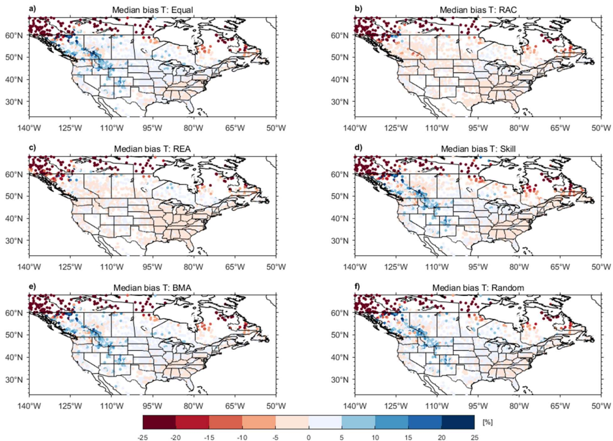
850 Figure S2. Similar to Figure 5, but bias is plotted as negative and positive values
