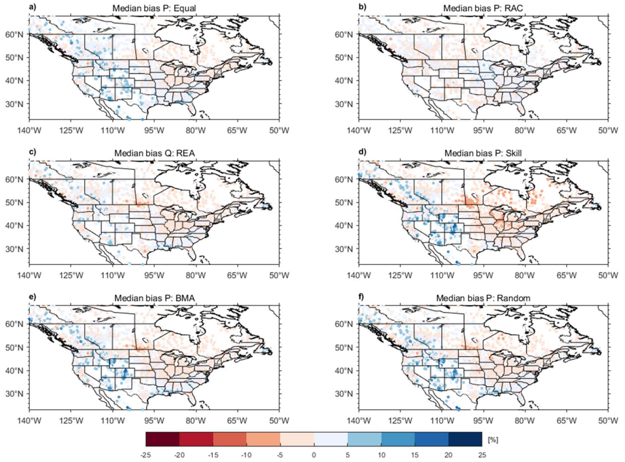
Figure S1: similar to fig 4 but median bias is plotted.
