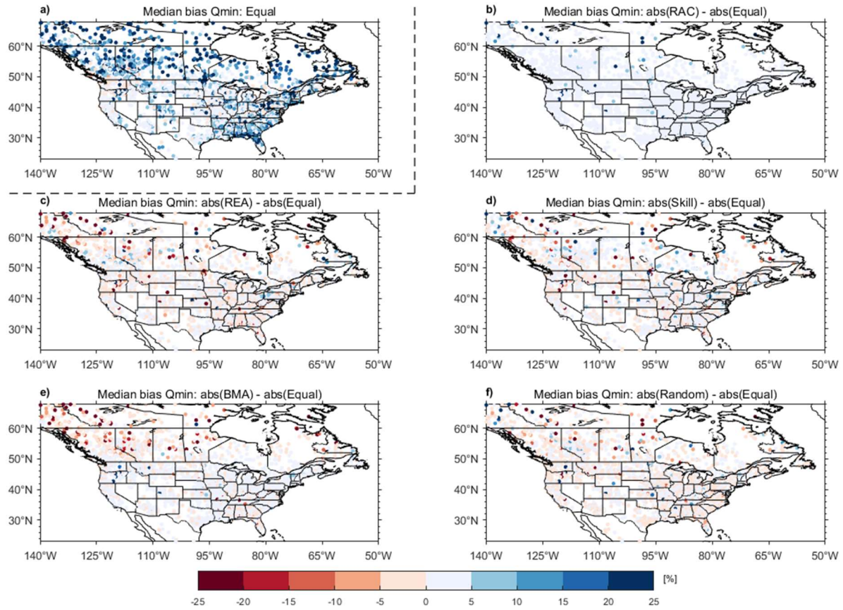
Figure S3. Similar to figure 6 but for minimum streamflow ( Q_{min} ).
