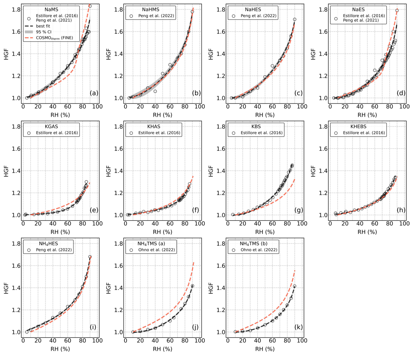
Figure S3. Hygroscopic growth factors (HGFs) of all OS particles as a function of RH at 295 K. The computed HGFs were estimated on the basis of the COSMO therm -derived water activities that used the FINE parameterization and are present in red dashed lines. The HGF measurement data from the literature are present in open circles in grey, with the best fit (black dashed lines) and 95% confidence intervals (95% CIs; shaded areas in grey).
