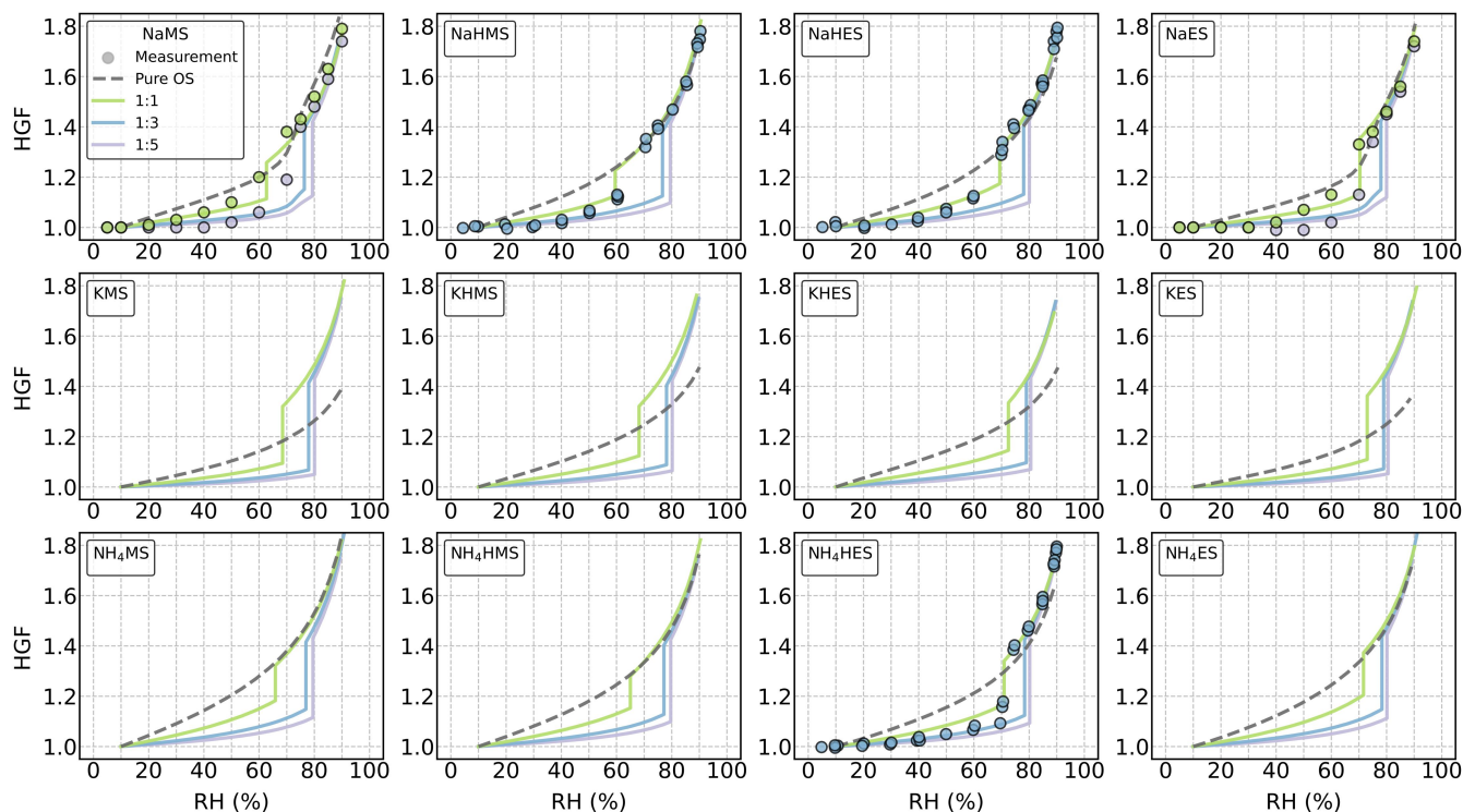
Figure S5. Hygroscopic growth factors (HGFs) for OS-AS mixture particles. The filled circles indicate the measurement data from the literature, with colors indicating different OS:AS mass ratios. The HGF data calculated from the COSMO therm -derived water activities are in dashed lines for pure organosulfur (OS) compounds and in solid lines for the OS-AS mixtures, with colors indicating different OS:AS mass ratios.
