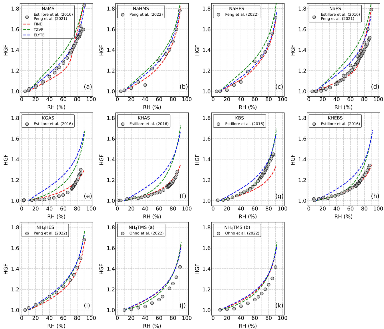
Figure S4. Hygroscopic growth factors (HGFs) of all OS particles as a function of RH at 295 K. The HGF derived from the COSMOtherm-derived water activities are in dashed lines for FINE (red), TZVP (green), and ELYTE (blue) parameterizations. The HGF measurement data from the literature are present in filled circles in grey.
